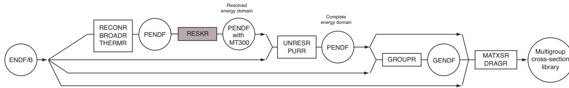
Figure 1. Flow chart of modules in NJOY
