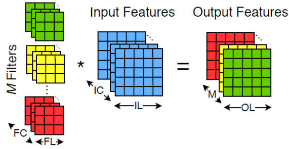
Figure 2.1 Computation of a convolutional layer.
