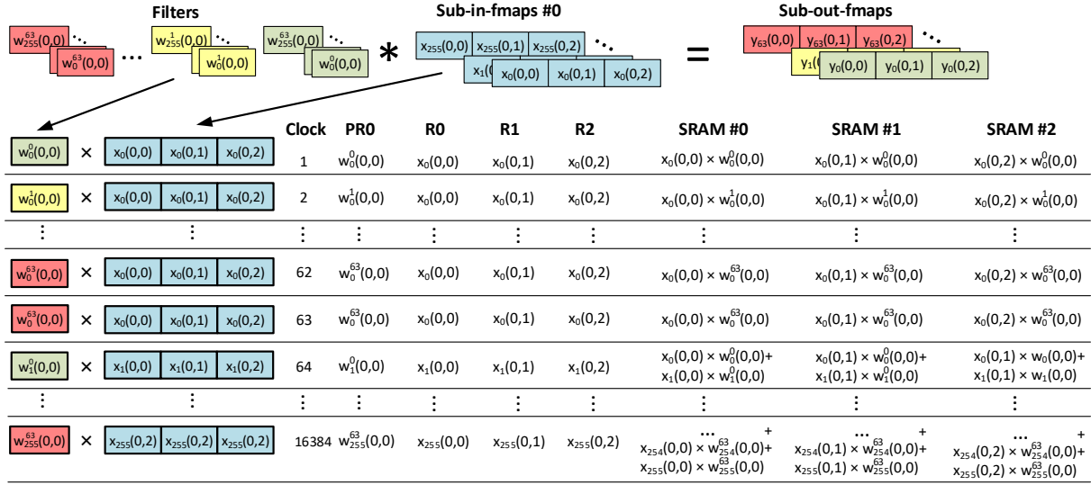
Figure 5.8 Proposed dataflow for 1x1 convolution [76].
