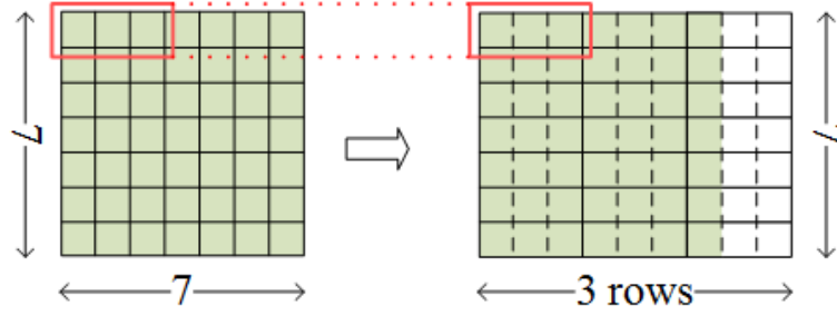
Figure 5.9 Splitting each plane of a 7×7 filter into 21 pieces [76]
