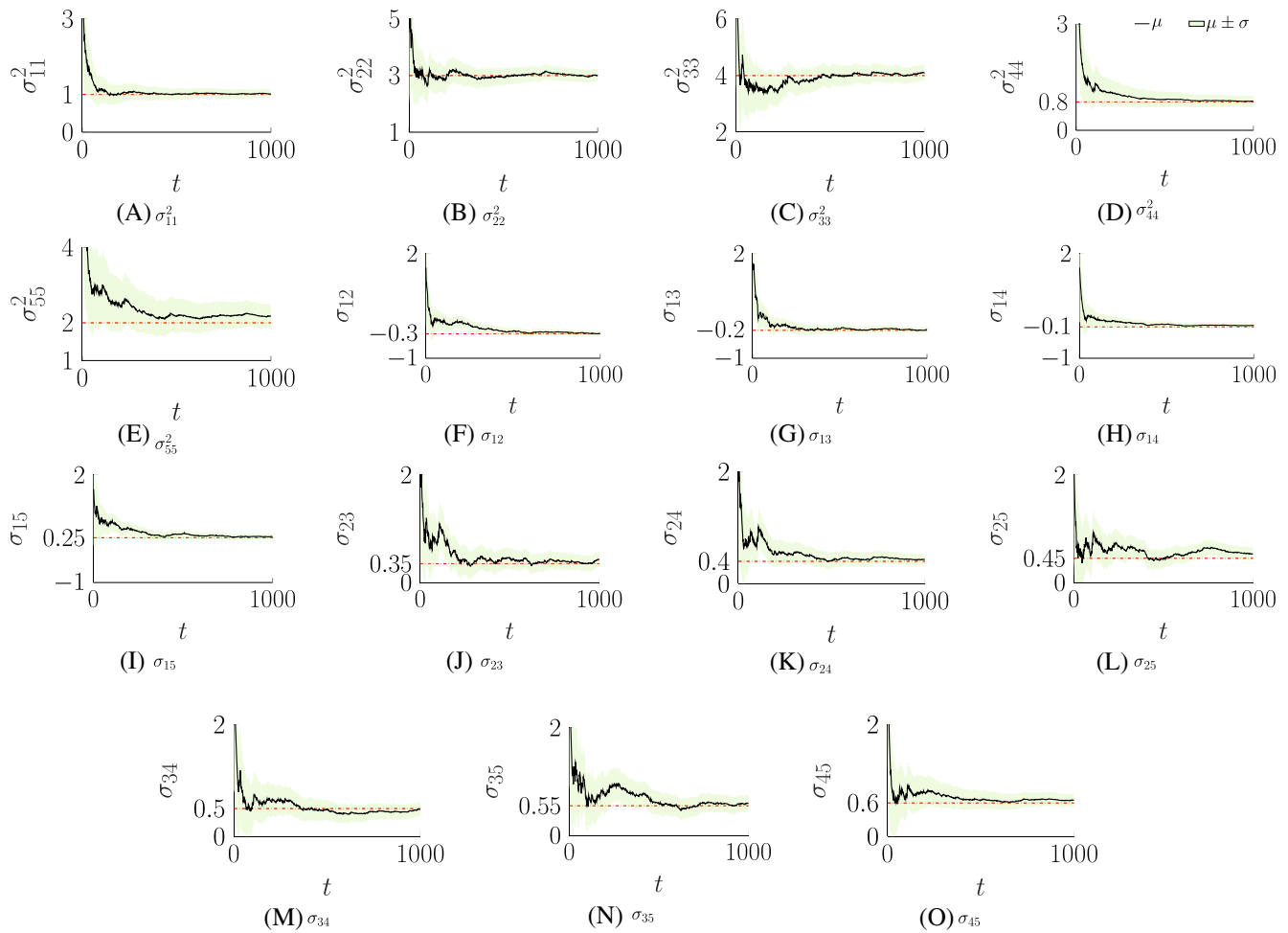
FIGURE E1 Online estimation of the error variance term and the covariance terms from the full \mathbf{Q} matrix compared to their true values marked by the dashed red line. The estimated values are shown by the black solid line and their \pm 1\sigma uncertainty bound is shown using the green shaded region.
