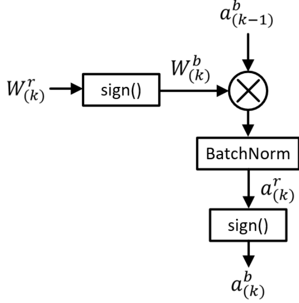
Figure 3.1 Forward propagation of BNNs. k represents the layer number, r , a full precision or real value and b , a binarized value.
