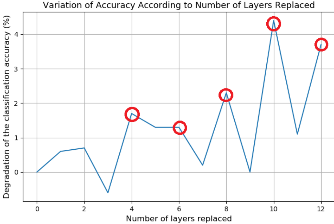
Figure 5.7 Degradation of the classification accuracy compared to the previous layer according to the number of layers replaced. A higher value means a larger degradation. The red circles represent the layers for which the inputs had more input channels (32 instead of 16).
