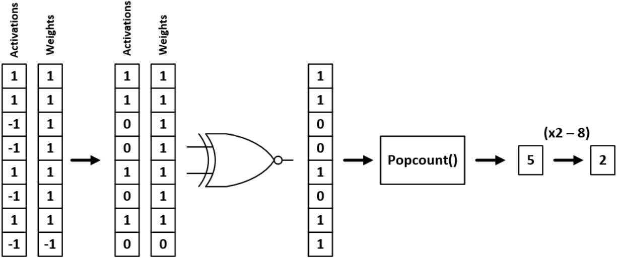
Figure 3.3 Example of a binary dot-product with xnor and popcount operations. The result of the popcount operation is multiplied by 2 and subtracted by the number of bits in the input array. This is required since -1s are represented with 0s.
