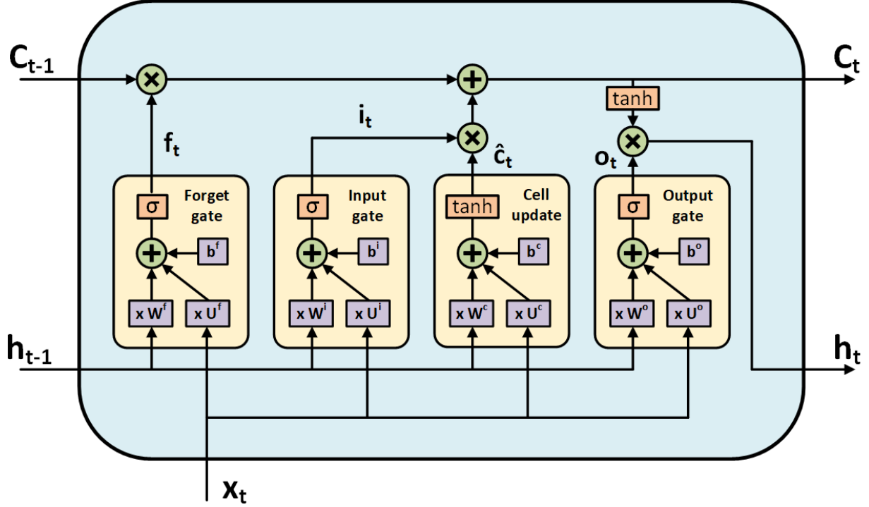
Figure 2.9 Structure of an LSTM cell. Each cell includes a forget, input and output gate. The C values represents the cell state which remembers the information across states.
