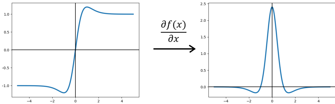
Figure 3.5 The Signswish function and its gradient.
