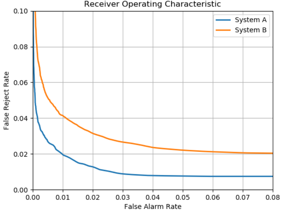
Figure 2.5 Example of ROC curves illustrating False Rejects vs False Alarms.
