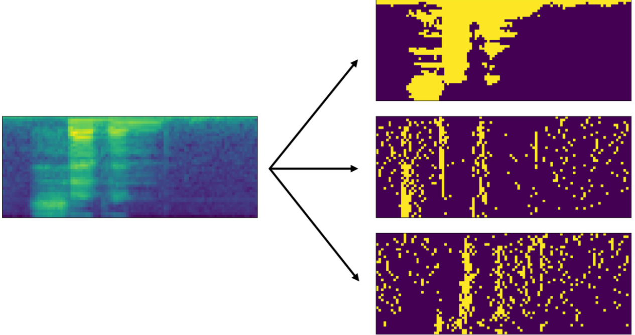
Figure 5.1 Converting the log-Mel spectrogram (middle-left) to a 3-channel representation with static power in the first channel (top-right), increases in power in the second channel (middle-right) and decreases in power in the third channel (bottom-right).
