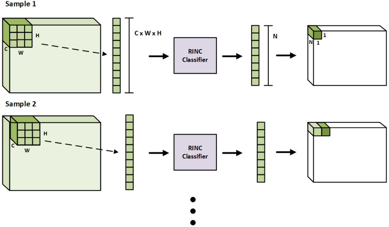
Figure 5.4 Replacing the convolution kernels of a CNN with a RINC classifier. For each kernel position, the data is flattened and injected into the RINC classifier. A single image can generate many training samples since every kernel position represents new data. C represents the number of input channels, W the width of the kernel, H the height of the kernel and N , the amount of filters used.
