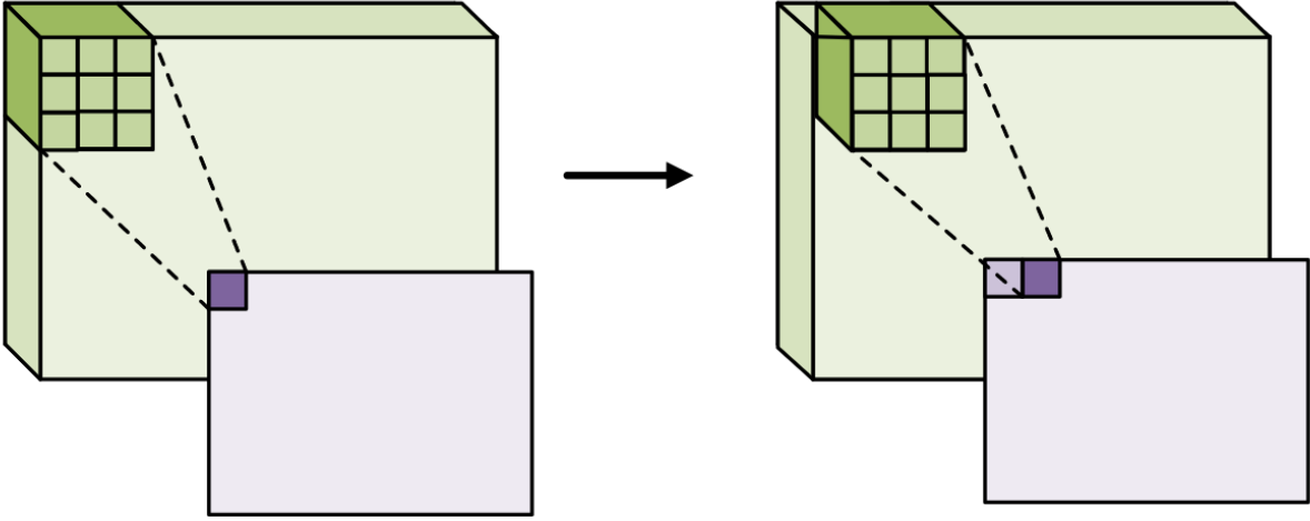
Figure 2.8 Example of the convolution operation performed in a CNN.
