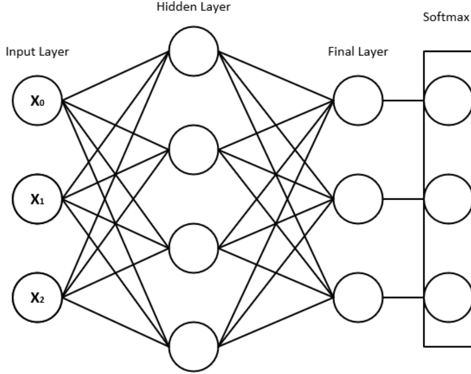
Figure 2.7 Example of a Multi-Layer Perceptron with a single hidden layer.
