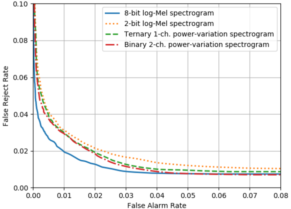
Figure 4.5 ROC curves for various input representations.
