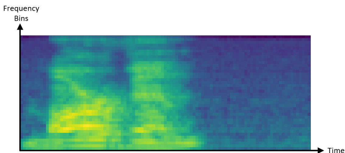
Figure 2.3 Example of the log-Mel Spectrogram with 40 filters. The vertical axis represents the various frequency bins (after applying filters). The horizontal axis represents time.
