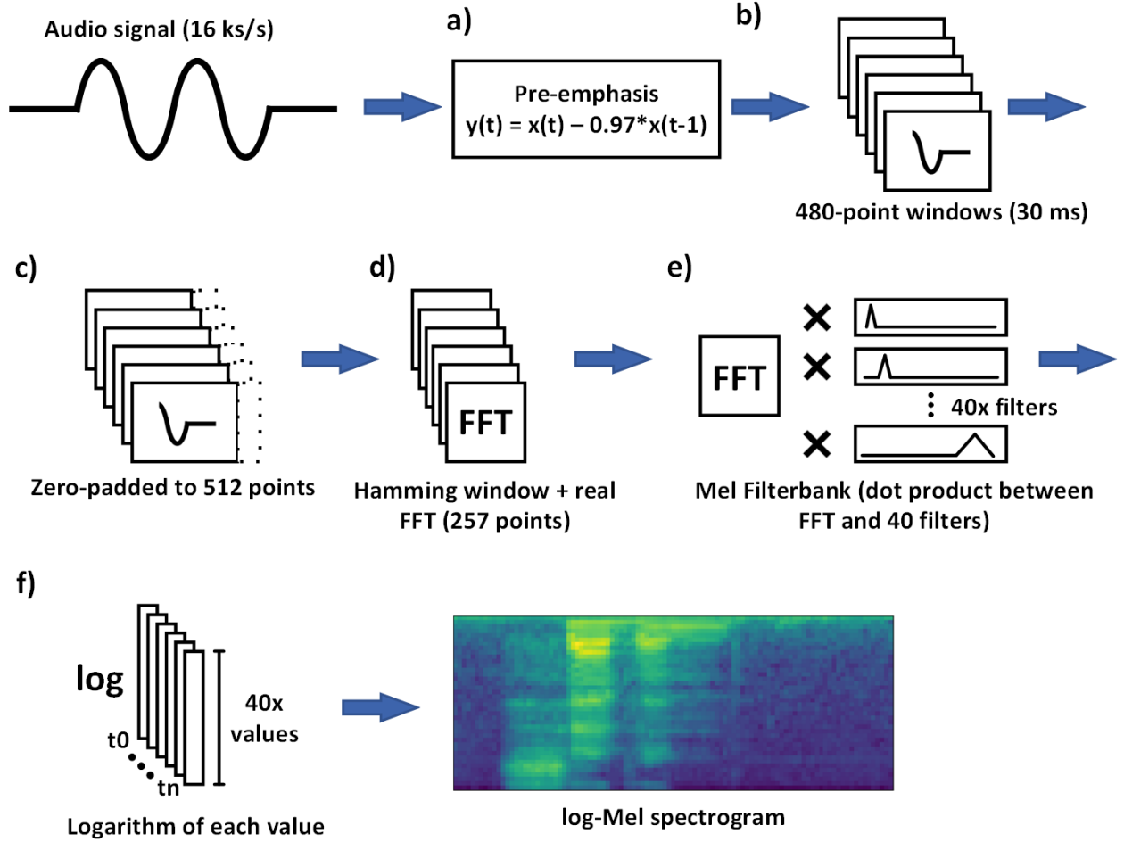
Figure 4.1 Steps to compute the log-Mel spectrogram of a speech signal or sound wave.
