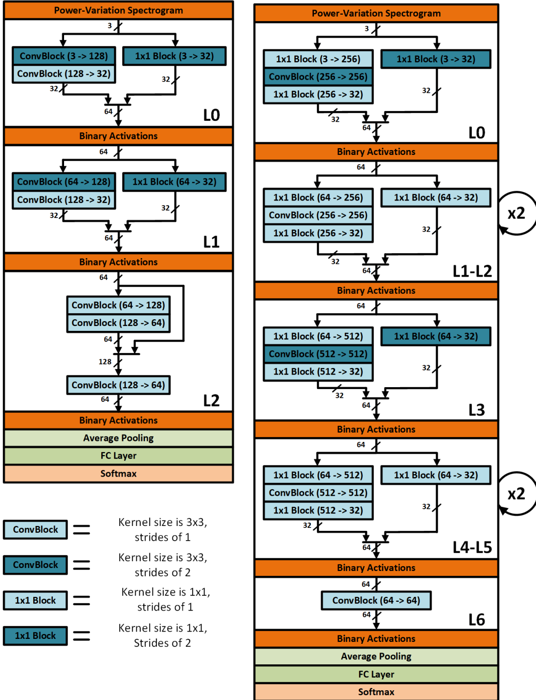
Figure 5.9 Networks that merge convolution blocks using RINC-2 classifiers. Network-A (left) contains 3 layers and was the first attempt at merging continuous layers. Network-B (right) contains 7 layers and uses 1 \times 1 convolutions to expand the size of the intermediate feature maps. Blocks in light blue use strides of 1 and blocks in dark blue use strides of 2. All weights and activations used in intermediate calculations are in floating-point format. A sign function is applied to the outputs of the last ConvBlocks of each layer to obtain binary values.
