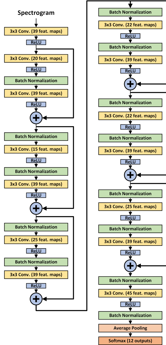
Figure 4.2 Architecture of EdgeSpeechNet-A. This ResNet is used to test the different input representations proposed in this paper.
