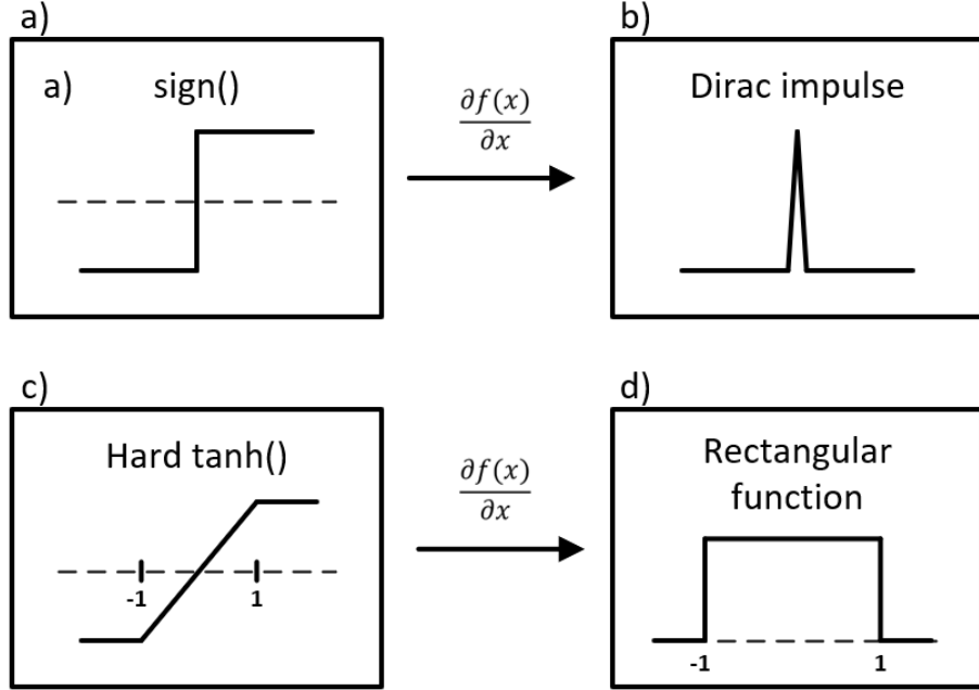
Figure 3.2 a) Sign function used during forward propagation. b) Gradient of sign function (Dirac impulse). c) Hard tanh function used during backpropagation. d) Gradient of hard tanh (Rectangular function)
