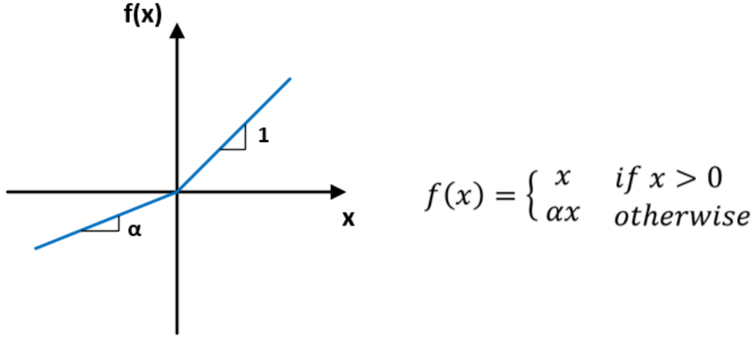
Figure 3.4 The PReLU activation function.
