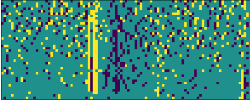
Figure 4.4 Ternary 1-channel power-variation spectrogram for the word “up”. A yellow pixel is equal to 1, a purple pixel to -1 and a green pixel to 0.
