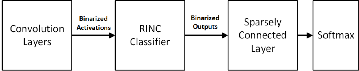
Figure 5.3 Original use-case of the RINC classifier. The classifier replaced the fully-connected layers at the end of a VGG/LeNet network. To accomodate binary decision trees, the outputs of the convolution layers were flattened and binarized. The sparsely connected layer was used to generate higher bit precision logits.
