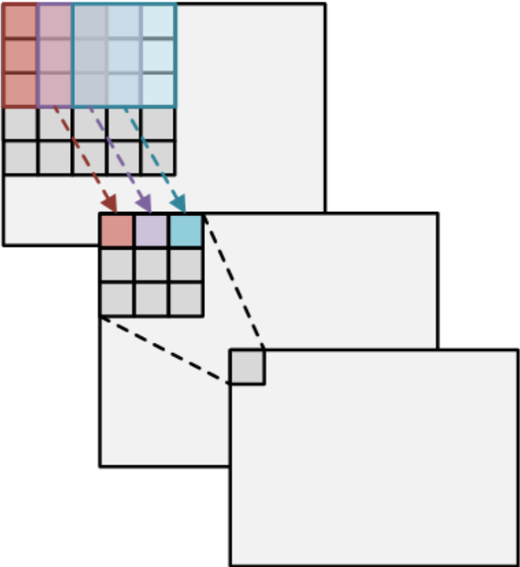
Figure 5.8 Receptive field after applying 2 convolution layers with 3 \times 3 kernels using strides of 1. If two layers were to be combined, a 5 \times 5 kernel would be required to capture all the same features.
