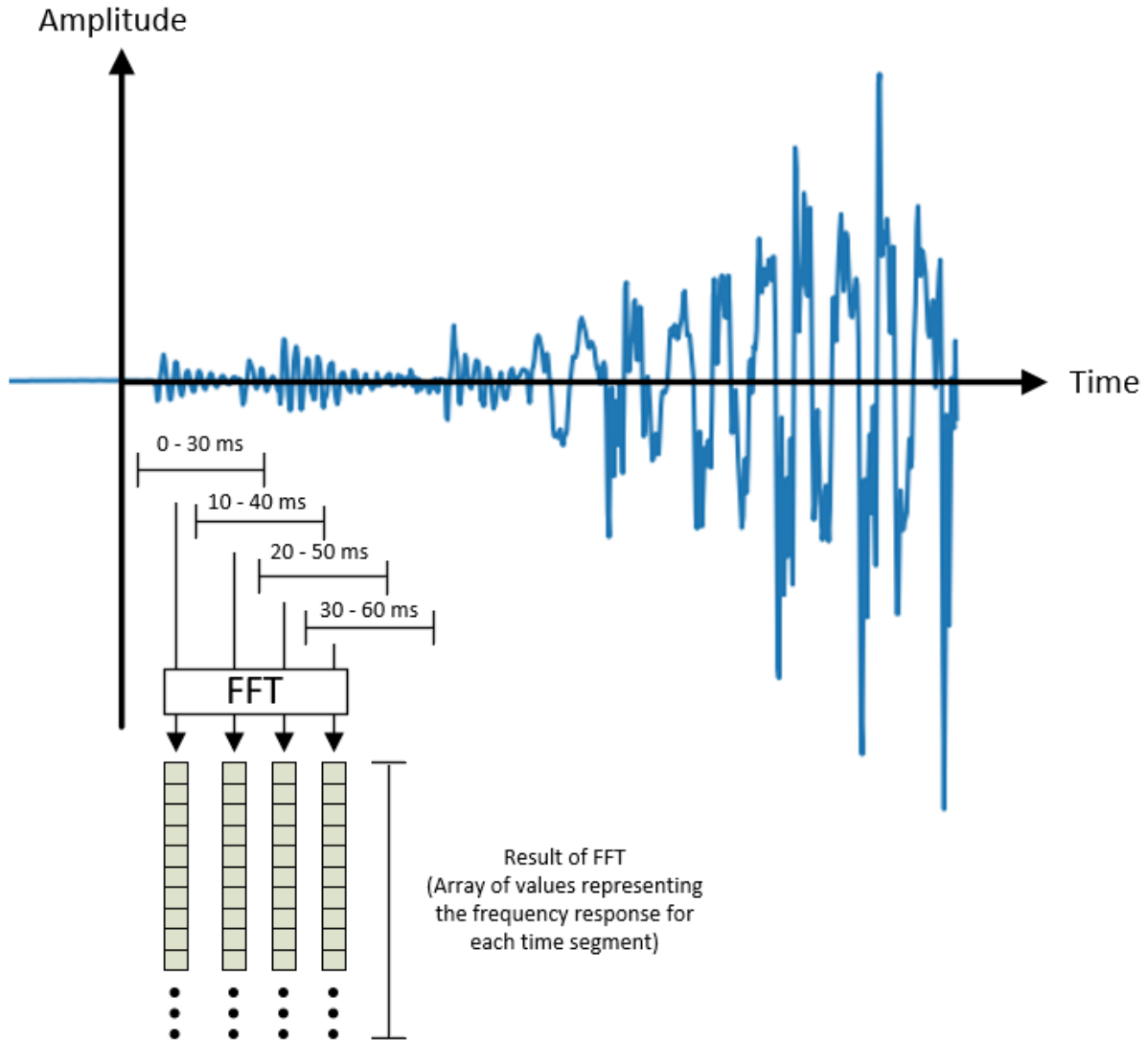
Figure 2.1 Extracting frames from an audio signal sampled at 16 kHz.
