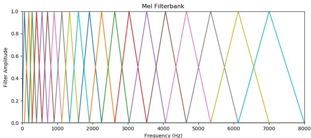
Figure 2.2 Filters spread out on the Mel Scale.
