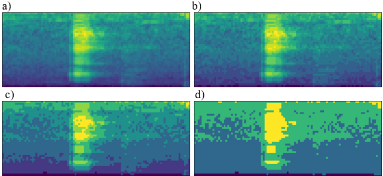
Figure 4.3 Quantized representations of the log-Mel spectrogram for the word “up”. a) 8-bit rep. b) 4-bit rep. c) 3-bit rep. d) 2-bit rep.
