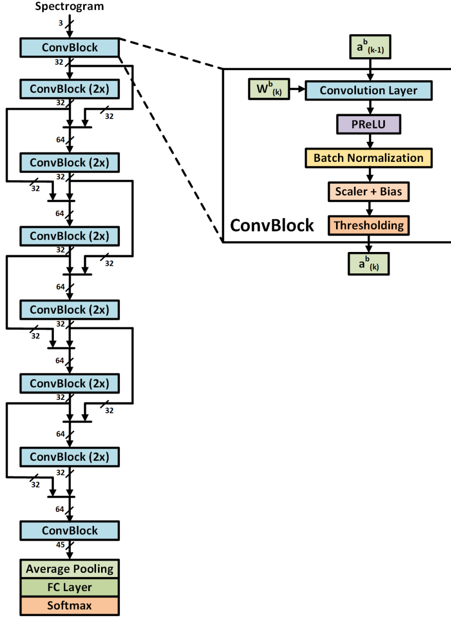
Figure 5.2 Proposed Binary Neural Network for keyword spotting (left). The ConvBlock used (right). The first ConvBlock does not use batch normalization. The scaler is a learnable parameter which multiplies the activations and the bias is a learnable parameter which is added to the activations. Thresholding is performed using the sign function. k represents the layer number and the b indice represents a binarized value.
