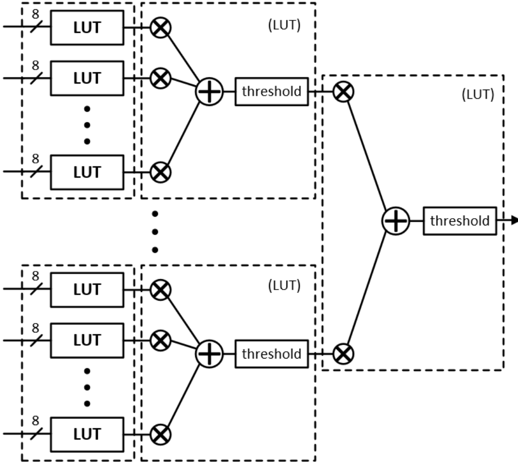
Figure 3.6 PoET-BiN architecture using 8-input LUTs.
