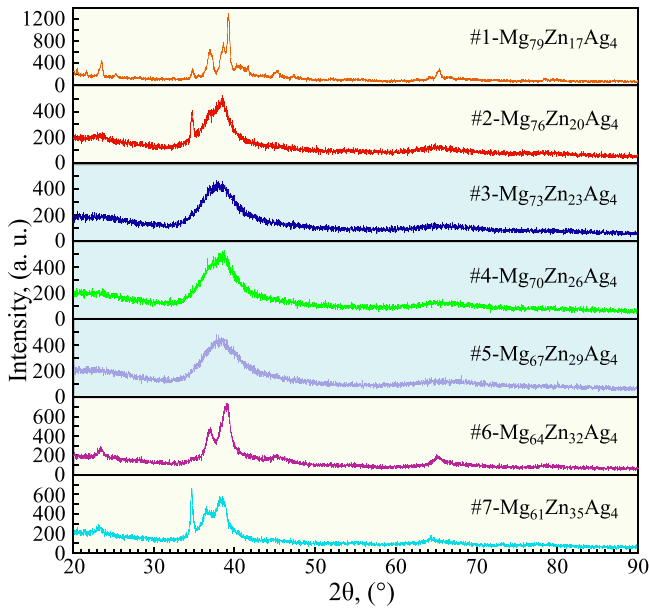
Fig. 2. XRD patterns of #1- \text{Mg}_{79}\text{Zn}_{17}\text{Ag}_4 , #2- \text{Mg}_{76}\text{Zn}_{20}\text{Ag}_4 , #3- \text{Mg}_{73}\text{Zn}_{23}\text{Ag}_4 , #4- \text{Mg}_{70}\text{Zn}_{26}\text{Ag}_4 , #5- \text{Mg}_{67}\text{Zn}_{29}\text{Ag}_4 , #6- \text{Mg}_{64}\text{Zn}_{32}\text{Ag}_4 and #7- \text{Mg}_{61}\text{Zn}_{35}\text{Ag}_4 samples obtained by powder XRD diffraction.
