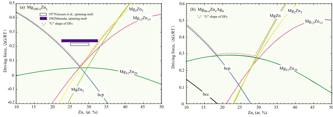
Fig. 1. The calculated DFs of individual crystalline phases of (a) Mg-Zn and (b) \text{Mg}_{96-x}\text{Zn}_x\text{Ag}_4 alloys using CALPHAD technique.
