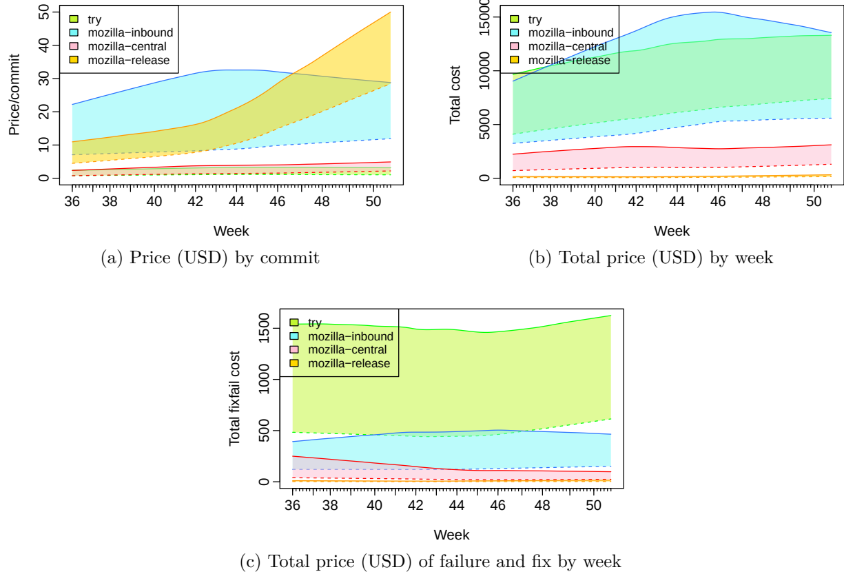
Figure 3.4 Loess regression of the median values for (a) and total for (b) and (c) with lower-bound (Azure approach) and upper-bound (AWS On-Demand) on each branch over weeks of releases 36 to 50.
