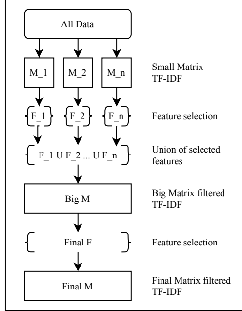
Figure 4.1 Iterative vectorization algorithm
