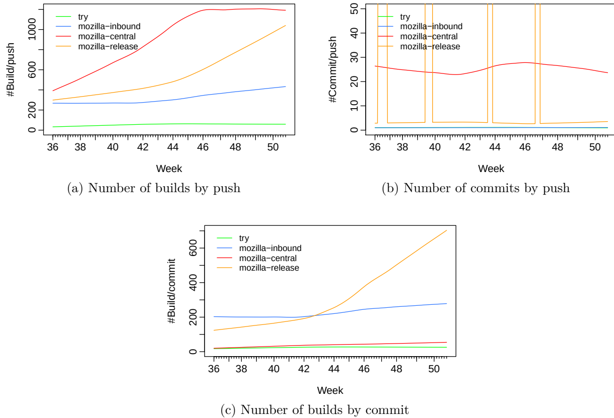
Figure 3.3 Loess regression of the median values on each branch over weeks of releases 36 to 50.
