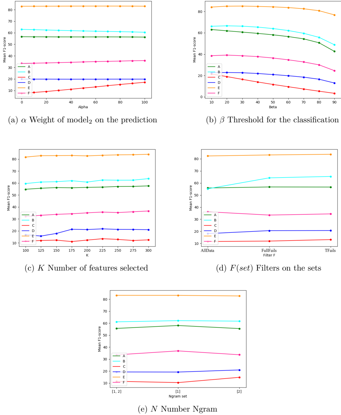
Figure 4.5 Comparison of the mean F1-score performance by hyper-parameters.
