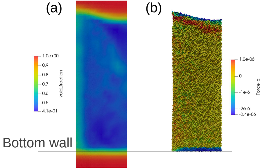
Figure 8: Snapshot of the U/U_0 = 0.1430 alginate particles simulation at 35 seconds (last time-step), showing (a) the void fraction profile and (b) the total force acting over particles in Newtons. Results are clipped in the axial direction to show the middle of the equipment. It can clearly be seen that the first few layers of particles are supported by the bottom wall.
