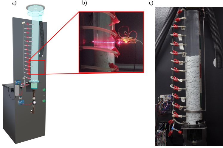
Figure 1: Schematic representation of a) the equipment and b) the laser apparatus used for bed height measurement.
