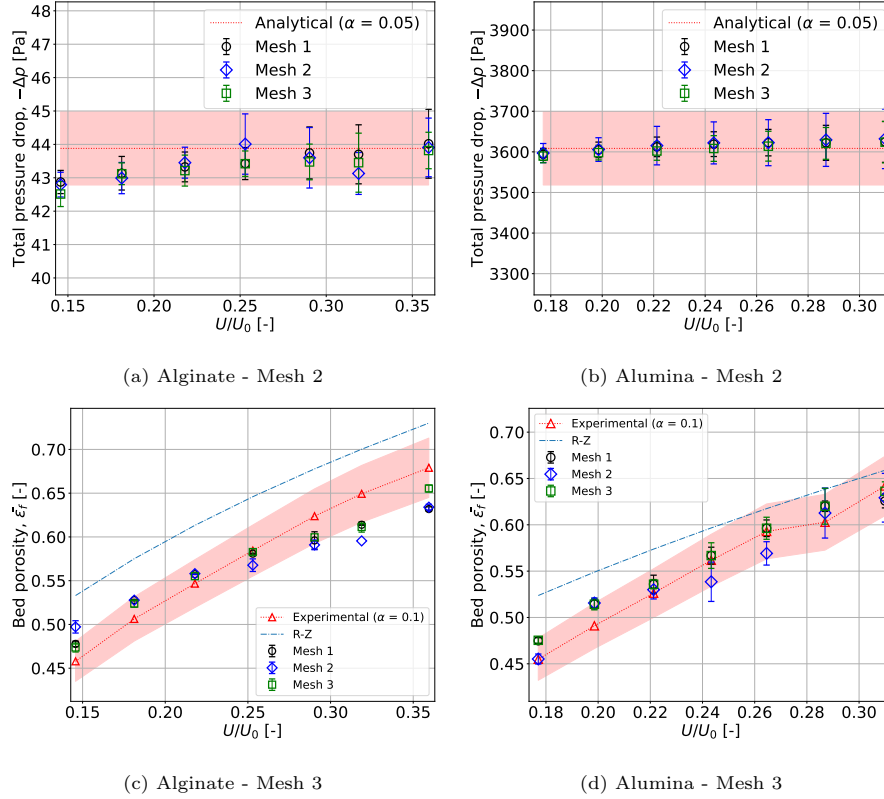
Figure 11: Bed expansion and pressure drop for the different mesh and particle combinations.
