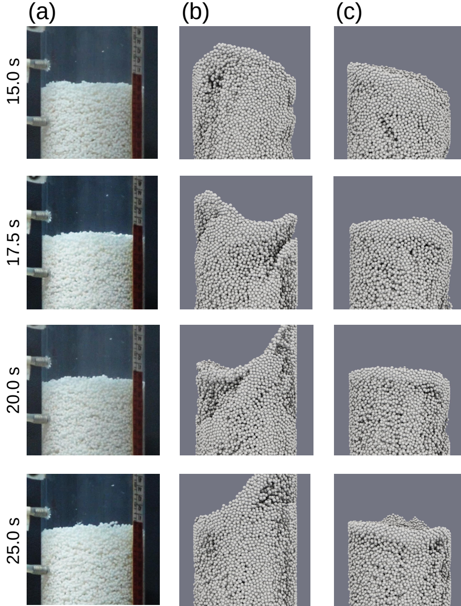
Figure 5: Images of the top of the pseudo-steady state (reached around 10 seconds of simulation)
