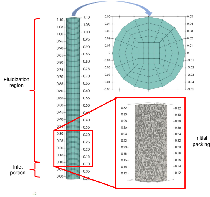
Figure 2: Schematic representation of the mesh and initial packing of particles (units in meters).
