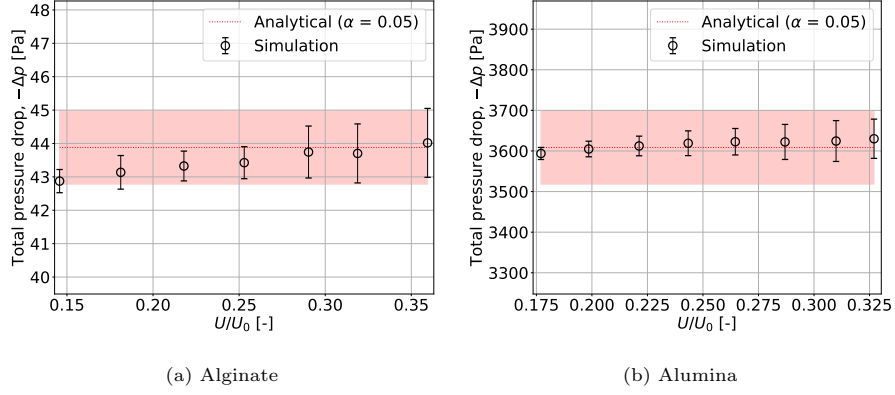
Figure 7: Average of the total pressure difference for the (a) alginate and (b) alumina particles
