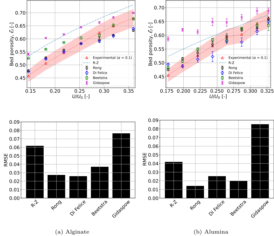
Figure 12: Bed porosity with different drag correlations for (a) alginate and (b) alumina particles.
