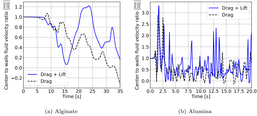
Figure 4: Center to walls velocity ratio for (a) alginate and (b) alumina particles, at U/U_0 = 0.3595 and U/U_0 = 0.3270 , respectively.
