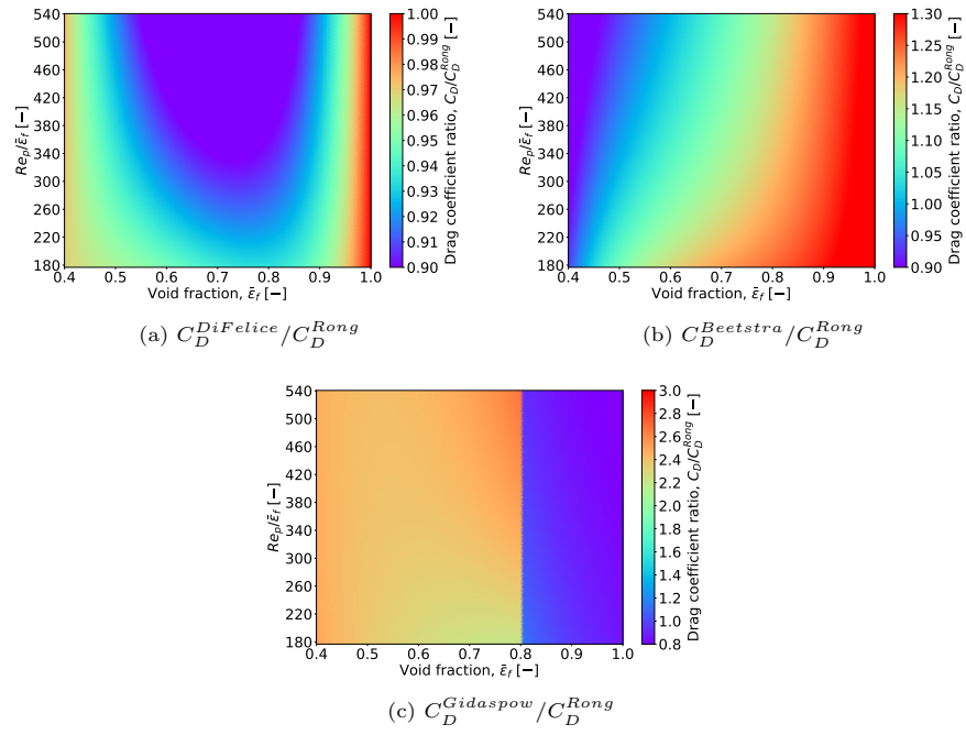
Figure 14: C_D/C_D^{Rong} comparison among correlations for the alumina particles, showing the ratios a) C_D^{DiFelice}/C_D^{Rong} , b) C_D^{Beetstra}/C_D^{Rong} , and c) C_D^{Gidaspow}/C_D^{Rong} for Di Felice, Beetstra, and Gidaspow, respectively. Color scales are different for each correlation due to their high discrepancy.
