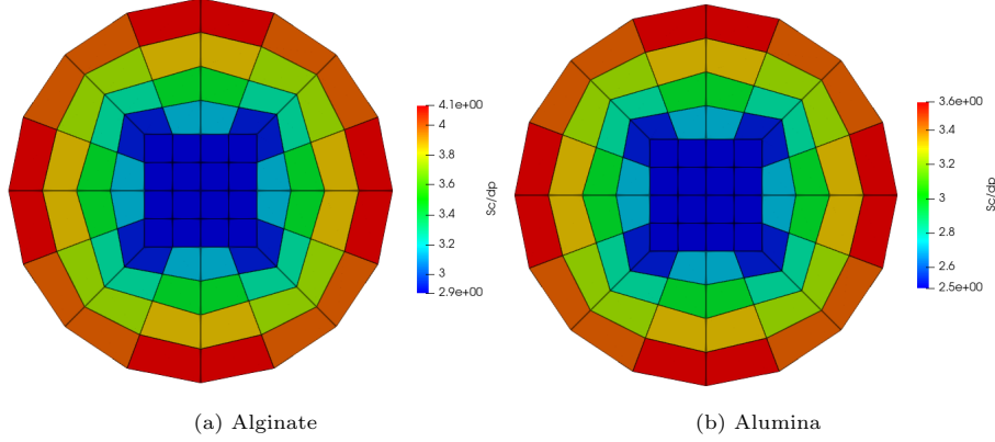
Figure 3: S_c/d_p for (a) alginate and (b) alumina particles.
