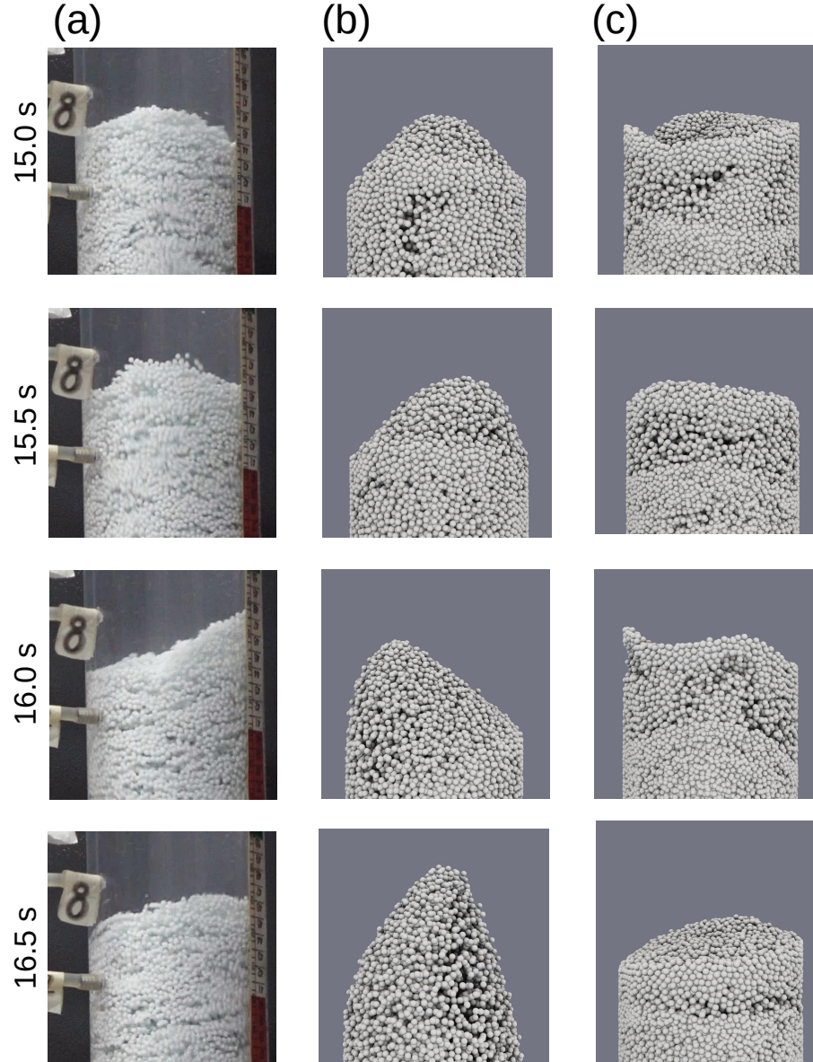
Figure 6: Images of the top of the pseudo-steady-state (reached around 4 seconds of simulation)
