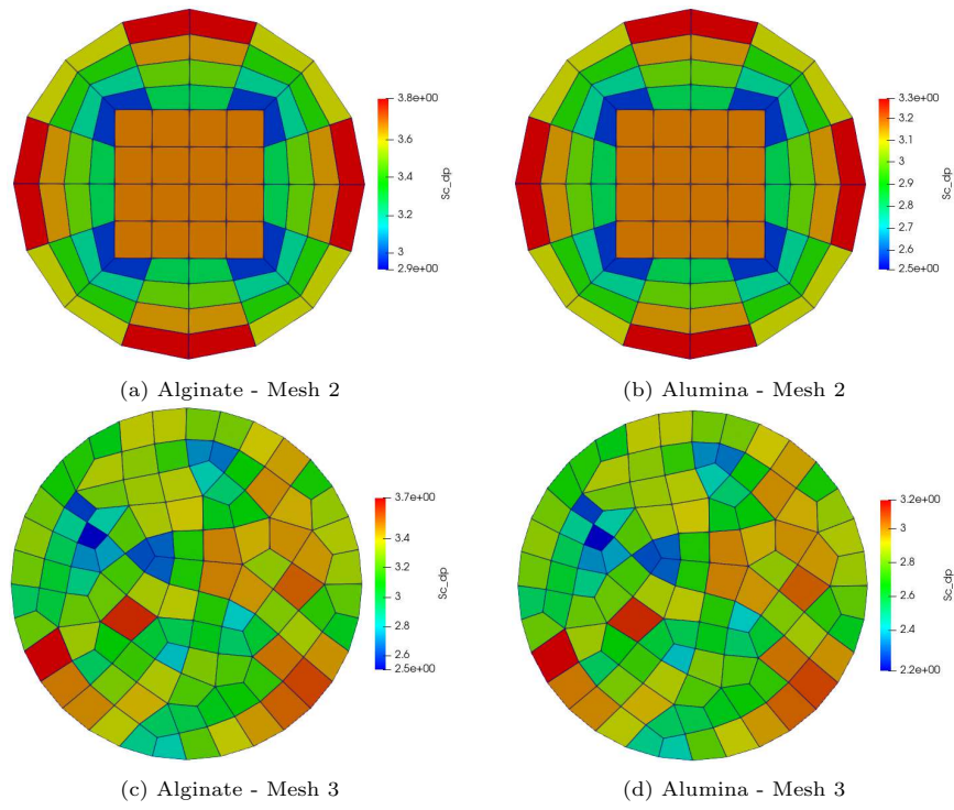
Figure 10: S_c/d_p for the different mesh and particle combinations.
