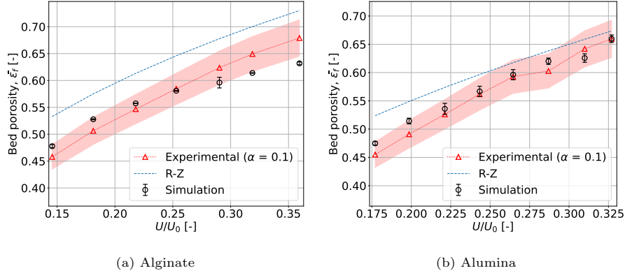
Figure 9: Bed porosity for (a) alginate and (b) alumina particles.
