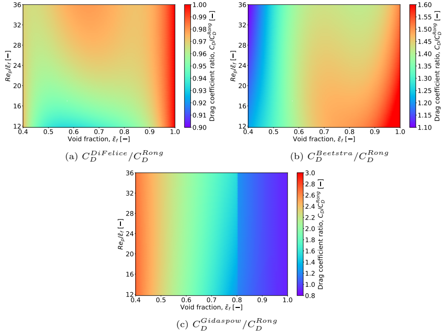
Figure 13: C_D/C_D^{Rong} comparison among correlations for the alginate particles, showing the ratios a) C_D^{DiFelice}/C_D^{Rong} , b) C_D^{Beetstra}/C_D^{Rong} , and c) C_D^{Gidaspow}/C_D^{Rong} for Di Felice, Beetstra, and Gidaspow, respectively. Color scales are different for each correlation due to their high discrepancy.
