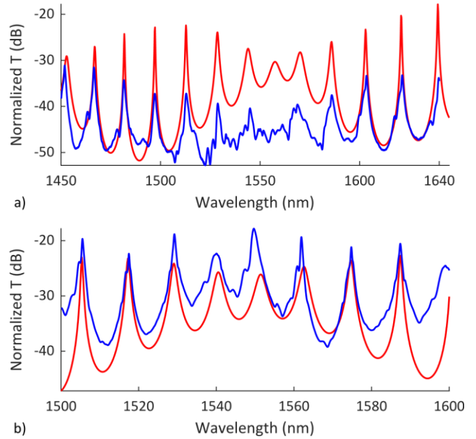
Fig. 6. Experimental (blue) and calculated (red) transmission spectrum from FPI. a) Empty cavity with width of silicon, gold and microfluidic channel being respectively 2.59\mu\text{m} , 60\text{nm} and 68.9\mu\text{m} b) Cavity filled with PDMS with width of silicon, gold and microfluidic channel being respectively 2.56\mu\text{m} , 60\text{nm} and 68.0\mu\text{m}
