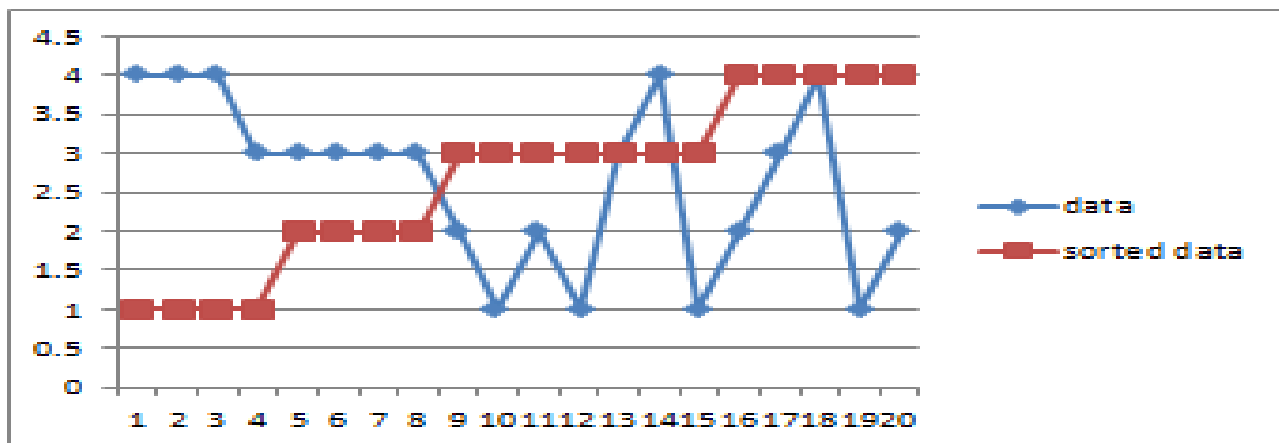
Fig. 5 Data classification.
