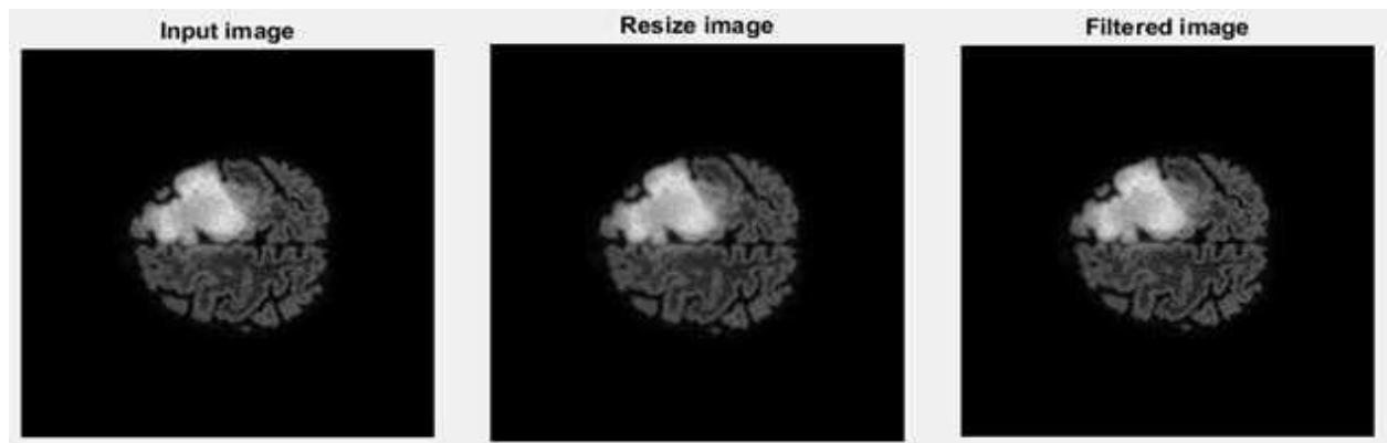
Fig. 6 Preprocessing steps:
