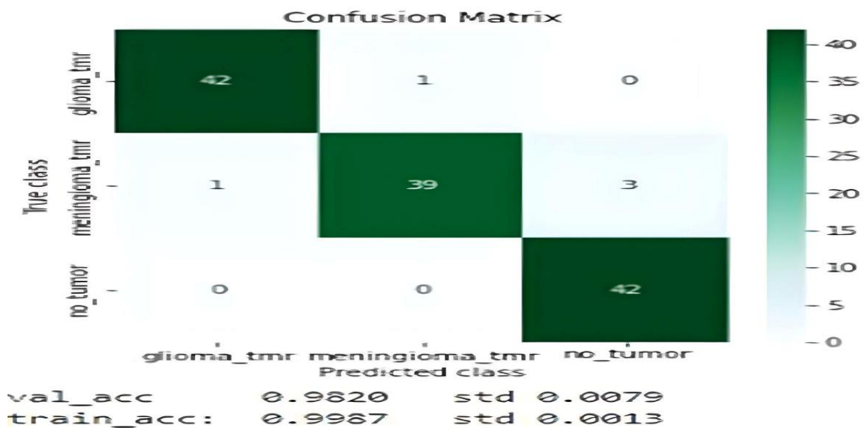
Fig. 6: confusion matrix
