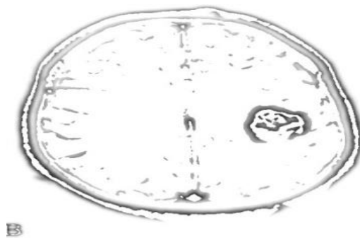
Fig.10: Inverted image
