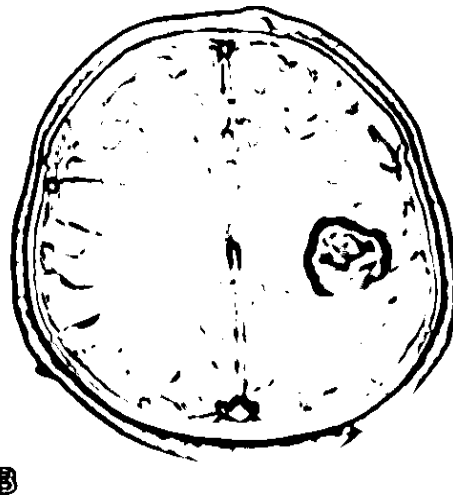
Fig. 11: Binarized image
