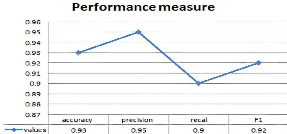
Fig.13: Performance measure
