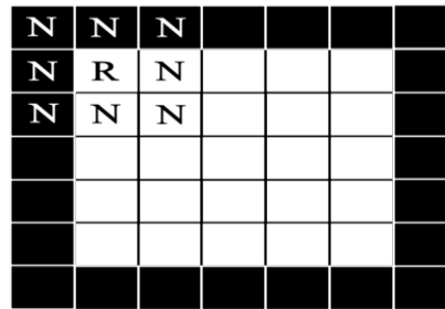
Fig.6: Illustration of zero-padding on 8-point neighbors
