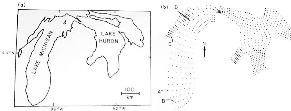
Figure 4: (a) Basins of lakes Michigan and Huron joined at the Straits of Mackinac. (b) Curvilinear mesh for the basins of lakes Michigan and Huron. Points A, B, C and D are special locations where observations were available for comparison with theory. (Birchfield and Murty, 1974)
