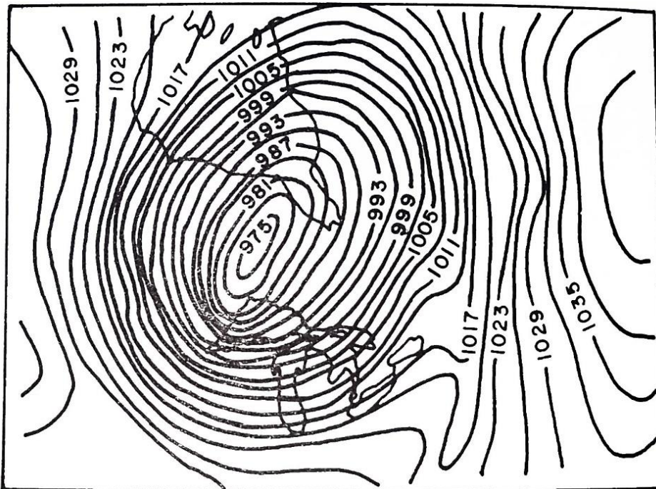
Figure 7: Simplified surface weather chart at 07:30 (GMT) on November 12, 1940. Numbers represent sea level pressures (millibars). (Murty and Polavarapu, 1975).
