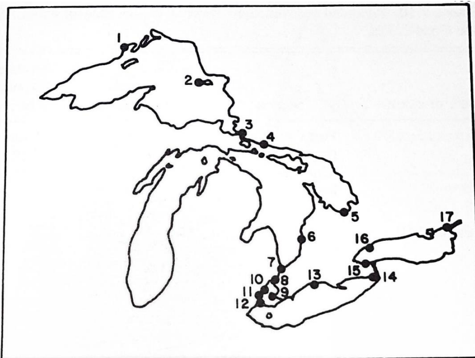
Figure 8: Water level stations used in the storm surge study for the Great Lakes. 1, Port Arthur; 2, Michipicoten; 3, Sault Ste. Marie; 4, Thessalon; 5, Collingwood; 6, Goderich; 7, Point Edward; 8, Port Lambton; 9, Tecumseh; 10, Isle aux Pêches; 11, Fighting Island; 12, La Salle; 13, Port Stanley; 14, Port Colborne; 15, Port Dalhousie; 16, Toronto; 17, Kingston. (Murty and Polavarapu, 1975).
