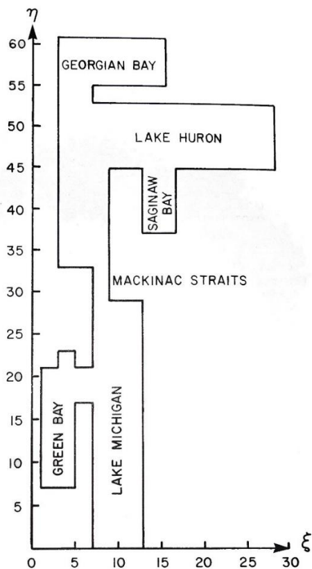
Figure 5: Basins of lakes Michigan and Huron as arranged on the (\xi, \eta) plane. (Birchfield and Murty, 1974)
