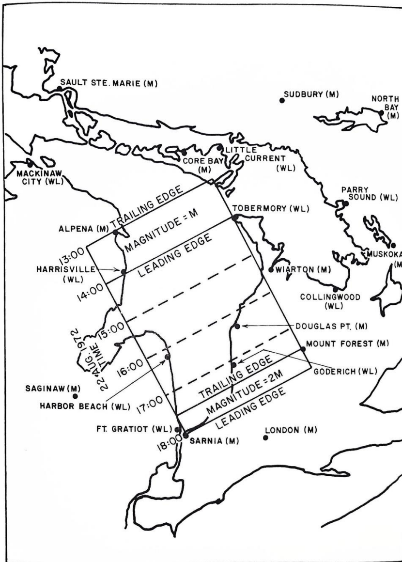
583 Figure 12: Water level (WL) and meteorological (M) stations on and around Lake Huron. The position of 584 the squall line as a function of time is also shown. (Murty and Freeman, 1973) 585
