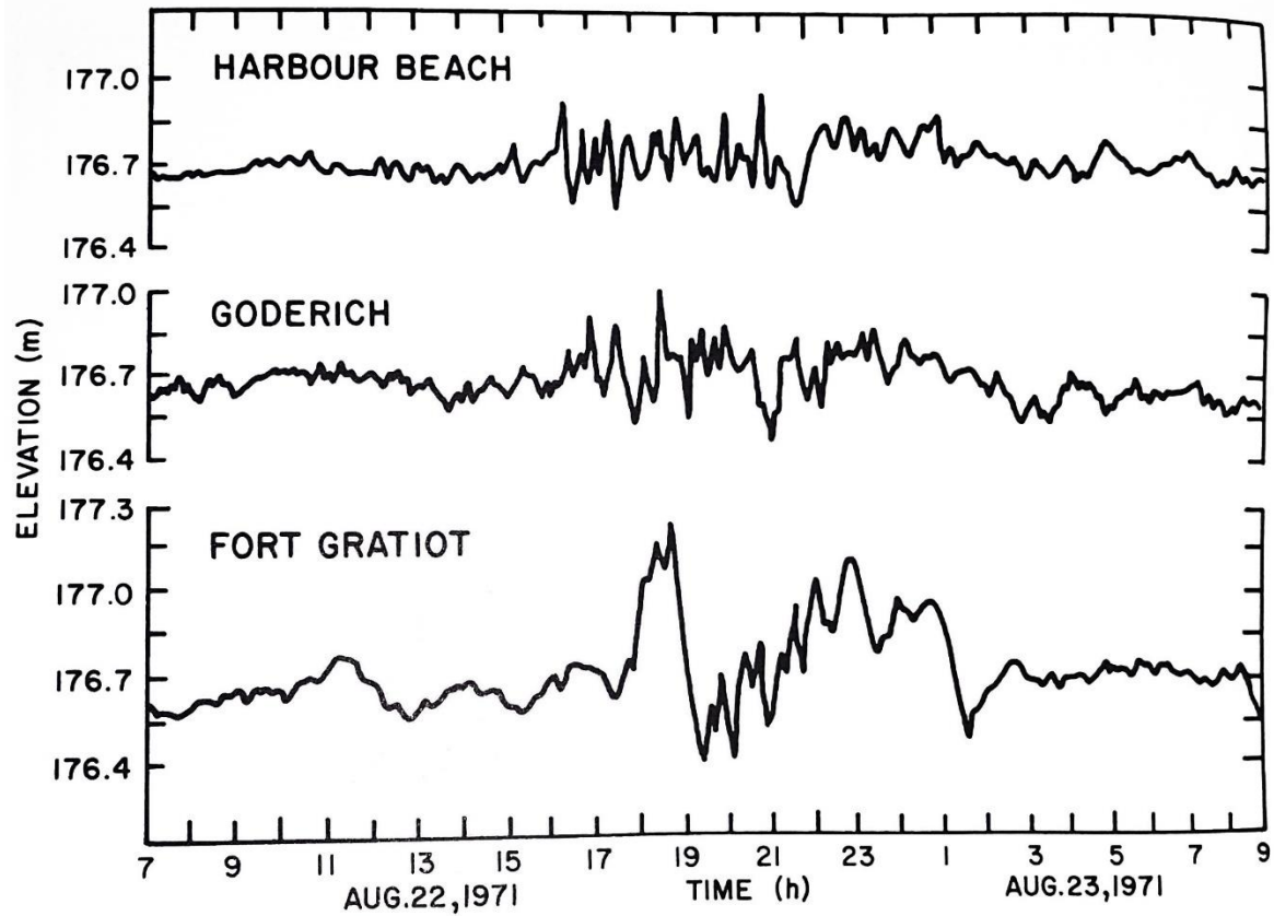
Figure 11: Five minute digitized water level values as obtained from continuous recorders at three stations on Lake Huron. (Freeman and Murty, 1972)
