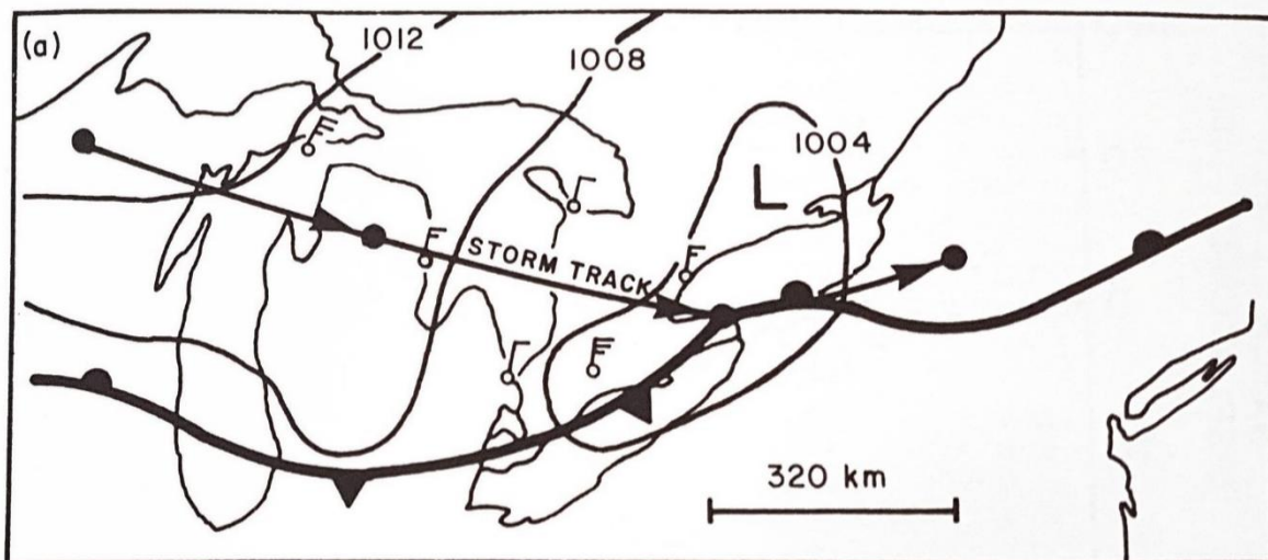
Figure 9: Simplified surface weather chart at 19:00 GMT on August 22, 1971, for the Great Lakes area. Black circles on the storm track show the positions of the center of the low at 6-h intervals. (Freeman and Murty, 1972)
