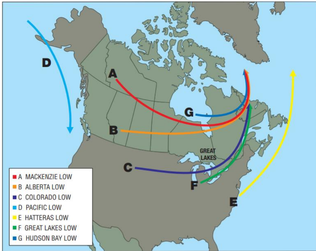
Figure 3: Summer storm tracks over the Great Lakes (NAV Canada, 2017)
