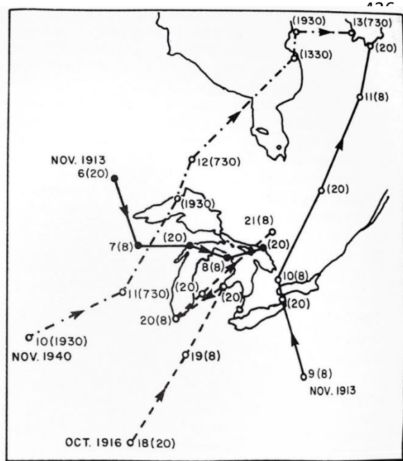
Figure 6: Tracks of three storms in the Great Lakes and surroundings. Numbers denote the dates (numbers in parentheses denote the time (GMT) in hours) (Murty and Polavarapu, 1975).
