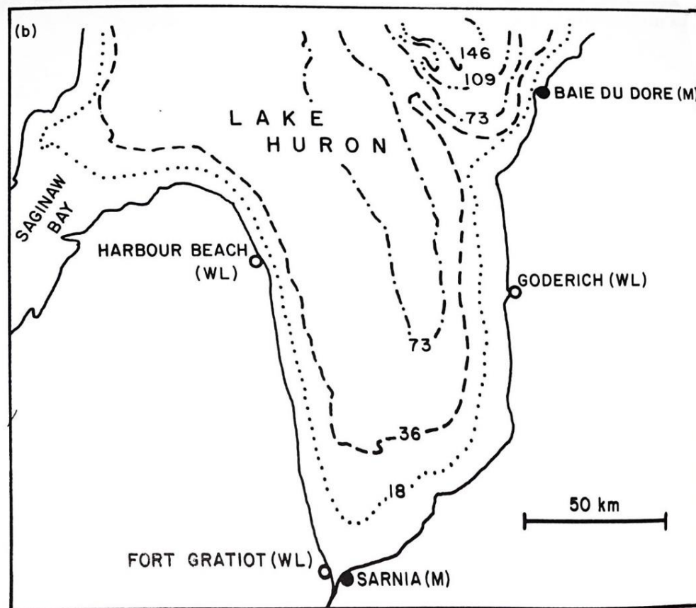
Figure 10: Locations of the various stations (M, meteorological; WL, water level) used in the study. Depth contours (meters) are also shown. (Freeman and Murty, 1972)
