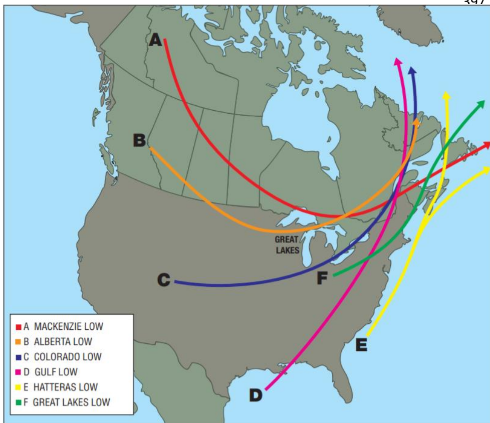
Figure 2: Cyclone tracks during winter in North America (NAV Canada, 2017)
