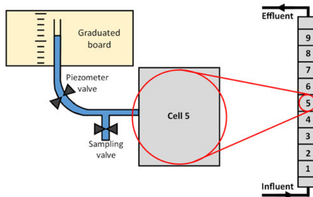
Figure 1. Schematic of column 1, with cell numbers labelled on the column. Details of valves and piezometer are shown for cell 5.
