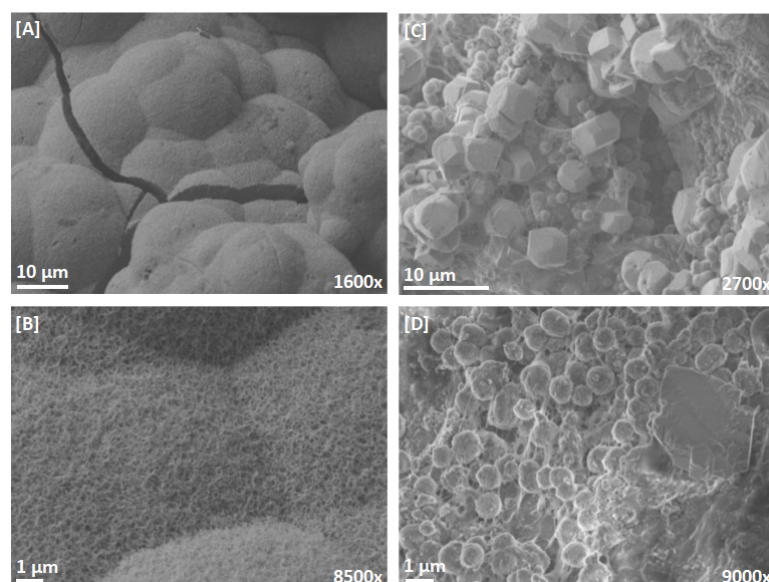
Figure 5. Crystallization in steel slag filters fed with inorganic (panels (A) and (B)) and organic (panels (C) and (D)) soluble influents. Panels (A) and (B): Column 1 cell 2. Panel C: Column 2 cell 9. Panel (D): Column 2 cell 6.
