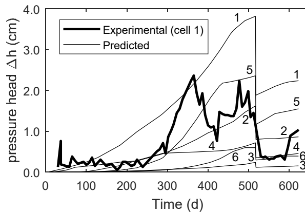
Figure 7. Pressure head build-up in cells 1 to 6 of column 1. The cell number is indicated next to each predicted line. The sudden reduction of pressure head at t = 517 d is caused by the reduction of influent flowrate from 6.9 \pm 1.3 mL/min to 3.4 \pm 0.5 mL/min.
