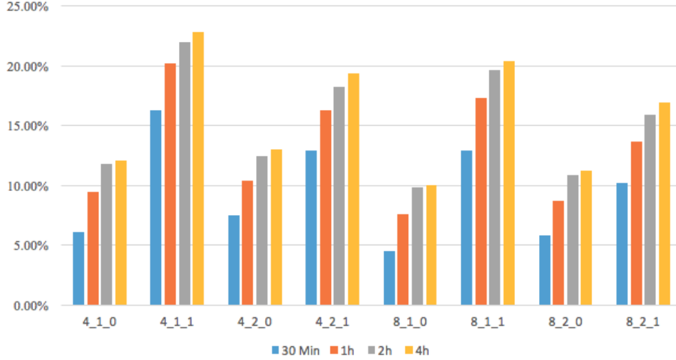
Figure 6.5 Gap to Greedy according to TW size (Week)
