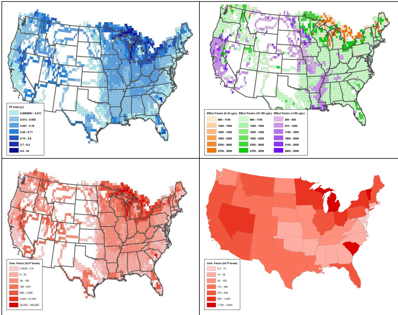
Figure S5. (a) Fate factors [yr], (b) Effect factor [PDF·m²·kg -1 ], (c) native and (d) state average characterization factors [PDF·yr·m²·kg -1 ] for phosphorous emissions in the United States.
