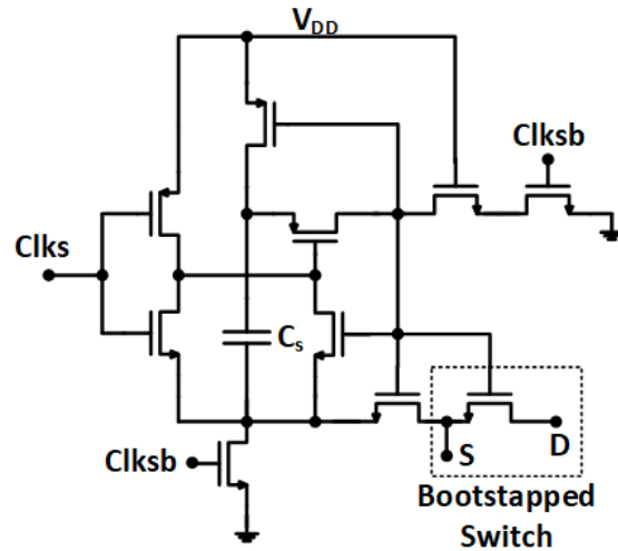
Figure 5.9 Bootstrapped switch.
