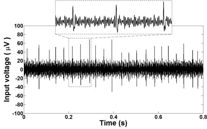
Figure 4.18 Recorded extracellular APs extracted from the brainstem of a mouse with the fabricated neural amplifier.
