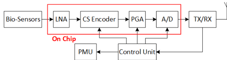
Figure 1.2 Simplified block diagram of a neural recording implant with CS encoder for one channel.
