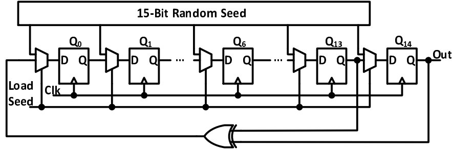
Figure 5.1 A 15-bit maximal-length Fibonacci LFSR.
