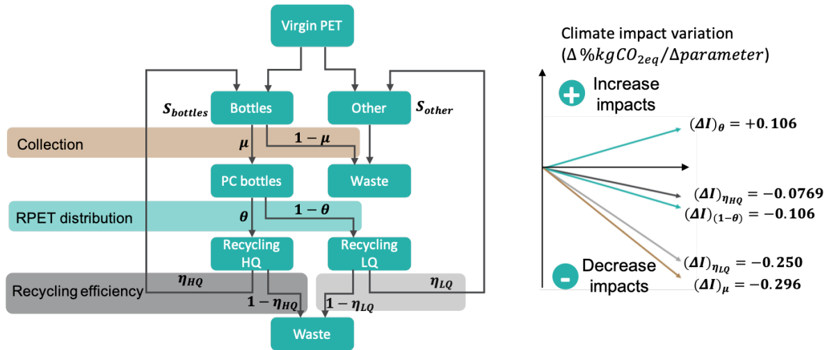
Figure 5.5: Left: simplified representation of the actual USA PET flows with tested key circularity parameters. Right: slopes representing the influence of key parameters to the total impacts on Climate Change of the USA PET market, such that e.g. (\Delta I)_{\mu} = (I_{\mu_1} - I_{\mu_0}) / (\mu_1 - \mu_0) . The lower it is, the less overall impacts.
