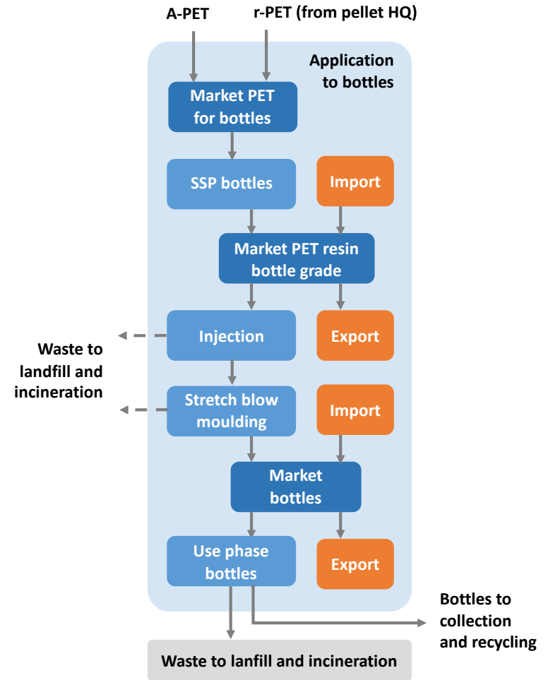
Figure B.2: Processes zoom-in on bottle application.
