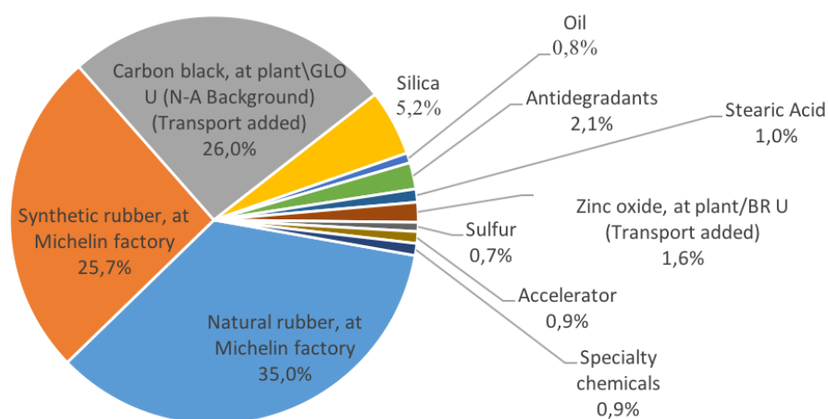
Figure A.4 Tread rubber band composition.
