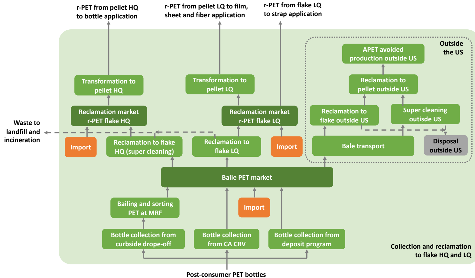
Figure B.7: Processes zoom-in on collection and reclamation to flake High Quality (HQ) and Low Quality (LQ).
