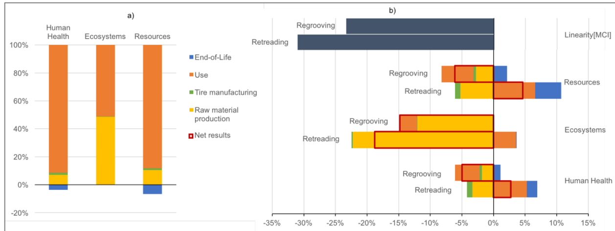
Figure 4.5: Results for the Brazilian context: a) Contribution analysis at the endpoint level of the baseline scenario; b) Relative variation of endpoint scores compared to the baseline scenario and impacts on circularity for retreading and regrooving scenarios
