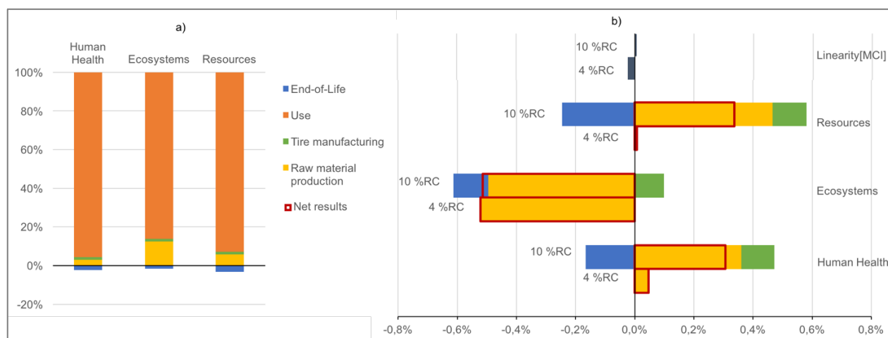
Figure 4.6: Results for the European context: a) Contribution analysis at the endpoint level of the baseline scenario; b) Relative variation of endpoint scores compared to the baseline scenario and impacts on linearity for the 4%RC and 10 RC scenarios.
