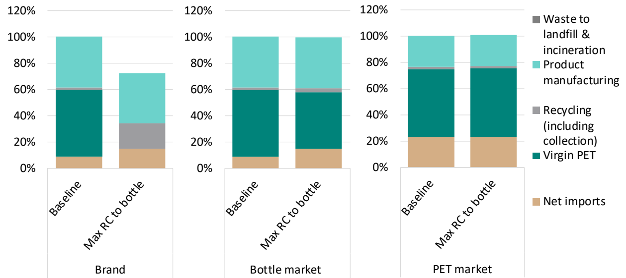
Figure B.13: Relative impact scores on Resources.
