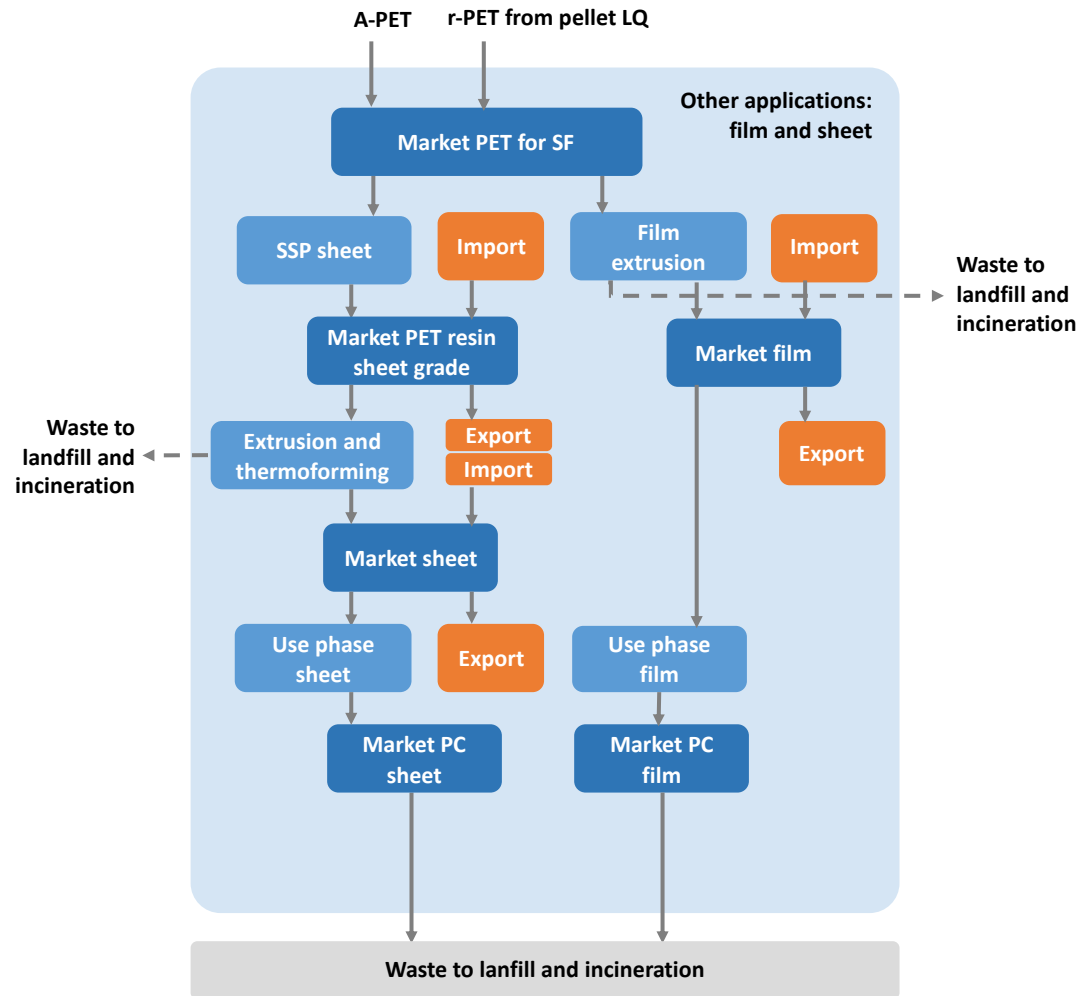
Figure B.6: Processes zoom-in on applications to film and sheet.
