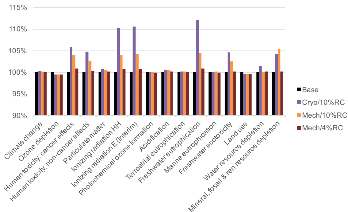
Figure A.10 Midpoint scores of recycled content scenarios, including a 10 %RC with cryogenic treatment.
