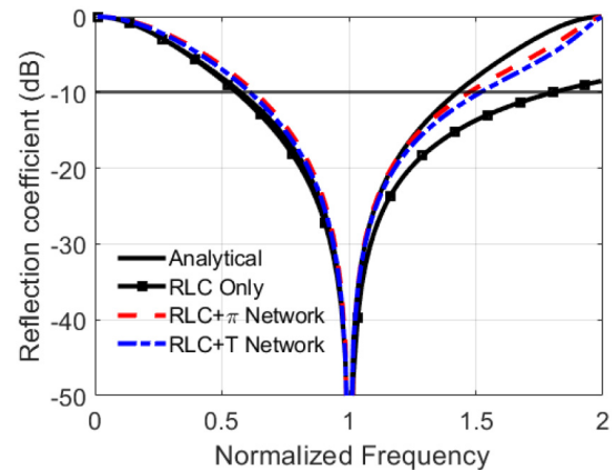
FIGURE 7. The reflection coefficient of the CSAA calculated using analytical expression [2, eq. (3.1)], RLC circuit only, RLC+PI and RLC+T network topologies.
