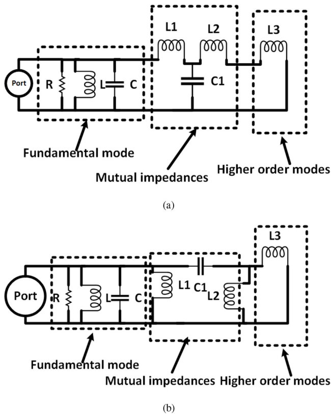
FIGURE 10. Complete lumped element-based equivalent circuit model of the CSAA: (a) equivalent RLC+T networks and (b) equivalent RLC+PI network.
