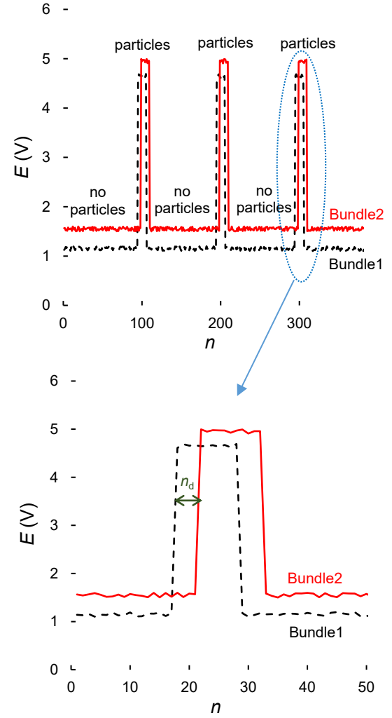
FIGURE 7 Voltage signals from three rotations of the chopper disk (top) and one rotation (bottom). When the glued particles pass in front of the probe, voltage signal is highest. Black and red lines show data of bundles 1 and 2, respectively. The lag, n_d , between the bundles 1 and 2 is the basis to calculate the effective length, l_e .
