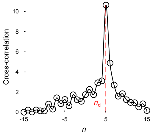
FIGURE 8 Cross-correlation curve for velocity calibration. The maximum cross-correlation occurs at data lag = n_d .
