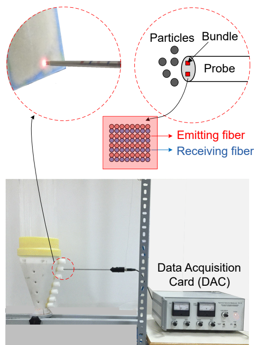
FIGURE 1 Schematic diagram of fiber optic probes. [14, 22] Each bundle consists of several sets of emitting and receiving fibers. We insert the optical probe into the multiphase bed, so that the probe tip lies in the bulk of particles. Emitting and receiving fibers are responsible for the emission of photons and transmission of the reflected photos from the surface of particles to a photo transistor. This photo transistor converts the light into an electrical voltage signal, which is recorded by a data acquisition card (DAQ).
