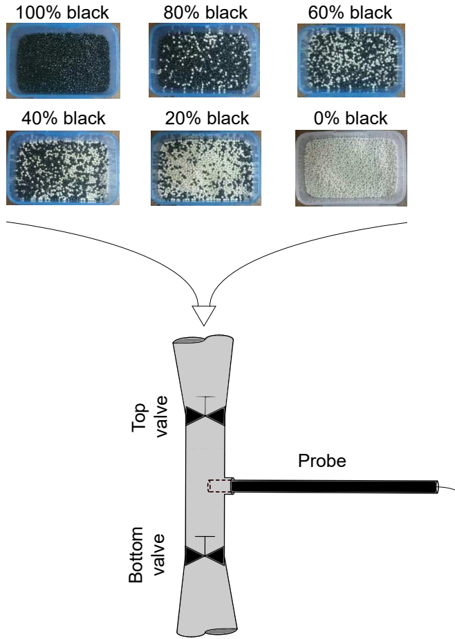
FIGURE 3 Optical probe calibration setup for solids holdup. Mixtures of various concentrations of black and white powder are poured into a downer with the probe protruding from the side through a hole. Valves at the bottom and top of the downer control the flow rate of the particles. We generate a calibration curve of the electrical signal and concentration of black powder, which represents the void fraction.
