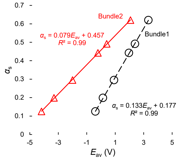
FIGURE 4 Typical solids holdup calibration curve. The holdup calibration curves relate (generally with a linear relation) the average voltage of the signals and the holdup values for each bundle.
