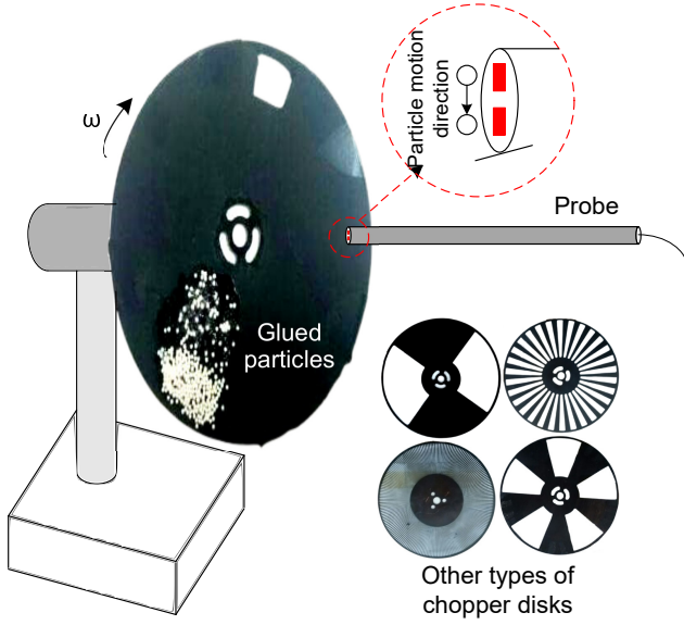
FIGURE 5 Particle velocity calibration experiments using a chopper disk comprised of black and white particles glued to the surface. A rotor rotates the disk at a rotational speed \omega . We place the probe tip orthogonal to the rotating disk at a distance of 1 mm to 2 mm.
