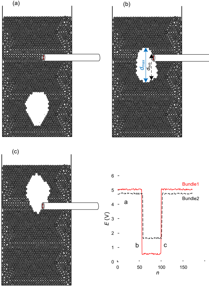
FIGURE 10 Possible positions of probe tip and a single bubble in a fluidized bed and corresponding voltage signals: (a) the bubble below the probe, (b) the probe inside the bubble, and (c) bubble above the probe. Red and black lines correspond to bundles 1 and 2, respectively.
