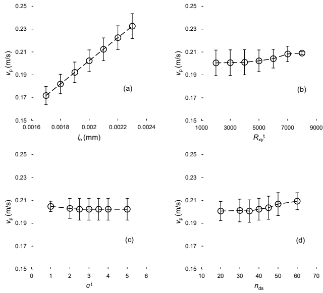
FIGURE 11 Sensitivity analyses on the effects of (a) effective length of the probe, (b) cross correlation threshold value, (c) standard deviation elimination threshold, and (d) number of data segments on particles velocity. We used the code in Appendix B, and the corresponding data for the sensitivity analyses. Error bars show the standard deviation of the particles velocity.
