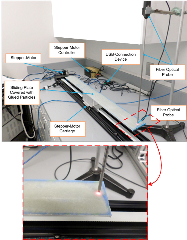
FIGURE 6 Calibration of fiber optic probe for velocity measurements of small particles with a belt-driven stepper motor. [22]
