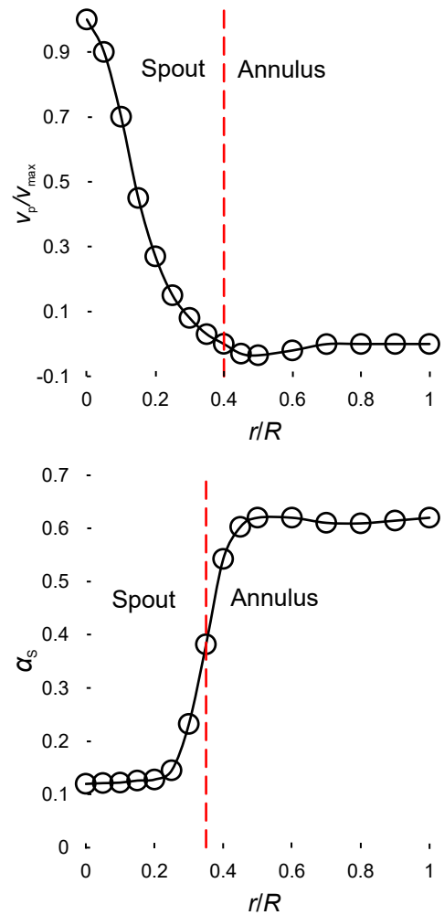
FIGURE 9 Typical particles velocity (a) and holdup (b) distributions in spouted beds. r denotes the radial distance from the spouted bed center.
