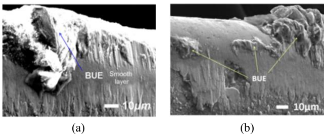
Fig.5. The BUE occurs within initial period when using cutting speeds (a) V_c = 50 m/min and (b) V_c = 60 m/min
