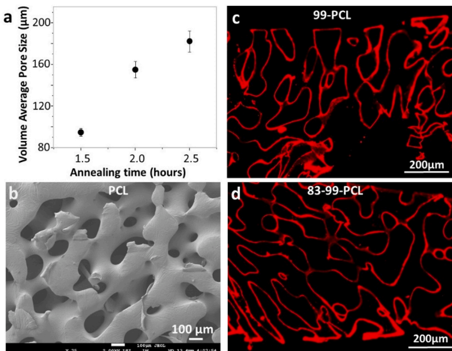
Fig. 1. Fabrication of porous PCL and chitosan coatings. (a) Scaffold blends of 45% PCL/55% PEO annealed for 1.5, 2 or 2.5 h yielded average pore sizes of 95 \pm 4 \mu\text{m} , 155 \pm 8 \mu\text{m} and 182 \pm 10 \mu\text{m} , respectively. (b) SEM image at 75 \times magnification of a PCL scaffold with average 155 \mu\text{m} pore diameter. Epifluorescent images of (c) 99-PCL (with RITC-99% DDA chitosan tracer) and (d) 83-99-PCL (coated with unlabeled 99% DDA chitosan and then 83% DDA chitosan containing RITC-83% DDA chitosan tracer).
