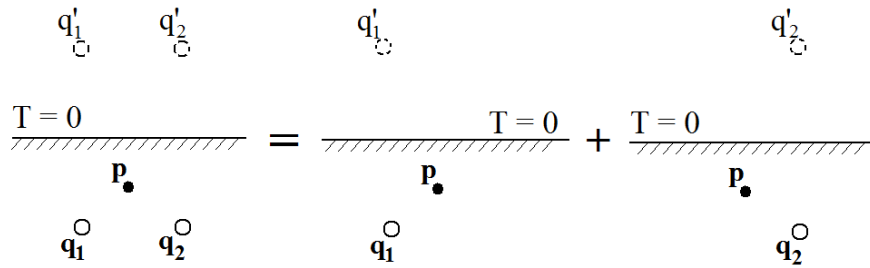
Figure 3.5 Illustration du principe de superposition spatiale.
