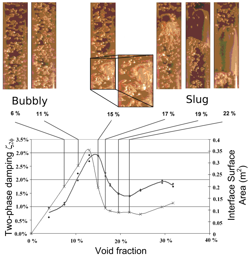
Figure 5.9 Damping ratio and interface surface area in air/alcohol mixtures (◇: two-phase damping; × interface surface area). from Anscutter et al. (2006)
