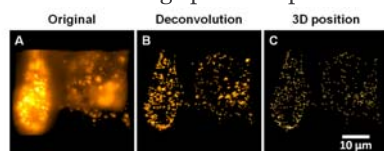
Fig. 2. Image treatment. (A) 3D image of EGFR-AuNSs on MDA-MB-231 cells obtained with 100 nm step z-scan by RLM set-up. (B) Deconvolution of the image using experimental point-spread function. (C) 3D position of NPs obtained by local maximum filter and 3D Object Counter (ImageJ).
