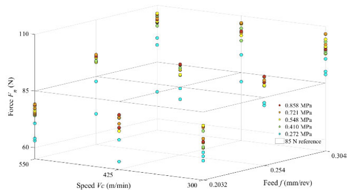
Fig. 5. Cutting forces F_n results plotted vs the feed, speed and cutting pressure
