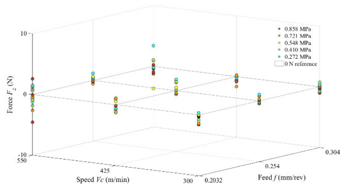
Fig. 6. Cutting forces F_z results vs the feed, speed and cutting pressure
