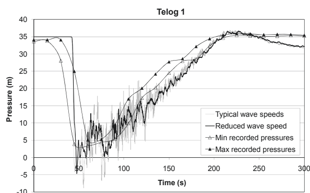
Figure 2. Comparison of pressures recorded at one distribution system site with pressures modelled with typical wave speeds and with a reduced wave velocity in cast-iron pipes (four pressure values per second were measured by the pressure recorders but only the minimum and maximum pressures over 15 s intervals were saved ( \Delta and \blacktriangle )).
