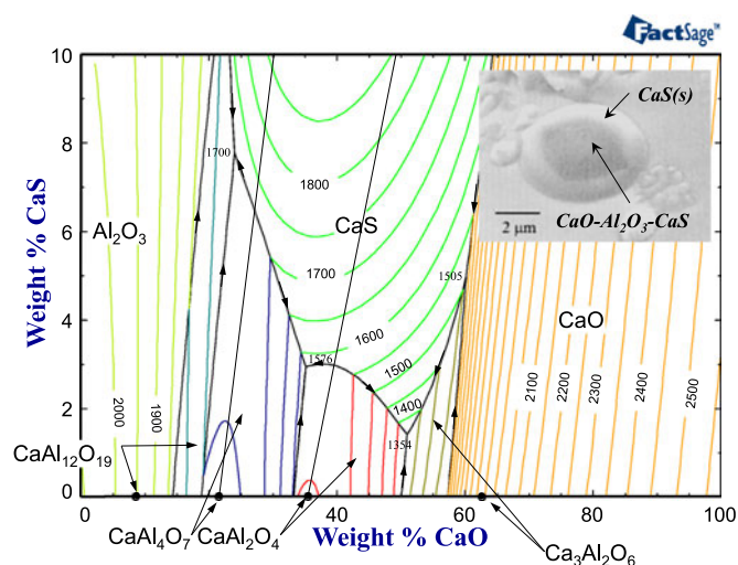
Fig. 2. FTOxid database – calculated liquidus projection of \text{CaO-Al}_2\text{O}_3\text{-CaS} oxy-sulfide system (FTOxid database) and inclusions found in Al-killed steel followed by \text{Ca} injection (inset [4]).
