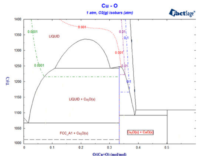
Fig. 34. Phase Diagram module – calculated O 2 (g) isobars in the Cu–O binary systems using data from FScomp.
