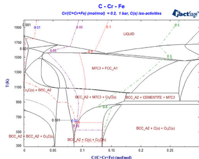
Fig. 36. Phase Diagram module – calculated C(s) iso-activity lines in the Fe–Cr–C ternary system.
