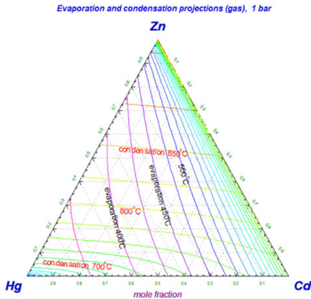
Fig. 21. Phase Diagram module – gas evaporation and condensation polythermal projections of the Zn–Hg–Cd ternary system, 1 bar.
