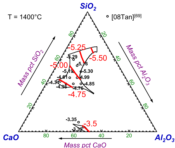
Fig. 37. Phase Diagram module – calculated iso-sulfide capacity ( C_s ) lines of CaO–SiO 2 –Al 2 O 3 slag at 1400 °C with the calculated liquidus (thin lines) [25] using data from FToxid .
