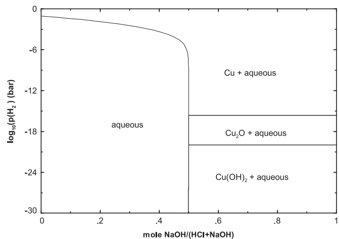
Fig. 38. Phase Diagram module – calculated partial pressure of H_2 vs. molar ratio NaOH/(NaOH + HCl) for the system H_2O –Cu–NaOH–HCl– H_2 , molality of Cu = 0.001.
