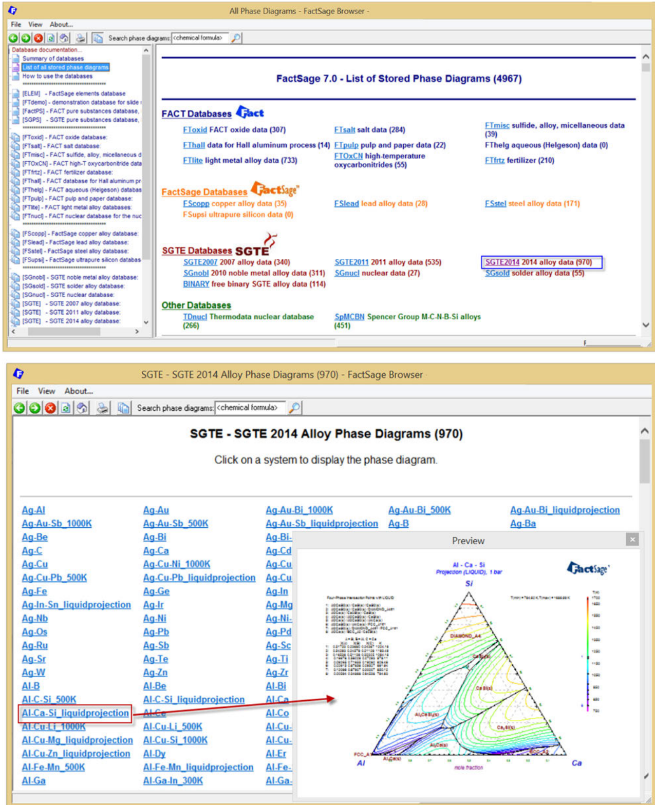
Fig. 5. FactSage Browser module – list of stored phase diagrams; summary of figures and display of the Al–Ca–Si liquidus polythermal projection taken from the SGTE 2014 database.
