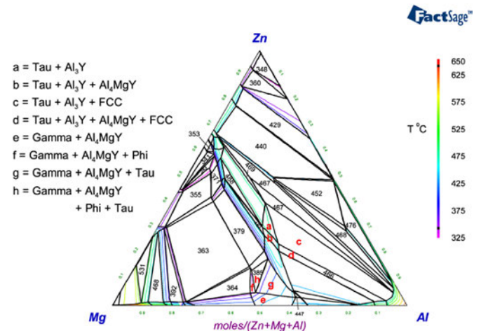
Fig. 28. Phase Diagram – Zn-Mg-Al-Y polythermal first-melting (solidus) projection at X_Y = 0.05 using data from FTLite.
