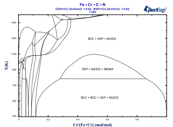
Fig. 29. Phase Diagram – T(K) vs. \text{Cr}/(\text{Fe} + \text{Cr}) phase diagram of the Fe-Cr-C-N system at \text{C}/(\text{Fe} + \text{Cr}) = 0.02 and \text{N}/(\text{Fe} + \text{Cr}) = 0.02 calculated under normal equilibrium conditions (ortho-equilibrium) using data from FSstel.
