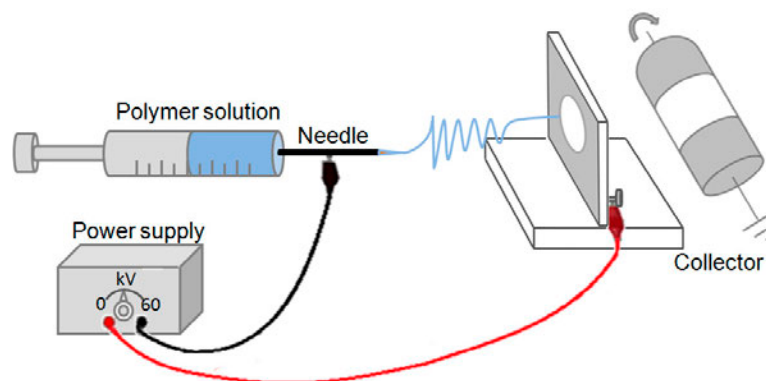
Figure 7. Schematic representation of the home-made electrospinning set-up.
