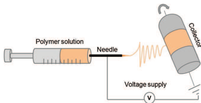
FIGURE 1 Schematic representation of the homemade electrospinning set up
