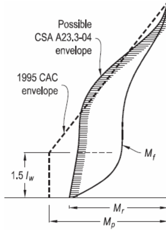
Fig. 1.3: Capacity design moment envelopes for ductile RC walls (Boivin and Paultre 2010).
