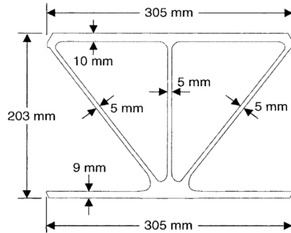
Figure 2.7 : Extrusion AlumaDeck (Burgelin, 2017)
