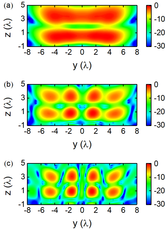
Figure 3.3 Normalized E-field distribution of NFMF on focal plane x = -8\lambda : (a) N_y = N_z = 10 ; (b) N_y = N_z = 11 ; (c) N_y = N_z = 14 .
