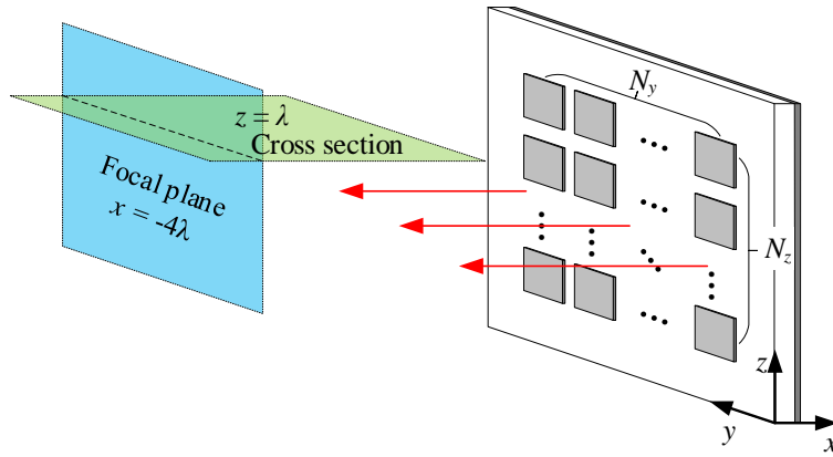
Figure 2.12 Configuration of transmitting antenna array on yoz plane and focal plane on yz -plane.
