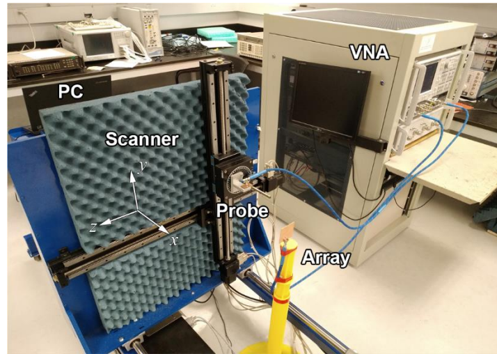
Figure 4.36 Practical testing environment for near-field scanning of 4 \times 4 NFMF array.
