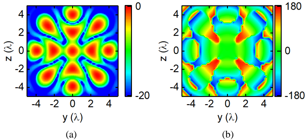
Figure 4.6 Example of spatial power splitting with circular distributed form distributed targets: (a) normalized amplitude (dB); (b) phase (degree).
