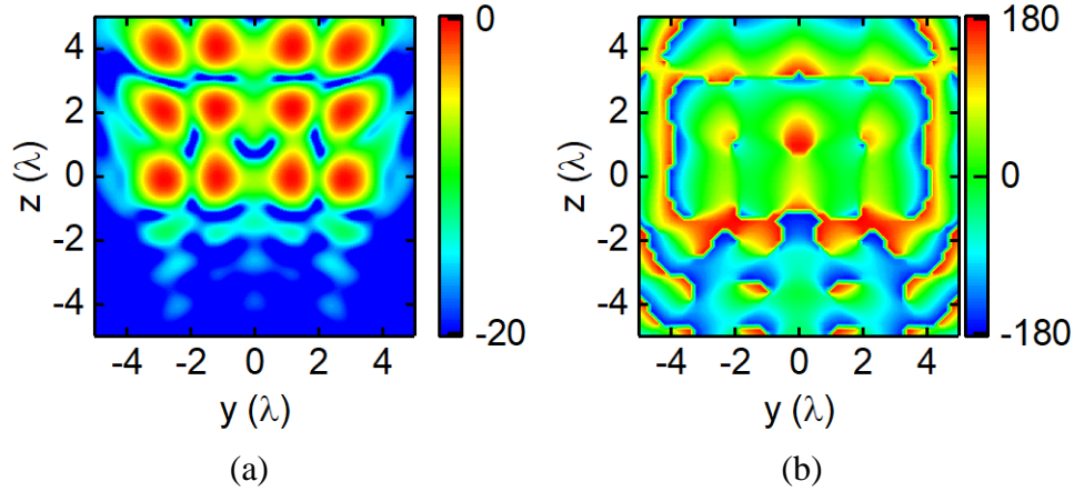
Figure 4.5 Example of spatial power splitting with matrix-form distributed targets: (a) normalized amplitude (dB); (b) phase (degree).
