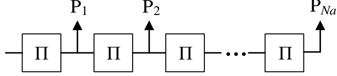
Figure 3.9 Cascaded Pi networks for multiple outputs with unequal distributed amplitude and phase.
