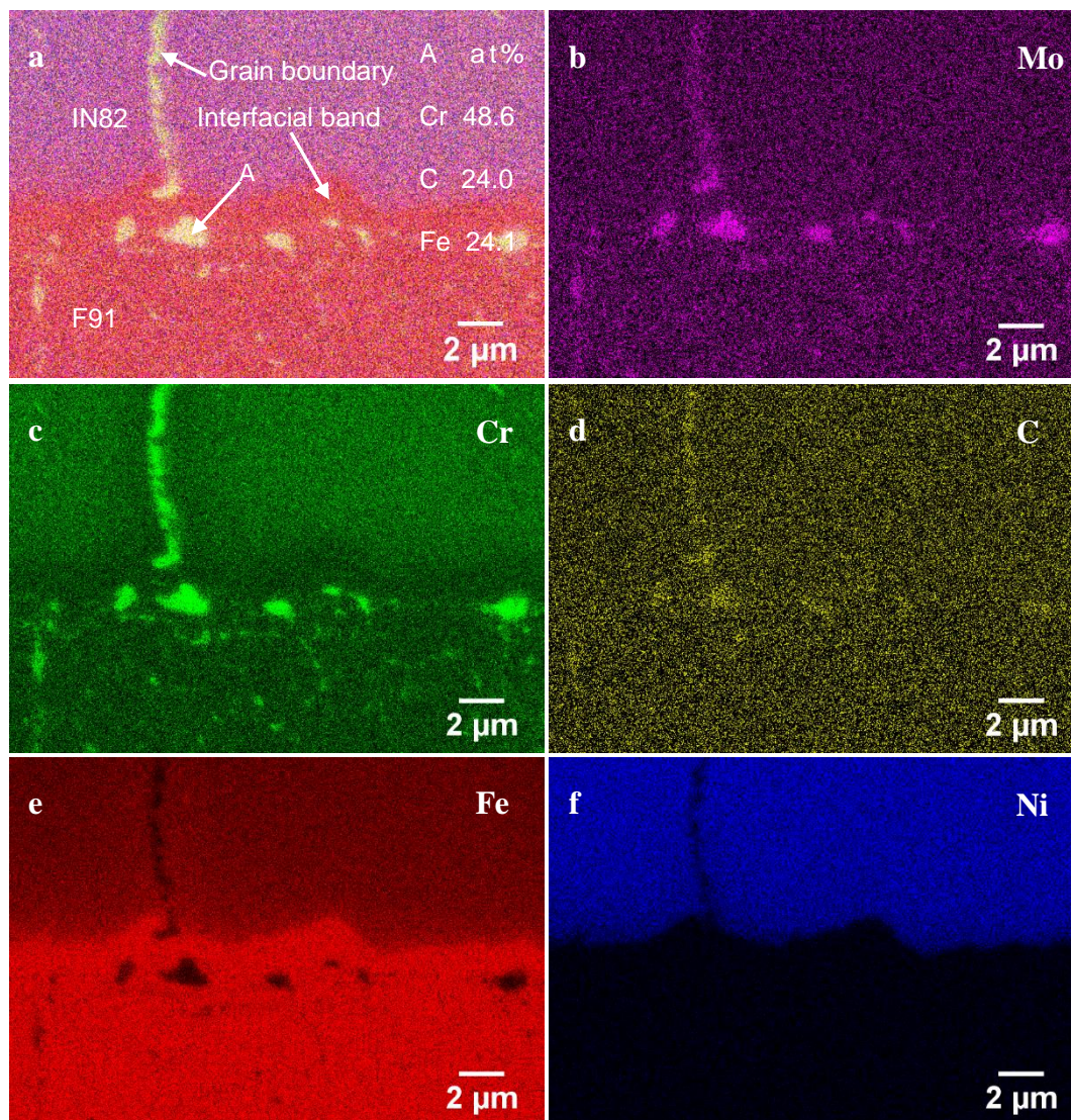
Figure 8.7: EDS elemental mapping on the F91/IN82 interface of a specimen aged at 650 °C for 8760 h: (a) EDS composite map; (b) Mo, (c) Cr, (d) C, (e) Fe, and (f) Ni elemental maps.
