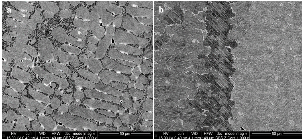
Figure 3.4: SEM micrographs of (a) S6 and (b) S21 showing the dendrite structure.
