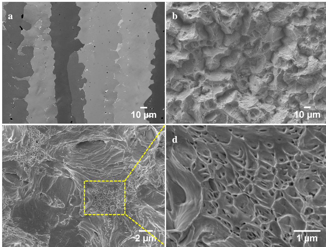
Figure 8.5: SEM micrographs of an IN82 specimen aged at 650 °C for 8760 h: (a) dendritic microstructure; (b) the intergranular/interdendritic cracks, (c) higher magnification view, and (d) the zone outlined by the rectangle showing the microvoids surrounded by dimples.
