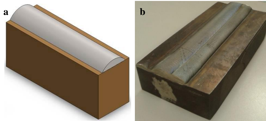
Figure 4.1: Hardfacing component: (a) illustration and (b) manufactured.
