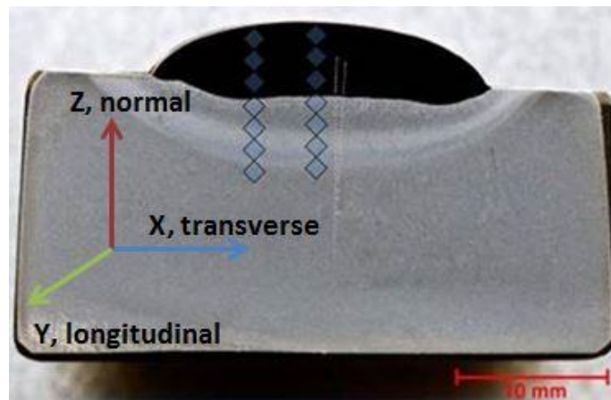
Figure 4.14: Cross-section of a hardfacing component with neutron diffraction measurement locations indicated.
