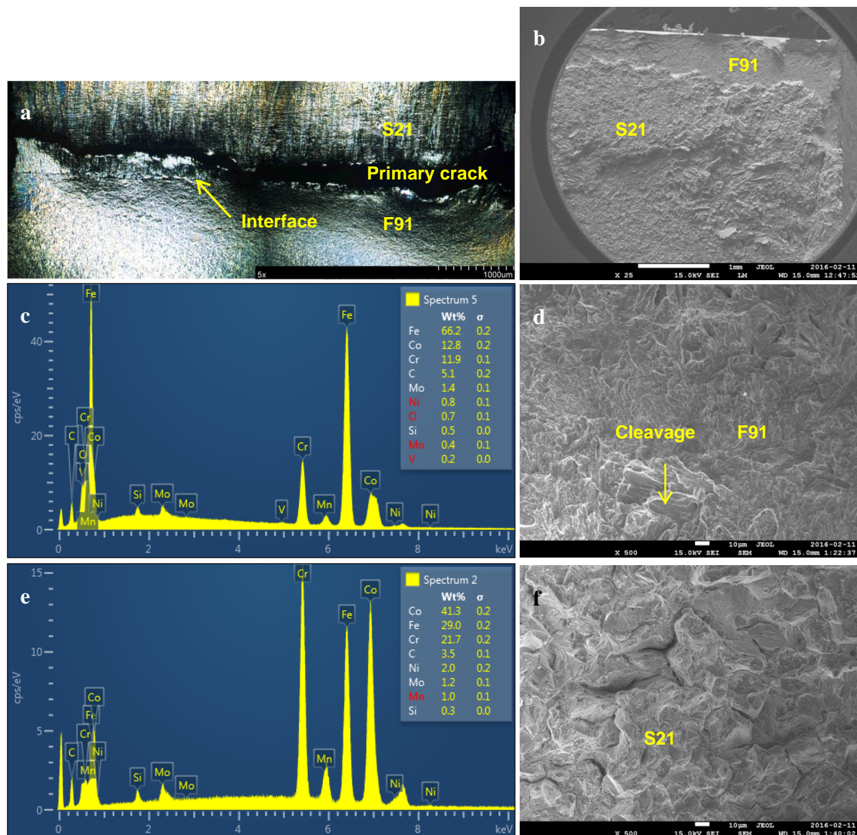
Figure G.7: A fractured S21 specimen in the as-tempered condition: (a) cross-section, (b) macro-fractograph, (c) EDS spot measurement on the F91 region, (d) fractograph showing cleavage in the F91, (e) EDS spot measurement on the S21 region, (f) fractograph showing the interdendritic cracks.
