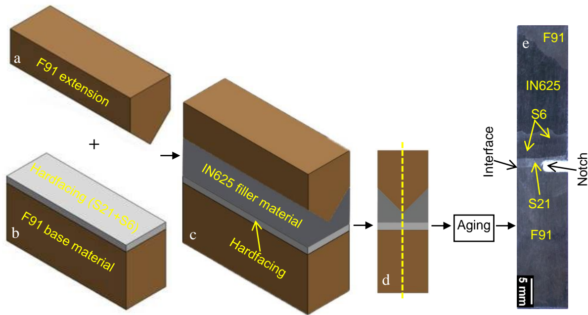
Figure 7.1: Charpy specimen manufacturing: (a) F91 extension, (b) Stellite-hardfaced coating with buffer layer of S21 and top layer of S6, (c) assembly made by welding an F91 extension to the Stellite-hardfaced coating sample using IN625 as the filler material, (d) bars cut from the assembly, and (e) Charpy U-notch specimen machined from the half bars (cross-section).
