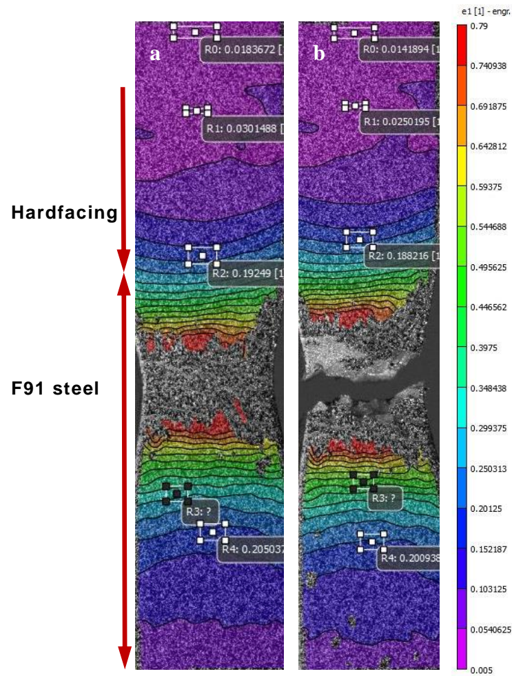
Figure 9.10: Principle strain maps of a tensile specimen aged at 550 °C for 1008 h: (a) before and (b) after fracture.
