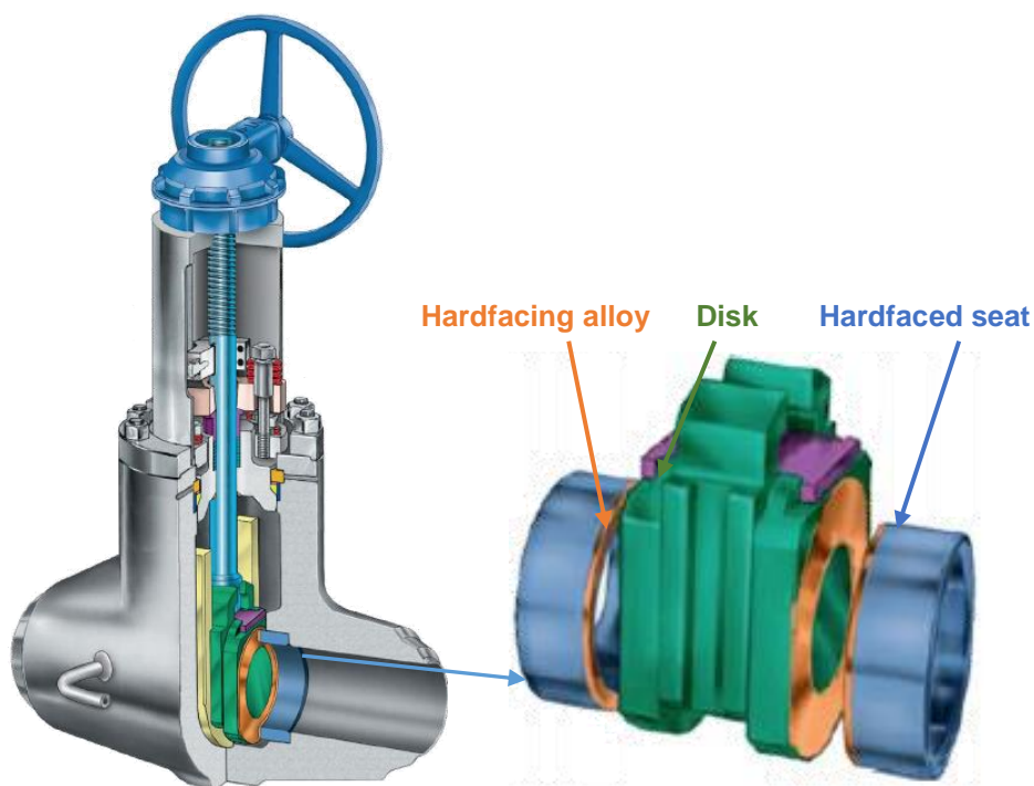
Figure 1.2: A Velan parallel slide gate valve (courtesy of Velan Inc.).
