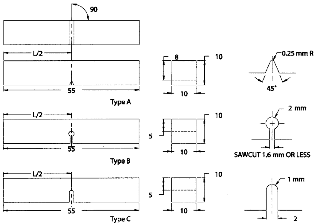
Figure 4.6: There types of Charpy (simple-beam) specimens [44].
