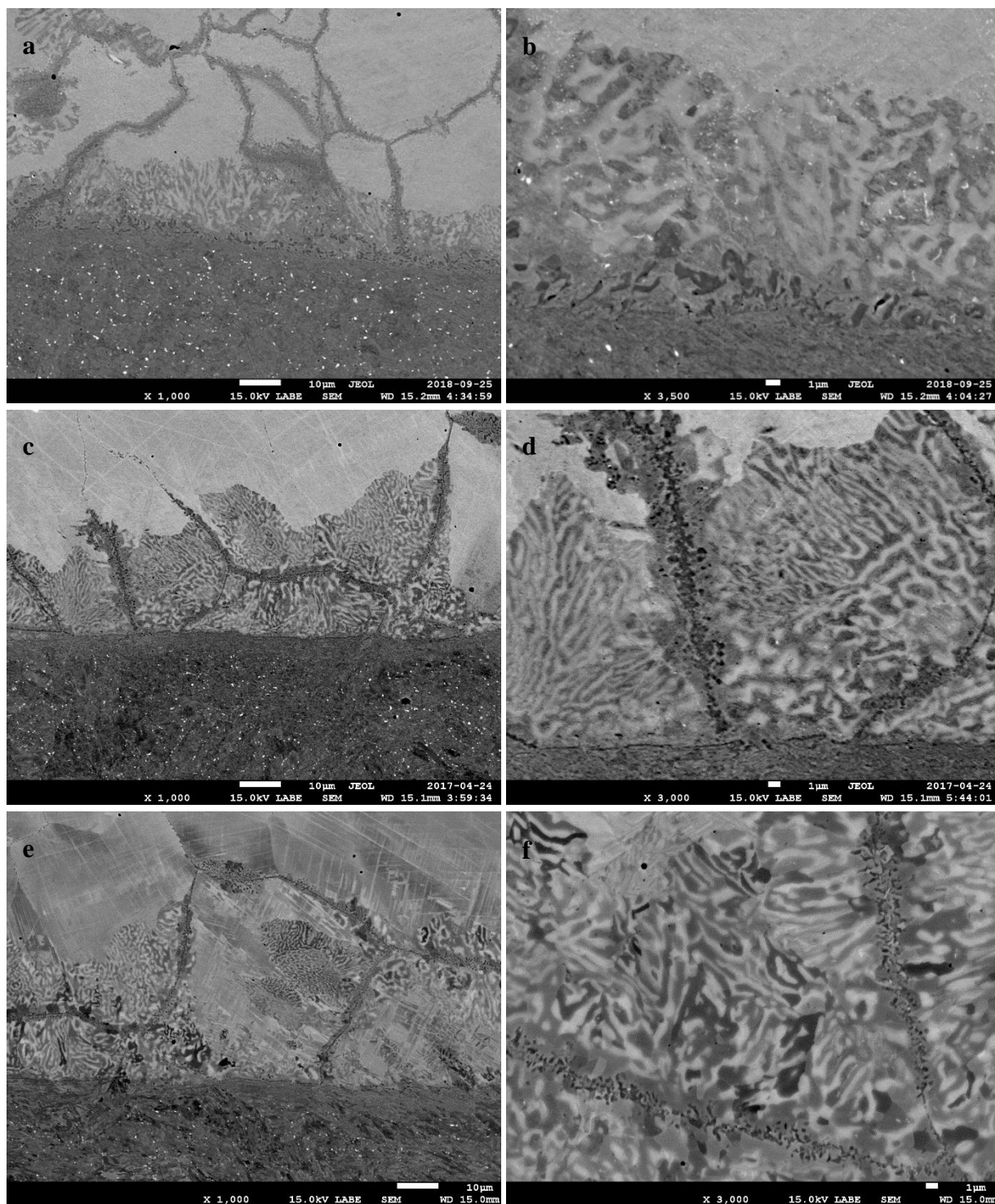
Figure 10.5: Steel/S21 interfacial microstructure: (a) and (b) from the ex-service component; from the laboratory sample aged at 550 °C for 8760 h (c) and (d) polished up to 1 \mu\text{m} , (e) and (f) further polished using a mixed colloidal silica suspension.
