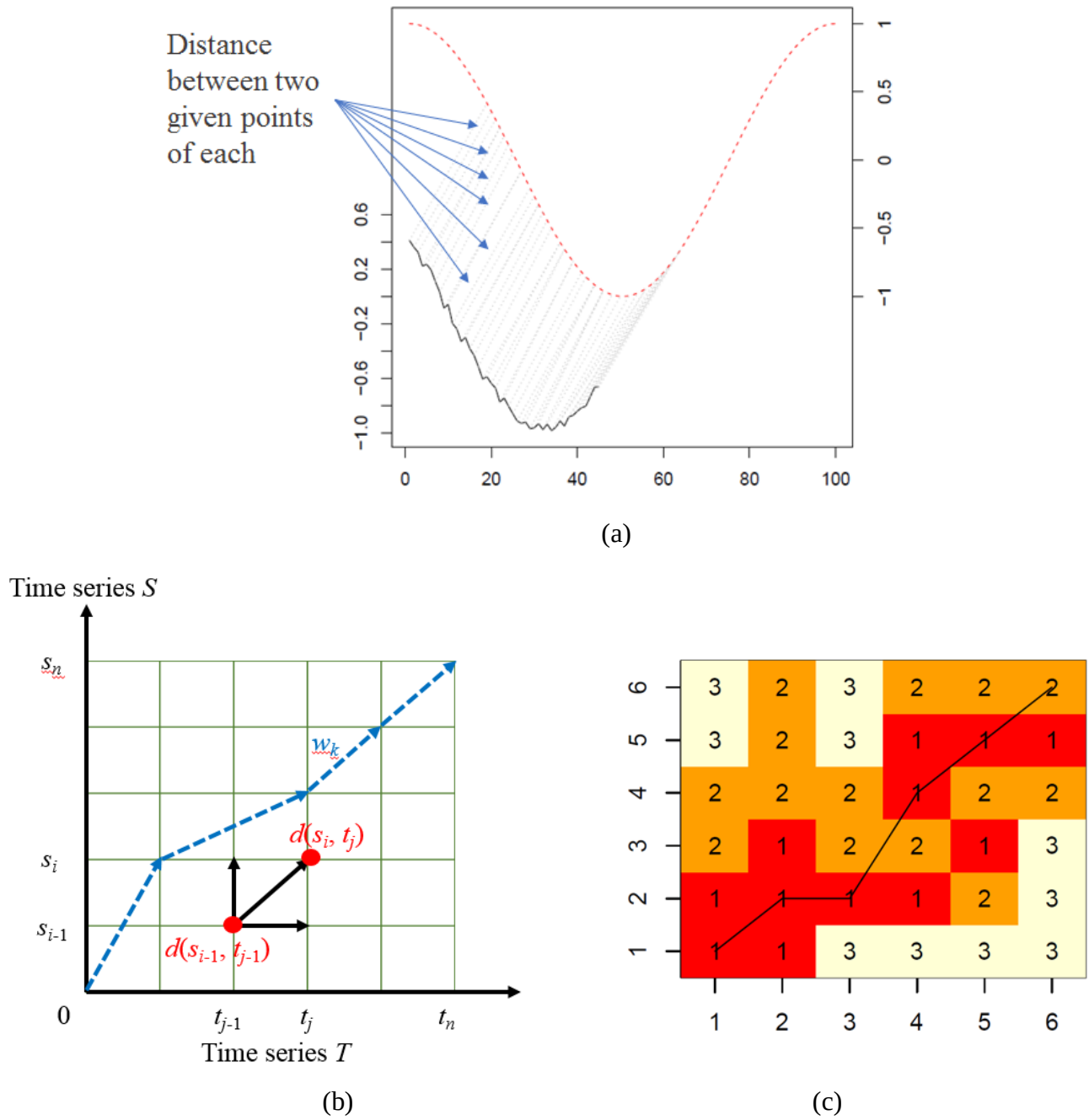
Figure 6-1: Dynamic time warping method
