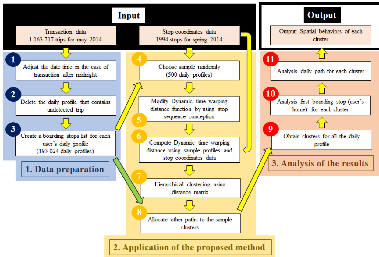
Figure 6-4: Proposed method
