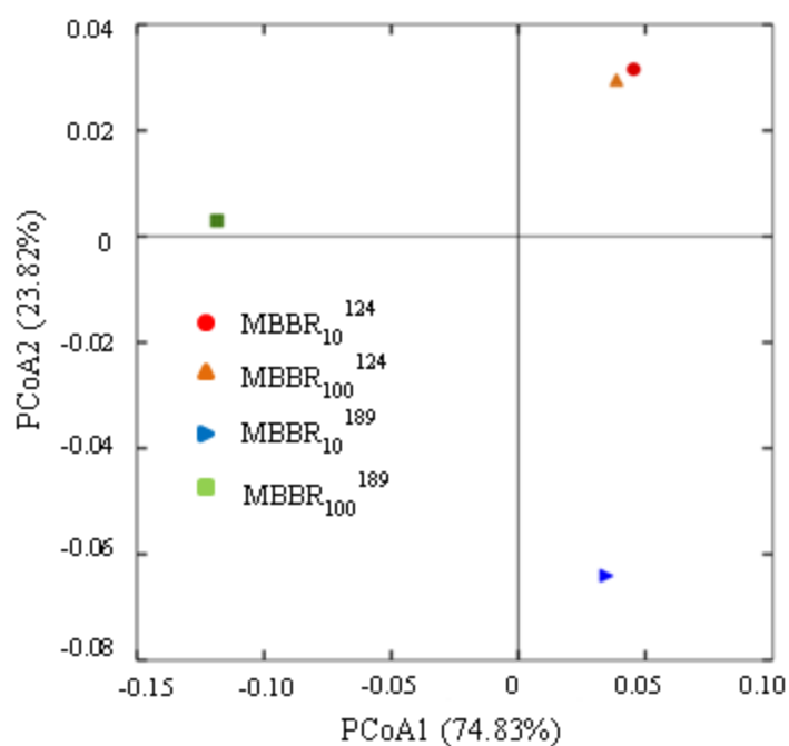
Figure B.9 : Principal coordinates analysis (PCoA) of weighted UniFrac distance based on 16S rDNA genes at different AgNP concentrations. Note: The characters 124 and 189 represents the biofilm collected in control period (day 124) and AgNP-treated biofilms at the end of the exposure period (day 189), respectively; MBBR 10 and MBBR 100 received nominal influent AgNP concentrations of 10 and 100 µg/L respectively over AgNP exposure period.
