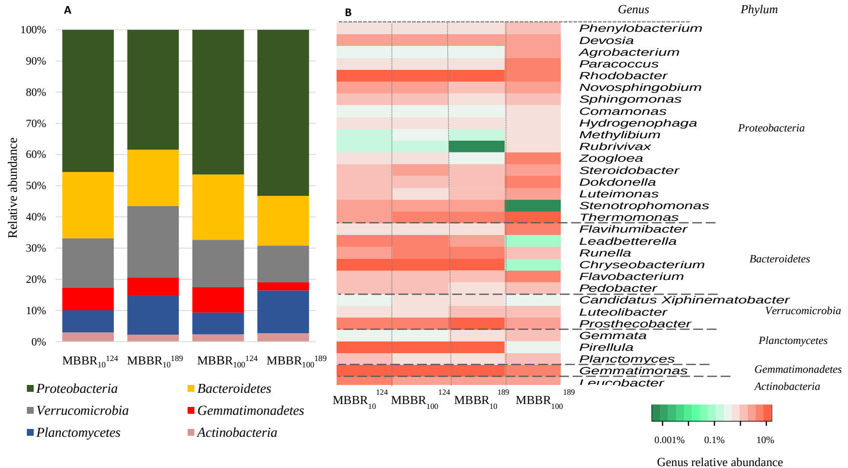
Figure 5.5: (A) Taxonomic classification of 16S rDNA paired-end sequencing from the biofilm samples at different AgNP concentrations at phylum level and (B) heatmap of genera with total sequence reads higher than 150 in selected phyla. Note: Superscripts 124 and 189 represent the biofilms collected at the end of control period (day 124) and after 64 days of AgNPs exposure (day 189) in MBBRs, respectively.
