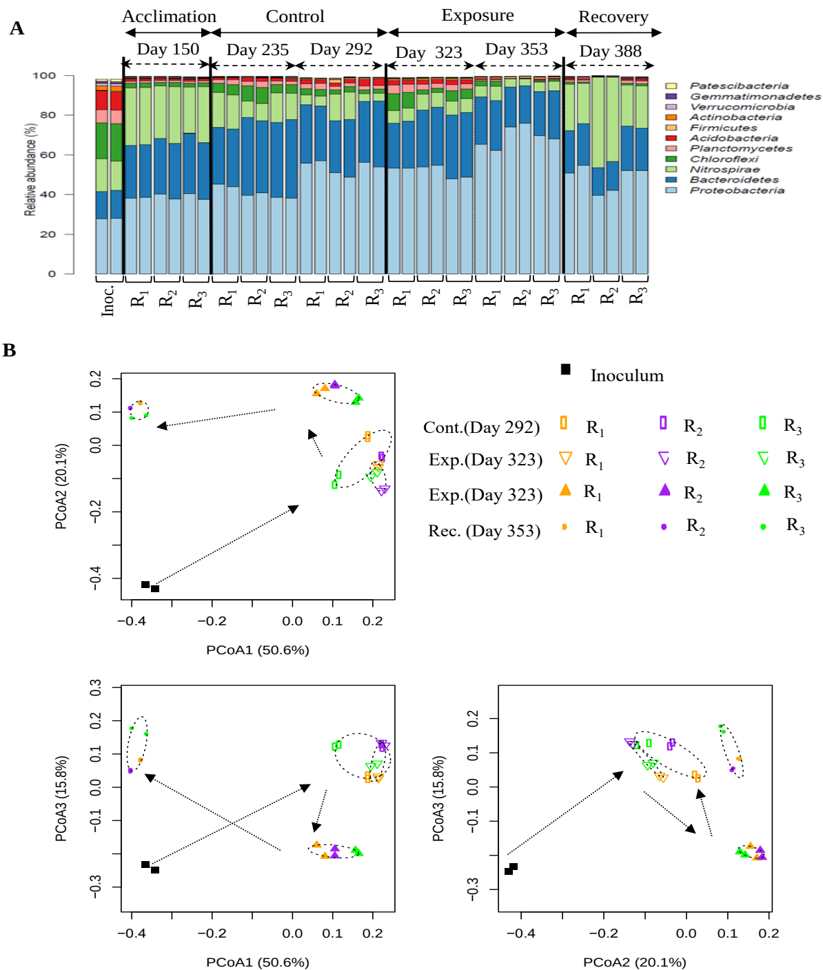
Figure 6.5: (A) Bacterial community composition of nitrifying MBBR 1 (R 1 ), MBBR 2 (R 2 ) and MBBR 3 (R 3 ) at different stages of operations (Acclimation, Control, AgNP Exposure, Recovery) at phylum level; (B) Principal coordinate's analysis (PCoA) based on Bray–Curtis distance in control (R 1 ) and Ag-treated reactors (R 2,3 ) in Control, Exposure and Recovery phases.
