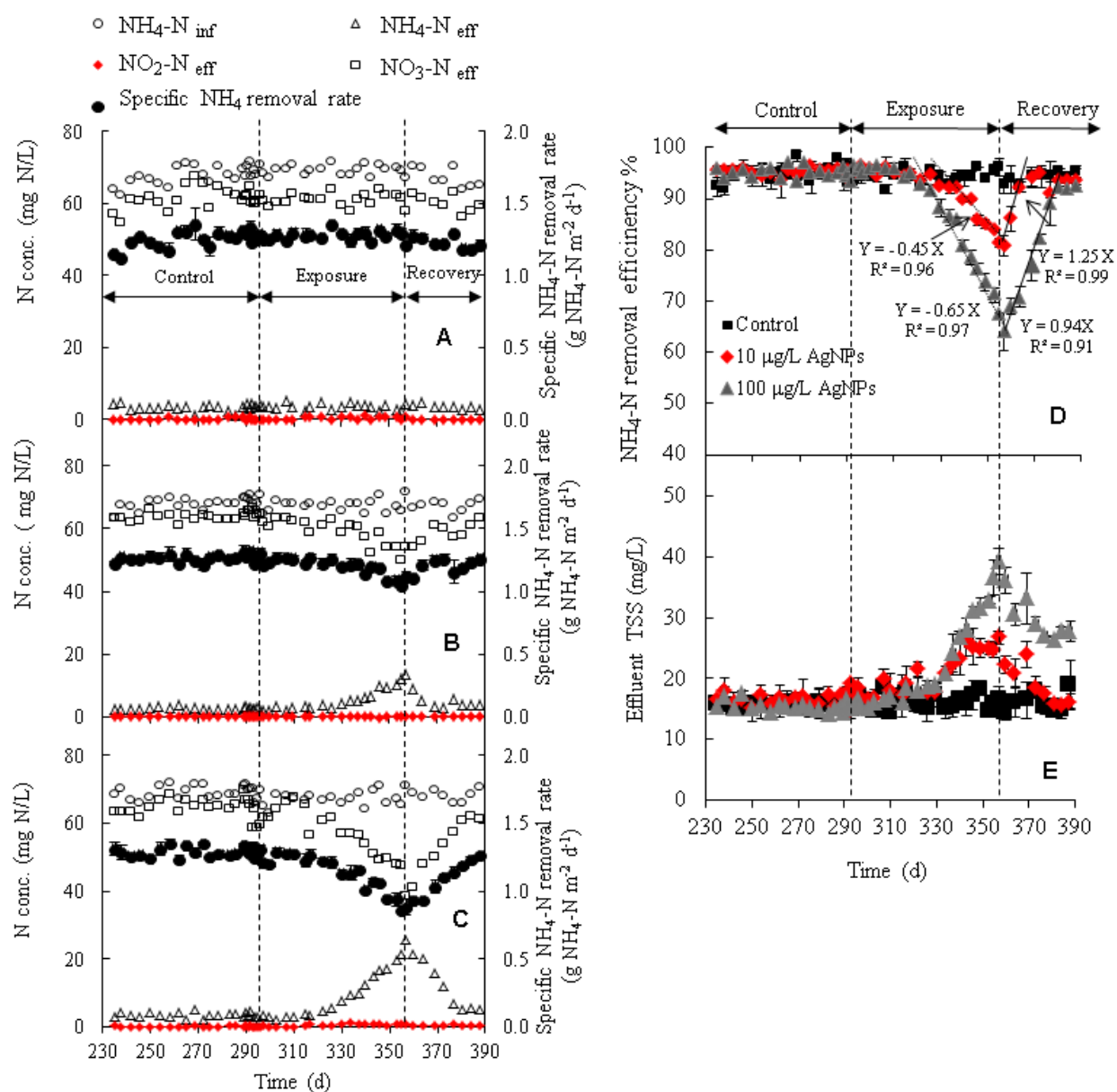
Figure 6.2 : Effect of PVP-AgNPs on nitrifying MBBR performance at (A) control, (B) 10 \mu\text{g/L} AgNPs, (C) 100 \mu\text{g/L} AgNP and (D) ammonia removal efficiency; (E) effect of AgNP addition on MBBR \text{TSS}_{\text{eff}} (error bars are only shown when larger than symbol size).
