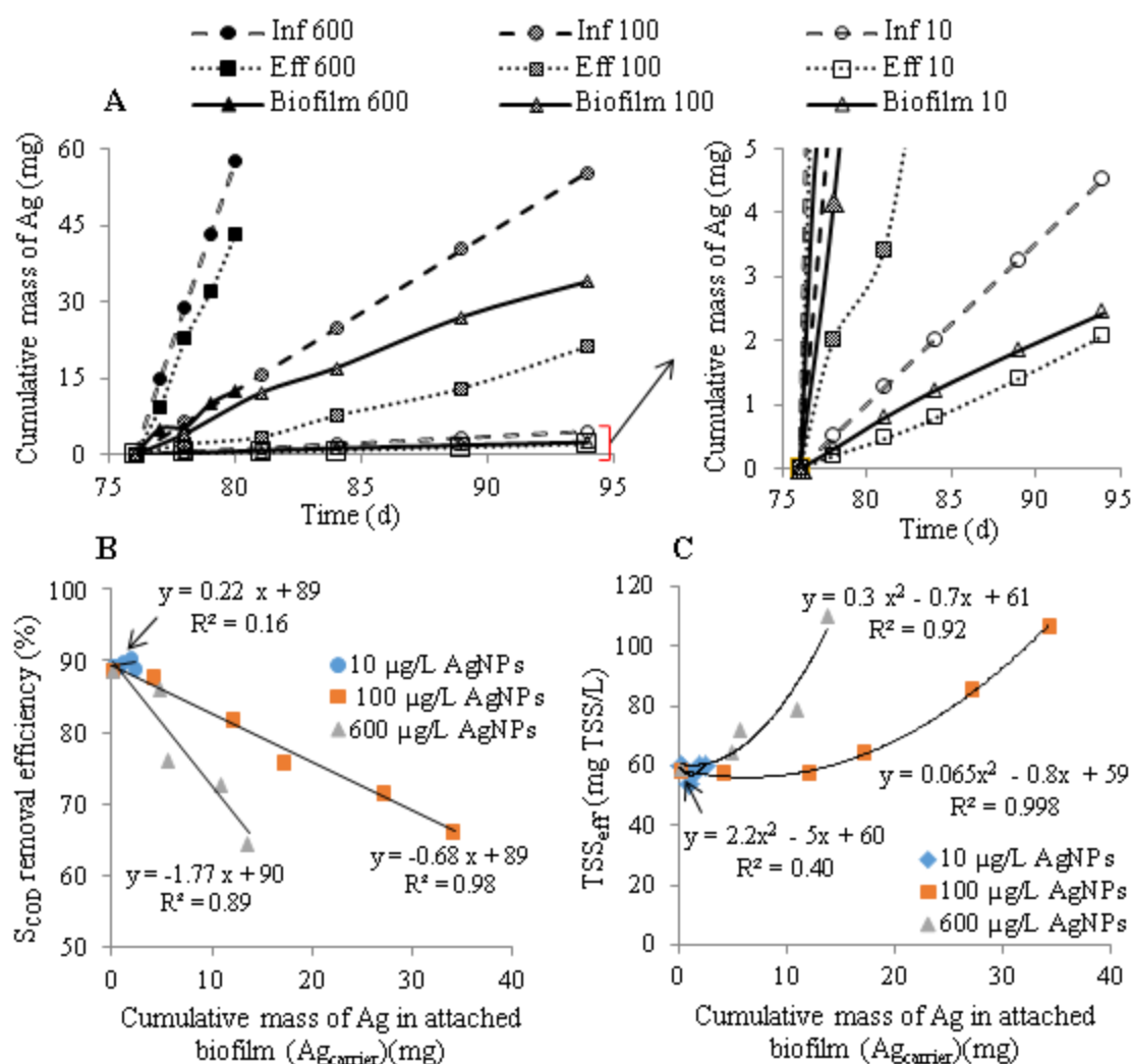
Figure 4.6 : Cumulative Ag mass balance in influent (Inf) effluent (Eff) and attached biofilm (Biofilm), (B) correlation between Ag_{carrier} and SCOD removal efficiency and (C) correlation between Ag_{carrier} and TSS_{eff} (Note: negligible Ag_{susp} ).
