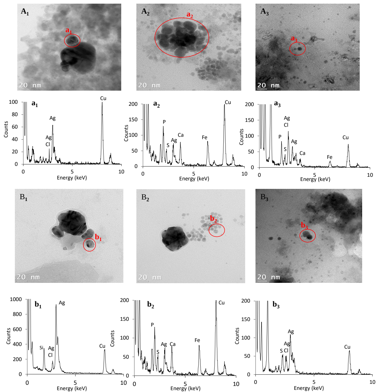
Figure C. 2: TEM images of the AgNPs in the effluent of MBBR receiving (A 1-3 ) 10 µg/L and (B 1-3 ) 100 µg/L AgNPs and (a 1 -b 3 ) EDS analysis of the AgNPs.(Note: Subscripts 1 and 2 correspond to the end of the exposure period (day 353) and subscript 3 represent the end of the recovery phase (day 388)).
