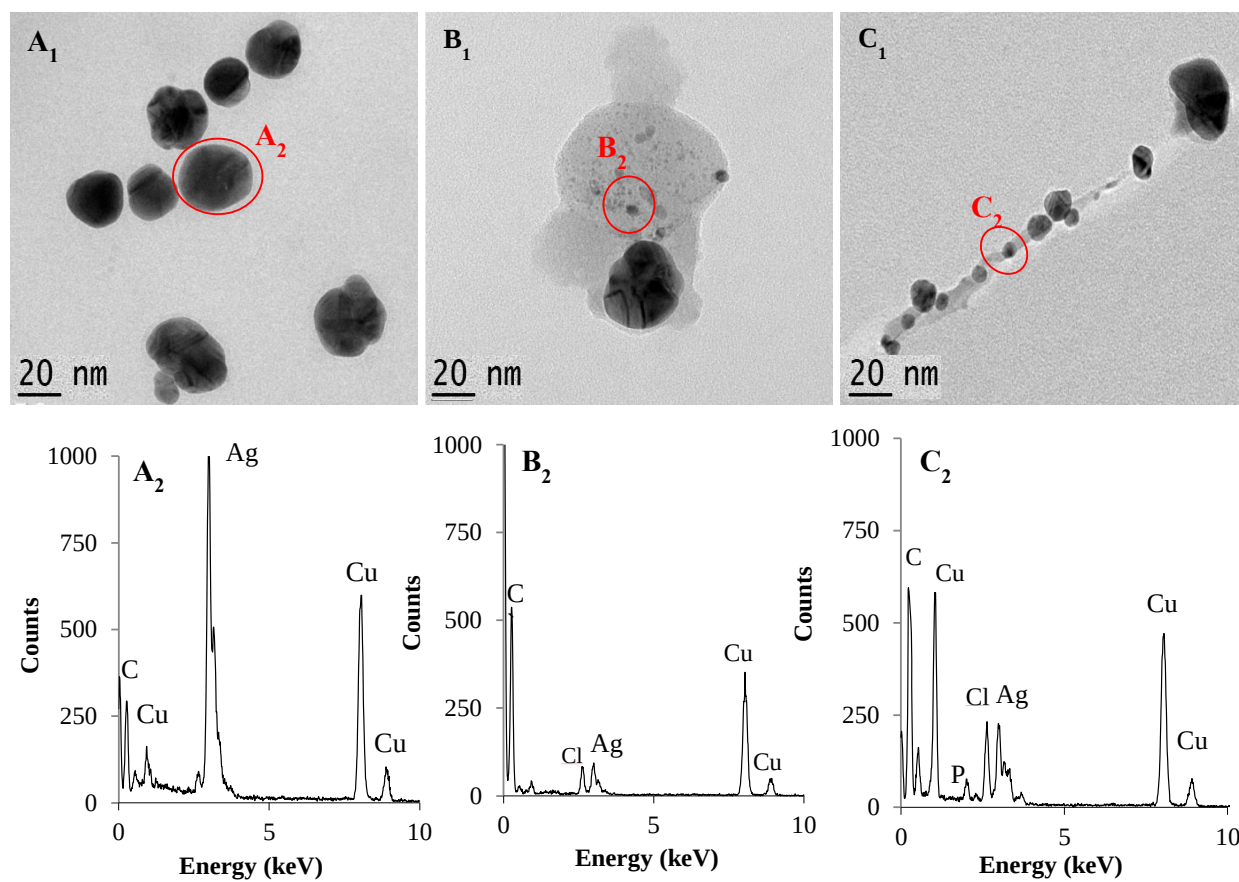
Figure B.7 : TEM images of the AgNPs in (A 1 ) influent and effluent of MBBR receiving (B 1 ) 10 \mu\text{g/L} (C 1 ) 100 \mu\text{g/L} AgNPs and (A 2 -C 2 ) EDS analysis of the AgNPs.
