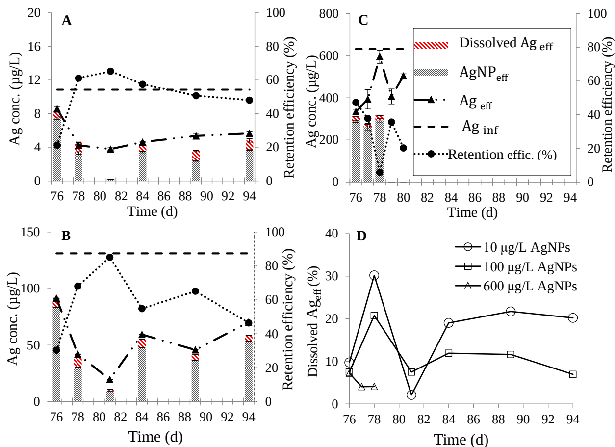
Figure 4.5 : Fate and retention of Ag in MBBRs receiving influent concentration of (A) 10 µg/L, (B) 100 µg/L, (C) 600 µg/L AgNPs and (D) dissolution of AgNP eff (error bars are only shown when larger than symbol size).
