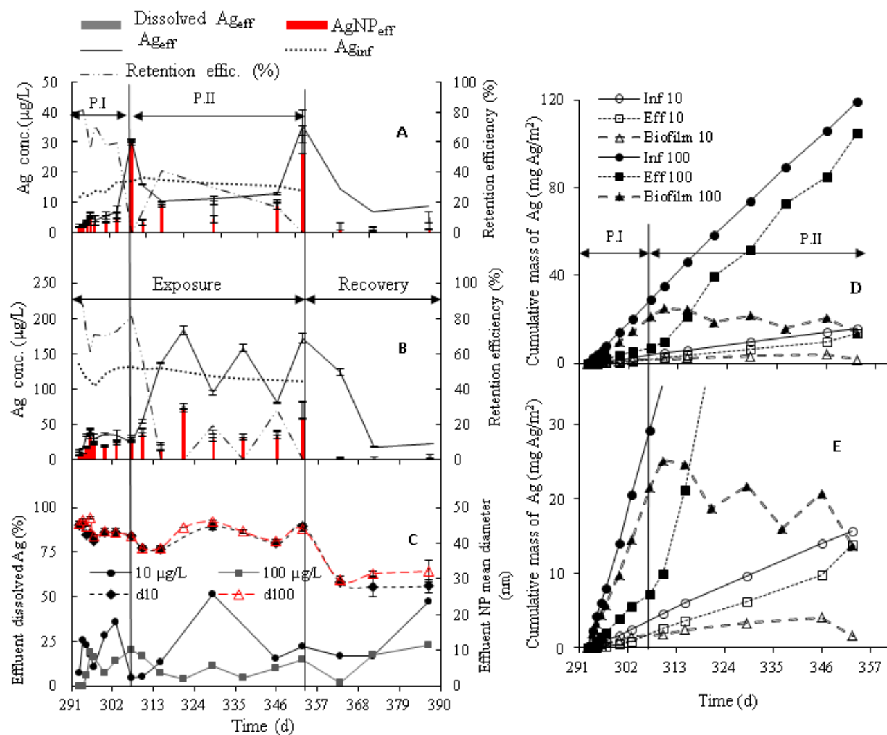
Figure 6.1: Fate and retention of Ag in MBBR receiving nominal AgNP influent concentration of (A) 10 µg/L (MBBR 2 ) and (B) 100 µg/L AgNPs (MBBR 3 ); (C) AgNP eff mean diameter and dissolution of AgNP eff (%); (D) cumulative Ag mass distribution in influent (Inf), effluent (Eff) and attached biofilm (Biofilm), (E) enlarged Y-scale of panel D. Note: P.I-II refers to two observed phases in Ag distribution profile.
