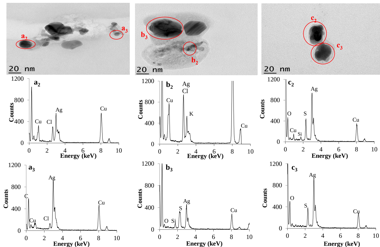
Figure A.2: TEM images of the AgNPs in effluent of MBBR receiving (A 1 ) 10 µg/L, (B 1 ) 100 µg/L and (C 1 ) 600 µg/L AgNPs and (a 2 -c 3 ) EDS analysis of the AgNPs.
