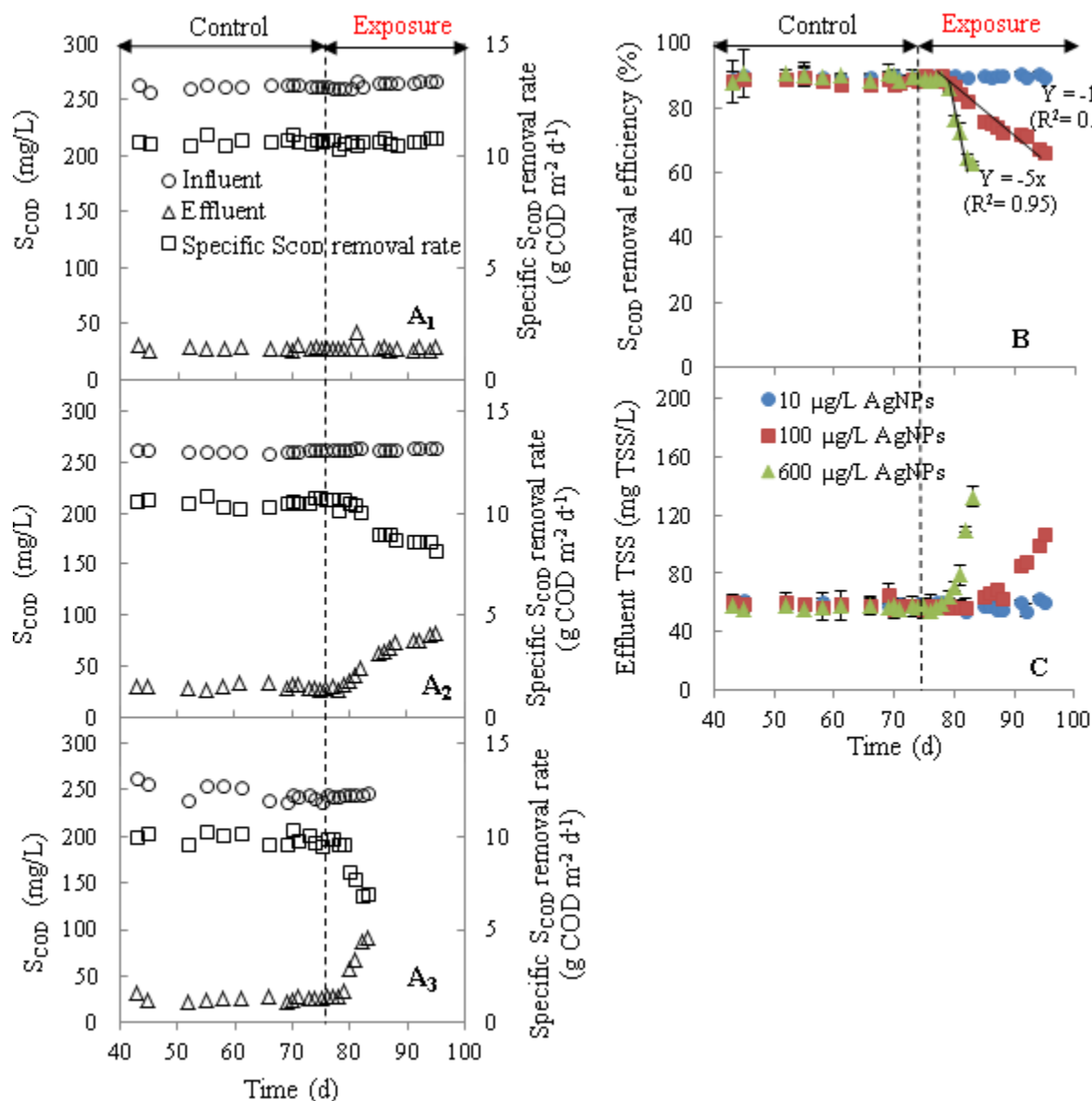
Figure 4.3 : Effect of PVP-AgNP addition on MBBR performance at (A 1 ) 10 \mu\text{g/L} AgNPs (A 2 ) 100 \mu\text{g/L} AgNPs, (A 3 ) 600 \mu\text{g/L} AgNPs, (B) S_{\text{COD}} removal efficiency and (C) Effect of AgNP addition on MBBR \text{TSS}_{\text{eff}} (error bars are only shown when larger than symbol size).
