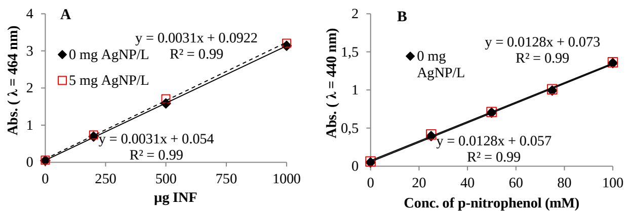
Figure B.4 : Calibration curves used in (A) intracellular DHA and (B) extracellular \alpha -glucosidase activity assay at different Ag concentrations.
