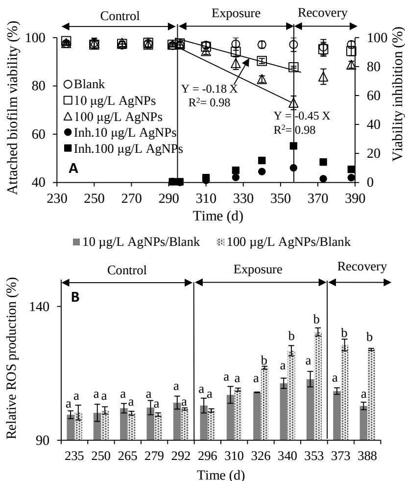
Figure 6.3: Long-term effect of PVP-AgNPs addition on (A) viability and (B) relative intracellular ROS generation of attached biofilm. Different superscript letters represent significant difference ( p < 0.05 ) (error bars are only shown when larger than symbol size).
