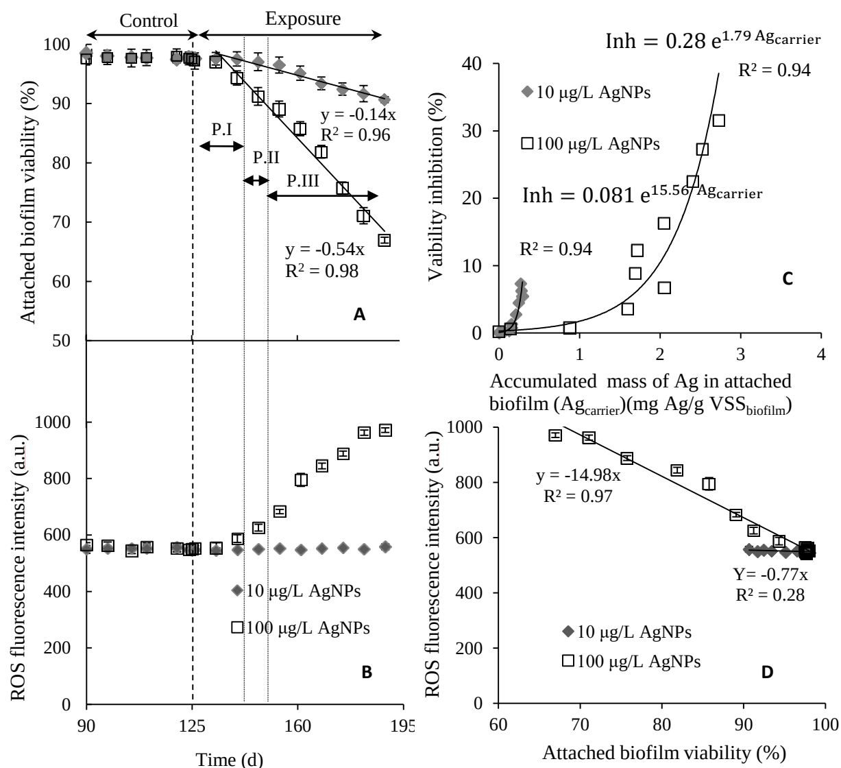
Figure 5.3: Effect of continuous PVP-AgNP injection on (A) attached cell viability, (B) intracellular ROS generation. (C) Correlation between \text{Ag}_{\text{carrier}} and attached biofilm viability inhibition and (D) correlation between viability inhibition and intracellular ROS generation (error bars are only shown when larger than symbol size). Note: P.I-III refers to three observed phases in Ag distribution profile.
