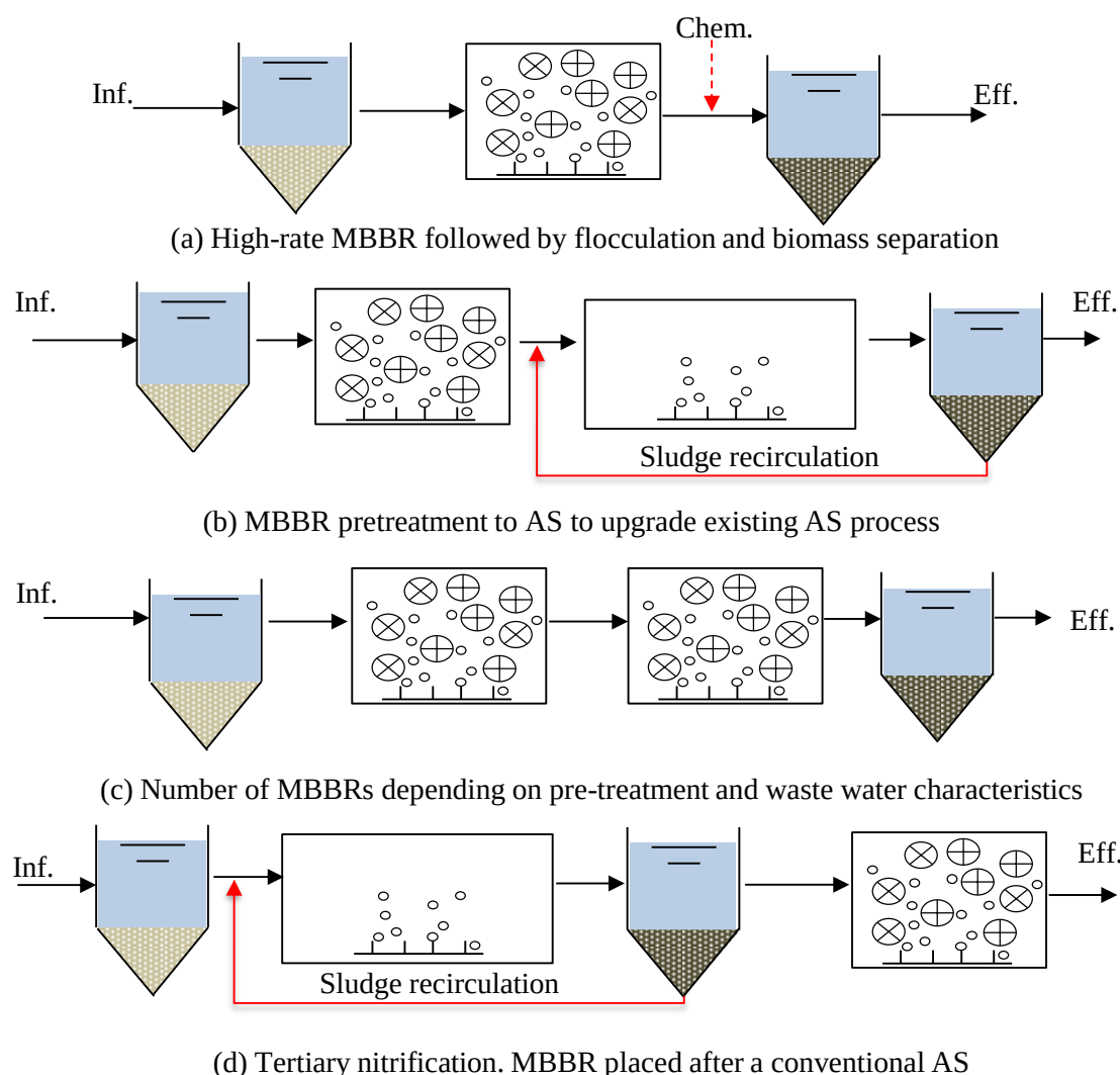
Figure 3.1: Typical process flow sheet for COD removal, nitrification and a combined C/N removal MBBR system (adapted from McQuarrie and Boltz, 2011).
