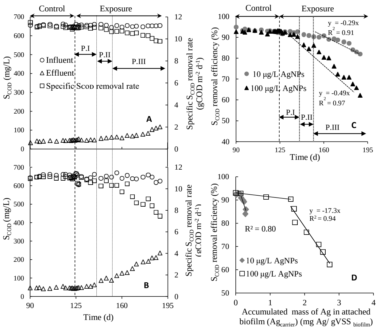
Figure 5.2 : Effect of PVP-AgNPs addition on MBBR performance at (A) 10 \mu g/L AgNPs (B) 100 \mu g/L AgNPs, (C) S_{COD} removal efficiency and (D) correlation between Ag_{carrier} and S_{COD} removal efficiency (error bars are only shown when larger than symbol size). Note: P.I-III refers to three observed phases in Ag distribution profile.
