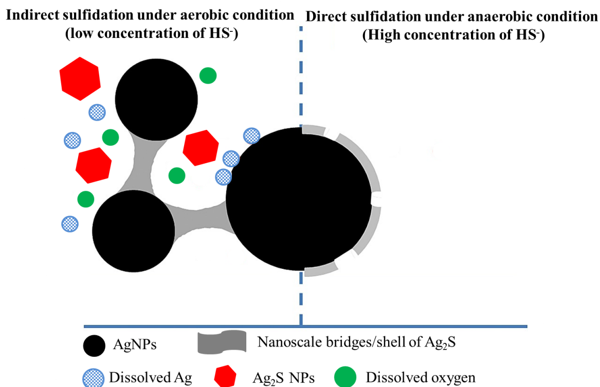
Figure 2.4 : Proposed sulfidation mechanisms of AgNPs (adapted from Zhang et al., (2018a).
