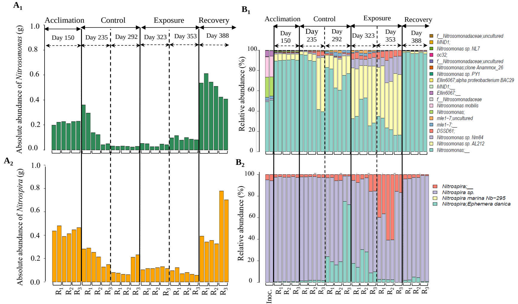
Figure 6.6: Absolute abundance of dominant (A 1 ) AOB and (A 2 ) NOB in nitrifying MBBR 1 (R 1 ), MBBR 2 (R 2 ) and MBBR 3 (R 3 ) at different stages of operation (Acclimation, Control, Exposure, Recovery), relative abundance of dominant species, affiliated to (B 1 ) Nitrosomonas and (B 2 ) Nitrospira genera. (Note: The absolute abundance of AOB and NOB are calculated using the DNA yield and biomass concentrations in MBBR at each sampling point.).
