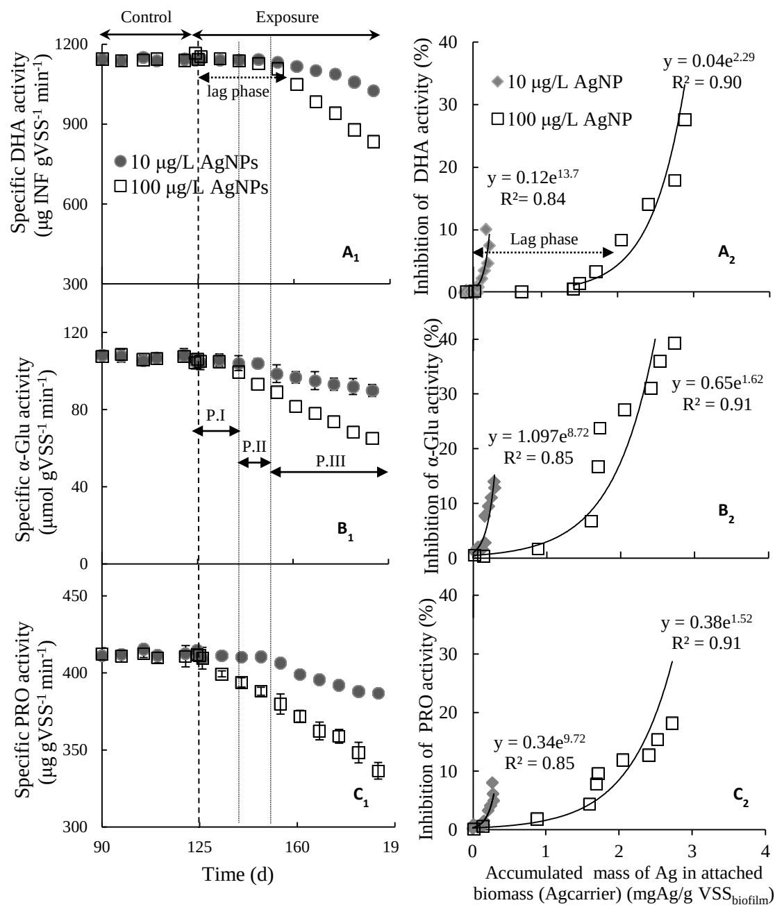
Figure 5.4: Effect of continuous PVP-AgNP injection on specific activity of (A 1 ) DHA (B 1 ) α-Glu and (C 1 ) PRO, (A 2 -C 2 ) correlation between Ag carrier and enzyme activity inhibition (Error bars are only shown when larger than symbol size).
