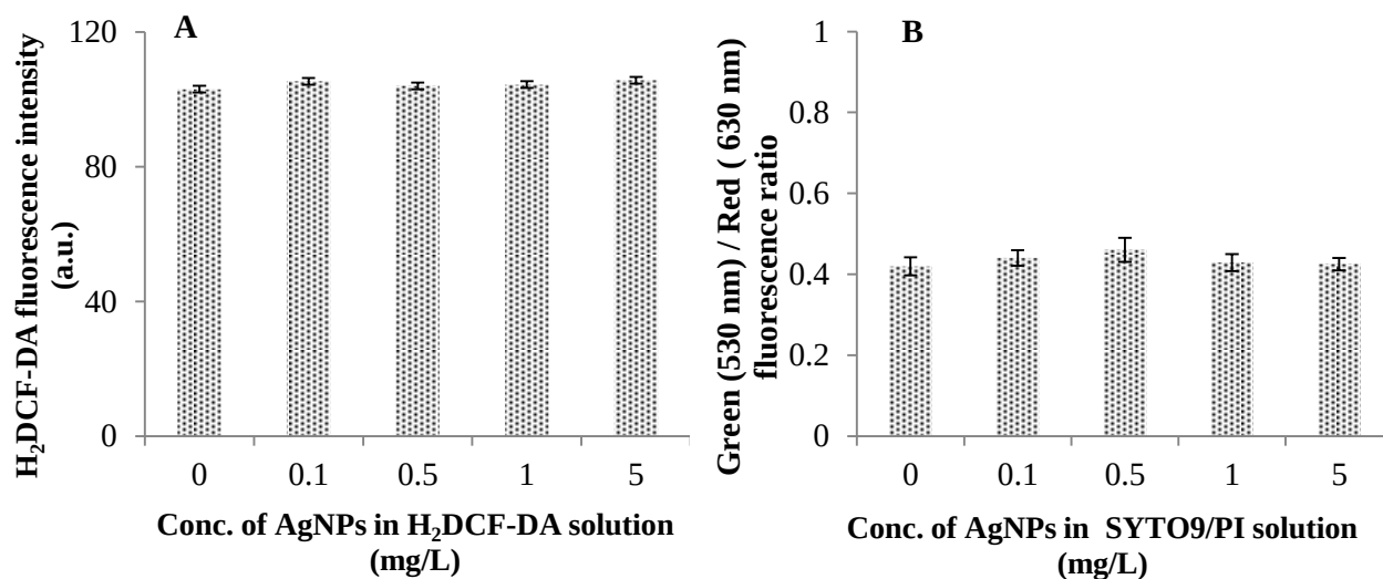
Figure B.3 : Quenching effect of AgNPs on fluorescence intensity of (A) H 2 DCF-DA solution in ROS assay and (B) SYO9/PI solution in Baclight viability assay.
