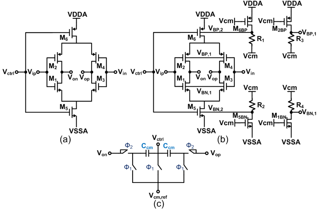
Figure 3.13 Inverter-based OTA, (a) Proposed SB inverter-based OTA in the weak inversion, (b) Proposed SBB inverter-based OTA in the weak inversion, (c) CMFB circuit.
