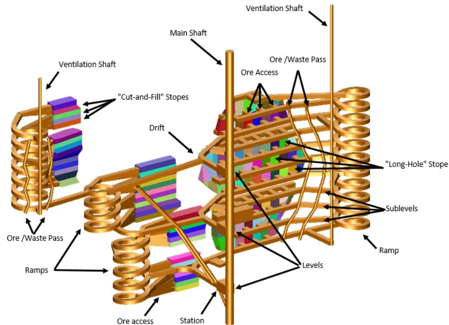
Figure 4.1 Mine Layout
