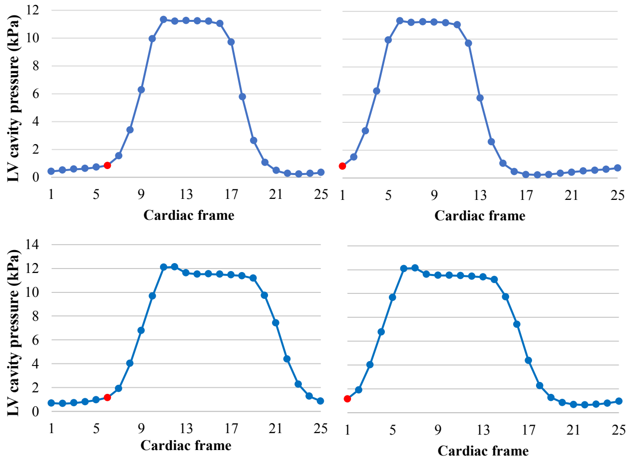
Figure 3.6. The evolution of the intra-ventricular pressure simulated at rest ( top ) and peak exercise ( bottom ) as a function of time for a typical case, before ( left ) and after the temporal synchronization ( right ). The red dot identifies the end-diastolic frame, which is the beginning of the cardiac cycle in the segmentation software CIM.
