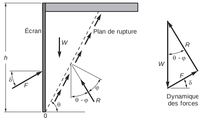
Figure 2-14 : Coin de Coulomb (Massicotte, 2019)
