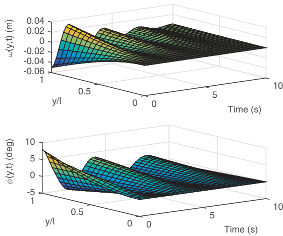
Fig. 1. Open-loop response.
