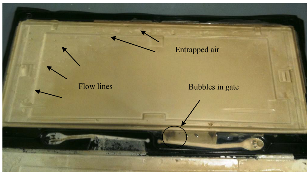
Figure 5-2 : Resin injection at a flow rate of 2000 g/s.
