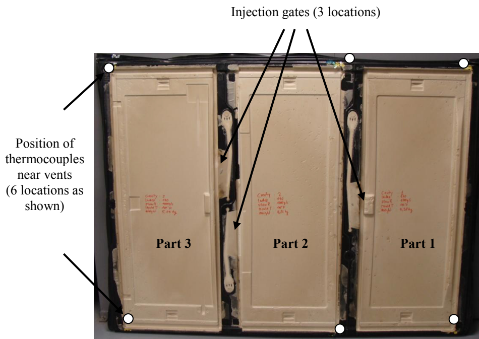
Figure 5-12 : Example of a 3D foam panel without its thermoplastic skin.
