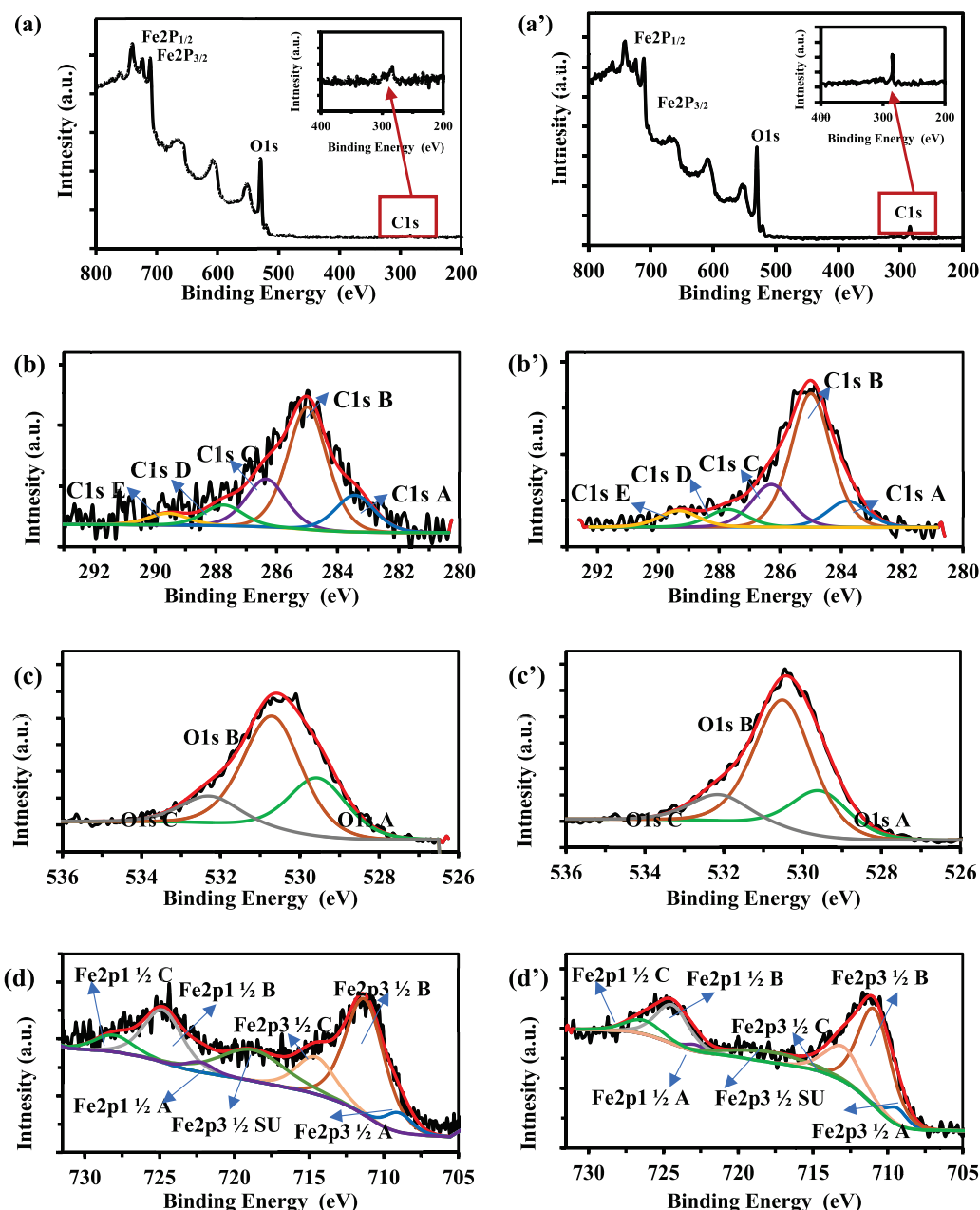
Figure 4. XPS Surveys spectra (a) bare MIONPs, (a') treated MIONPs; deconvolutions of high-resolution spectra of C1s for (b) bare MIONPs, (b') treated MIONPs; High resolution oxygen peak deconvolution for (c) bare MIONPs and (c') treated MIONPs; High resolution iron peak deconvolution for (d) bare MIONPs and (d') treated MIONPs.
