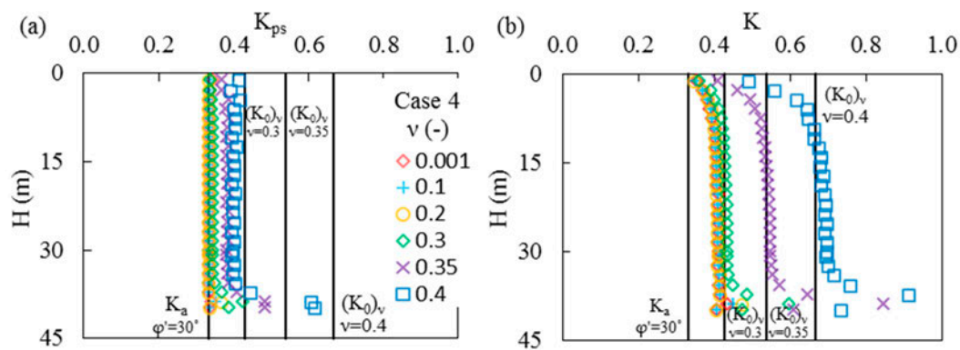
Figure 7. Vertical profiles of (a) K_{ps} and (b) K near the RW for different values of \nu , independent from the \phi' value (Case 4 in Table 1).
