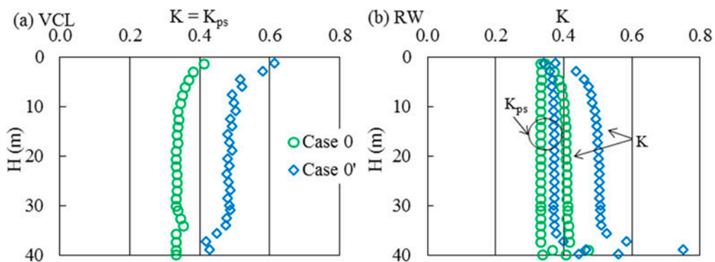
Figure 4. Vertical profiles of the earth pressure coefficient K and the principle stress ratio K_{ps} (a) along the VCL and (b) near the RW, for independent (Case 0) and related (Case 0') values of \nu and \phi' (see Table 1 for details).
