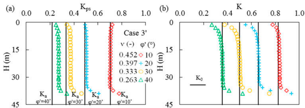
Figure 9. Vertical profiles of (a) K_{ps} and (b) K near the RW for different \varphi' values related to \nu values (Case 3' in Table 1).
