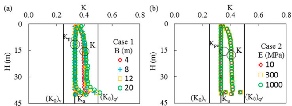
Figure 5. Vertical profiles of K_{ps} and K near the RW for different values of (a) B (Case 1 in Table 1) and (b) E (Case 2 in Table 1) for independent values of \nu and \varphi' .
