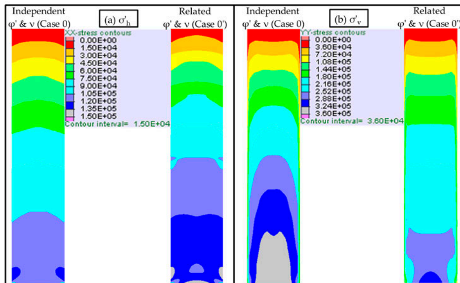
Figure 2. Horizontal (a) and vertical (b) stress (in Pa) contours from FLAC simulations conducted for independent (Case 0) and interrelated (Case 0') values of \nu and \phi' (see Table 1 for details).
