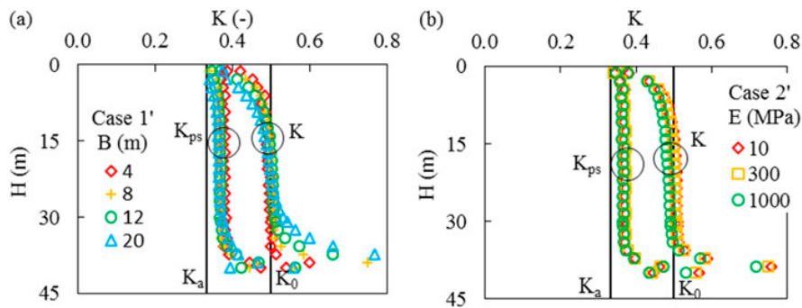
Figure 8. Vertical profiles of K_{ps} and K near the RW for different values of (a) B (Case 1' in Table 1) and (b) E (Case 2' in Table 1) for linked \nu and \varphi' values.
