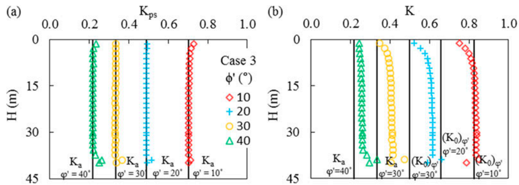
Figure 6. Vertical profiles of (a) K_{ps} and (b) K near the RW for different values of \phi' with a constant \nu value (Case 3 in Table 1).
