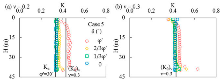
Figure 12. Vertical profiles of K (= \sigma'_h / \sigma'_v) near the RW as a function of the angle \delta' for \nu = (a) 0.2 and (b) 0.3, obtained with a constant value of \varphi' = 30^\circ (Case 5 in Table 1).
