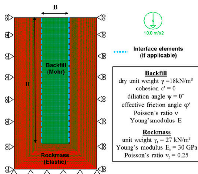
Figure 1. Numerical model of a backfilled opening built with a finite difference code FLAC.
