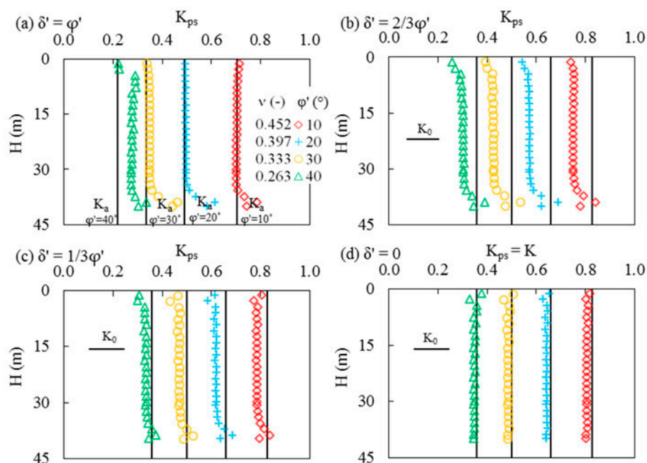
Figure 13. Vertical profiles of K_{ps} (= \sigma'_3 / \sigma'_1) near the RW as a function of \nu for the angles \delta' = \varphi' (a), 2/3\varphi' (b), 1/3\varphi' (c) and 0 (d), obtained with related values of \nu and \varphi' (Case 4' in Table 1).
