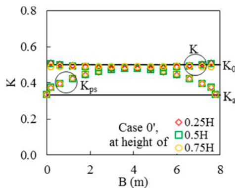
Figure 10. Distributions of K_{ps} and K across the opening width ( B ) at different heights for related values of \nu and \varphi' (Case 0' in Table 1).
