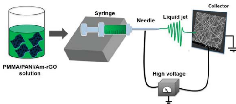
Figure 1. Schematic illustration of the electrospinning setup.
