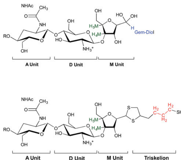
Fig. 4 Structure of unmodified CS (top) and CS- b -triskelion adduct (bottom). The protons corresponding to the ^1\text{H} NMR peaks used for the calculations of the functionalization degree in eqn (1) and (2) are shown in green, blue and red.
