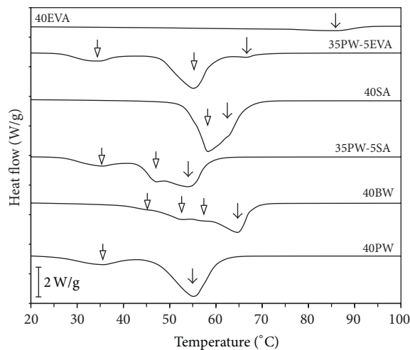
FIGURE 2: DSC thermogram of binders.
