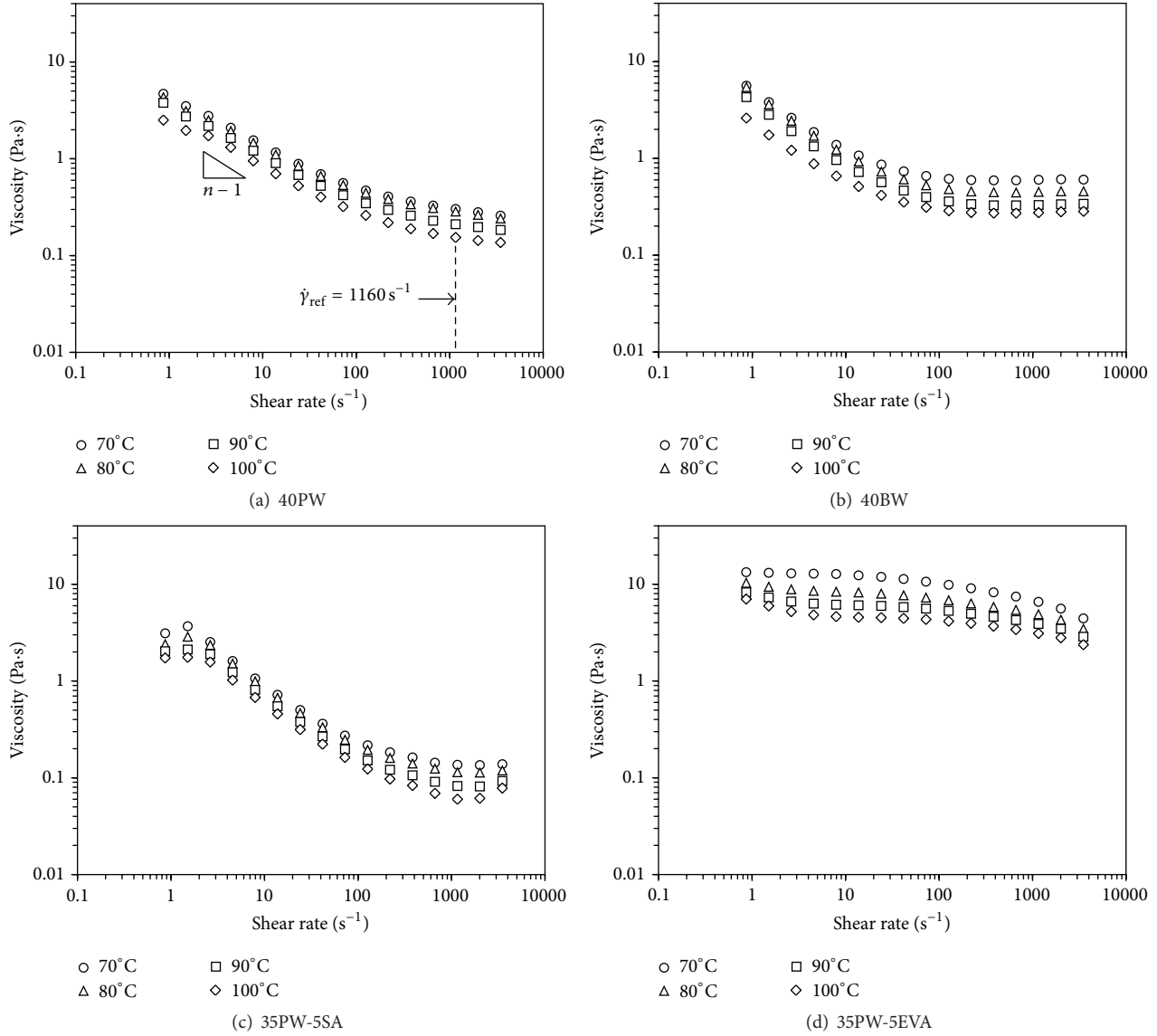
FIGURE 4: Viscosity profiles of feedstocks at different temperatures.
