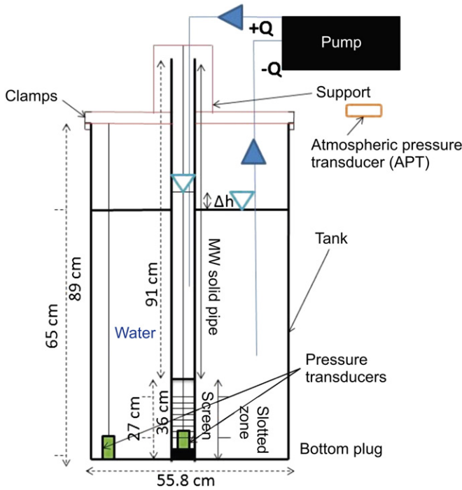
Fig. 2. Sketch of the experimental set-up to determine K_1 .
