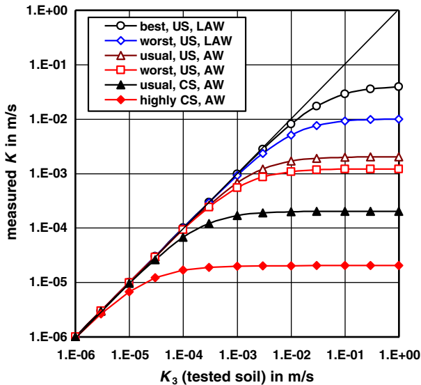
Fig. 4. Influence of screen ( K_1 ) on the K_{\text{test}} value when there is no filter pack: analytical results (Eq. (5)) and numerical results are similar; worst for K_1 = 6 \times 10^{-5} m/s; usual for K_1 = 10^{-4} m/s; best for K_1 = 2 \times 10^{-3} m/s; US = unclogged screen; CS = clogged screen; AW = aerated water; LAW = less aerated water.
