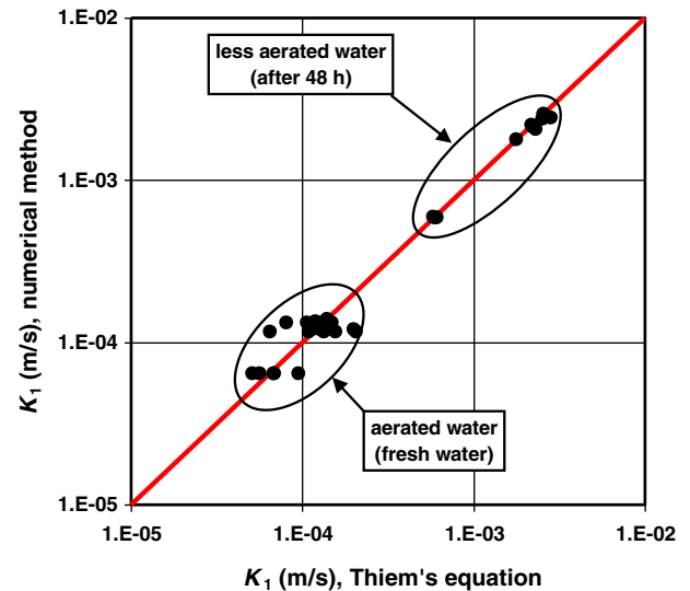
Fig. 3. Correlation between K_1 values obtained either numerically or using Eq. (1) for unclogged screens in a water tank.
