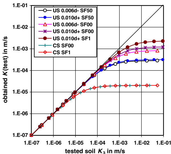
Fig. 5. Influence of K_1 (screen) and K_2 (filter sand) on K_{\text{test}} for constant-head tests with fully penetrating screens. US = unclogged screen, CS = clogged screen with K_1 = 10^{-5} m/s; 0.006d – is the type of screen; SF50 the type of filter sand.
