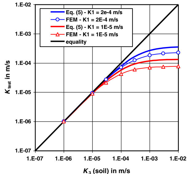
Fig. 6. Influence of K_1 (screen) and K_2 (filter sand) on K_{\text{test}} for variable-head (slug) tests and one case of partially penetrating screen (FEM = finite element method).
