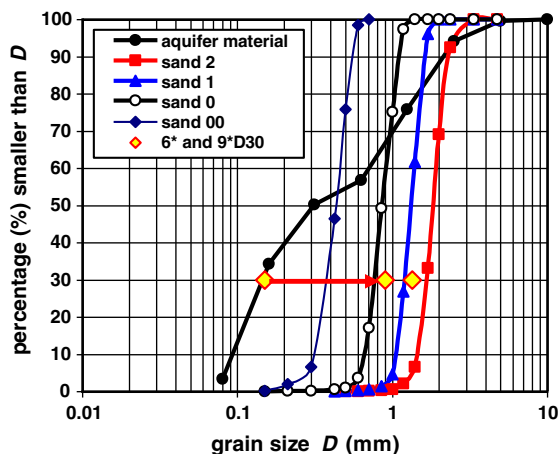
Fig. 7. Selection of the filter sand according to the criteria of Table 2. If the aquifer material is homogeneous, the filter sand 1 is appropriate. However, if the aquifer material is stratified, bimodal, the filter sand 0 must be selected, otherwise the MW screen will be severely clogged and the sampled groundwater will be turbid.
