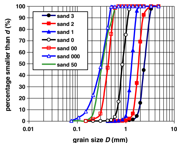
Fig. 1. Examples of grain size distribution curves (GSDCs) for commercial filter sands.
