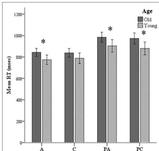
FIGURE 4 | Mean reaction times (RTs) shown here over all lexical-semantic conditions of the task: A, abstract; C, concrete; PA, pseudo-abstract (pseudo-words derived from abstract stimuli); and PC, pseudo-concrete (pseudo-words derived from concrete stimuli). * p < 0.05 .
