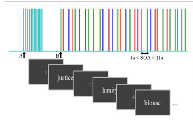
FIGURE 1 | A schema of the task diagram with inter stimulus interval = 1.36 s and stimulus onset asynchrony from 4 to 11 s. Triggers from the computer presenting the task were sent to the NIRS computer after synchronization: A, start control task and B, start main task. Each color bar represents a different condition: concrete, abstract, and pseudo-words.
