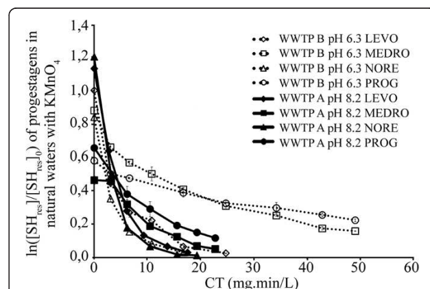
Figure 3 Steroid hormone (SH) decay curves following oxidation with permanganate in wastewaters (WWTP A, pH 8.2 and WWTP B, pH 6.3) for progestagens. [\text{KMnO}_4]_0 ranged from 17 to 39 \mu\text{M} . Solid (WWTP A) and dotted (WWTP B) lines represent the trend of the measured data (symbols).
