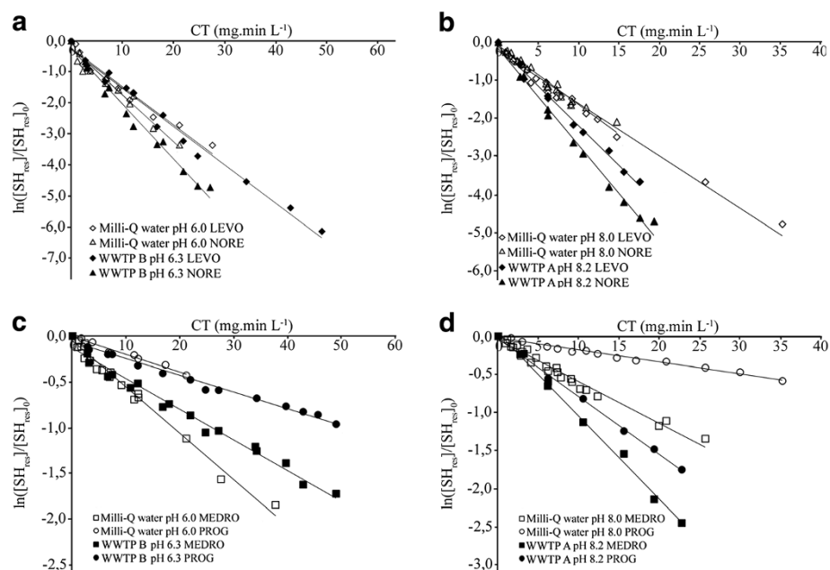
Figure 1 Second-order rate kinetic plots for the oxidation of progestagenic steroid hormones (SH) by permanganate and the resulting effect of dissolved natural organic matter (NOM) from wastewaters (WWTW A and WWTW B) for progestagens at a) and c) pH 6.0, b) and d) pH 8.0 when compared to Milli-Q water according to progestagens having similar reaction rate constants. Experimental conditions were, [KMnO_4]_0 from 17 to 39 \mu M and [progestagens]_0 from 1.9 to 3.9 \mu M . Solid lines represent the linear regression of the measured data (symbols) with their related coefficients of determination ( R^2 \geq 0.96 ).
