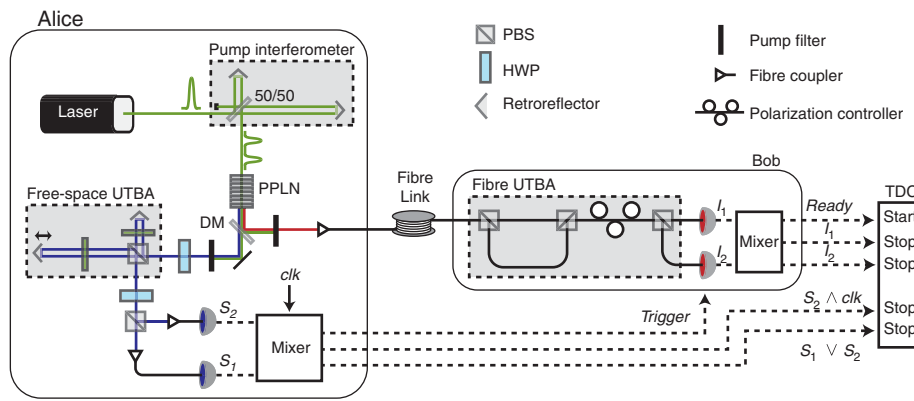
Figure 2 | Experimental set-up. A laser diode sends 50 ps pulses at 530.6 nm wavelength through an interferometer with path-length difference equivalent to 1.4-ns travel-time difference. The pulses emerge in an even superposition of two well-defined time bins that we label the early and late bins and then propagate into a nonlinear, periodically poled lithium niobate crystal (PPLN), thereby creating time-bin entangled qubits at 807 and 1,546 nm wavelengths through spontaneous parametric downconversion. The two qubits are separated at the dichroic mirror (DM). The free-space and fibre UTBAs allow Alice and Bob to measure their qubits in randomly selected bases x and y , respectively, as defined by equation (1); see Methods. The angle \varphi is selected by the orientation of the output half-wave plate (HWP) at Alice’s and the polarization controller at Bob’s. The coincidence detections are monitored using a TDC and analysed in real-time to realize all steps of the protocol. Clk; laser clock; PBS, polarization beam splitter.
