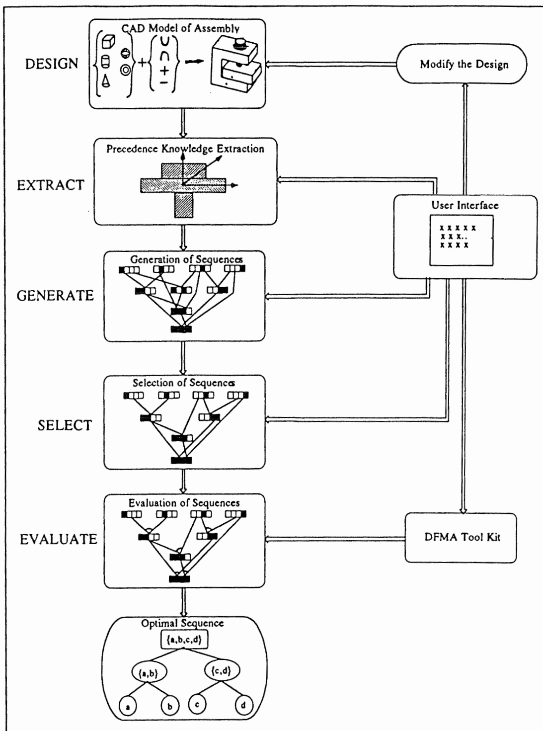
Figure 8.1. Architecture of CIAPS
