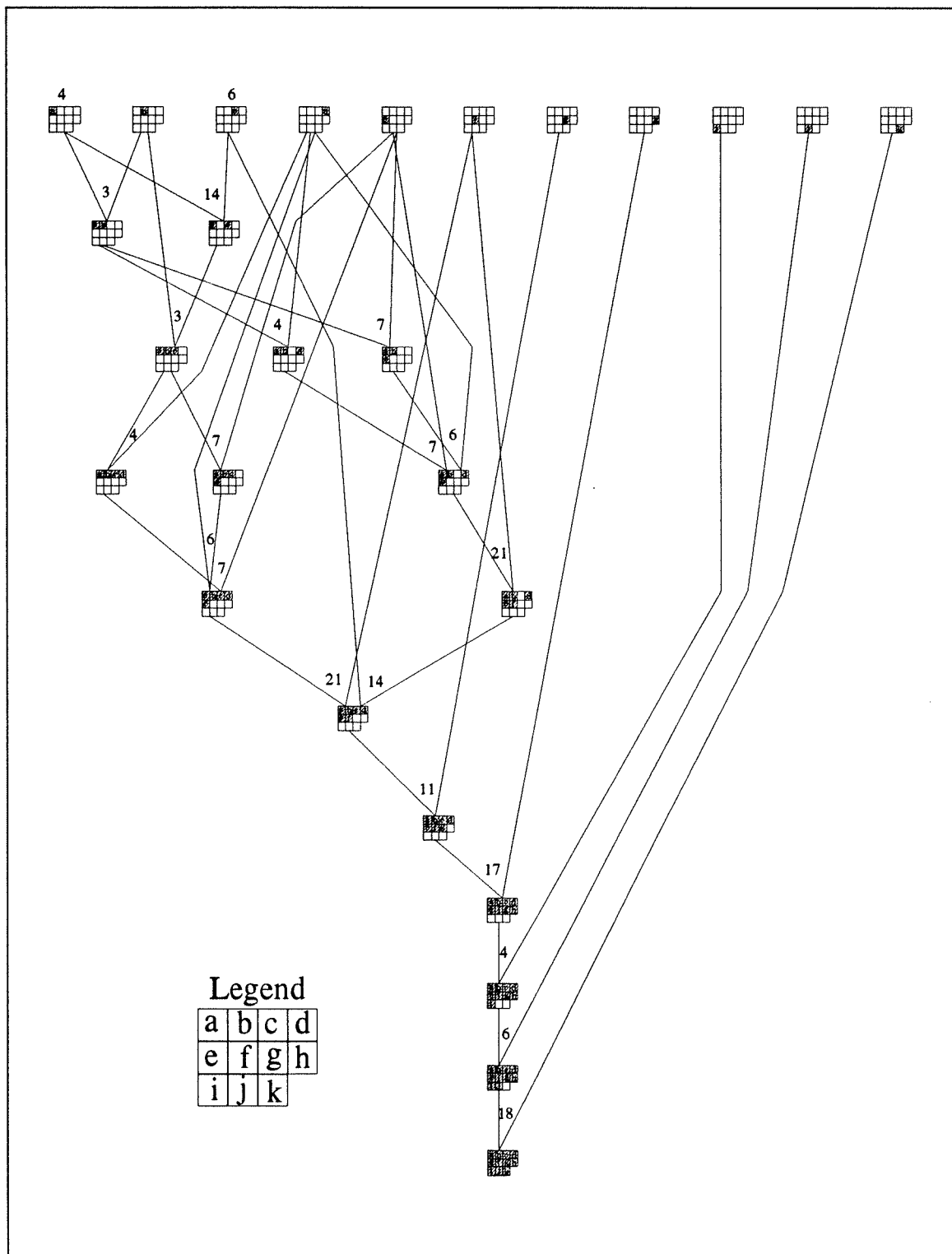
Figure 9.13. The ASG for the oven door assembly with the associated cost factors
