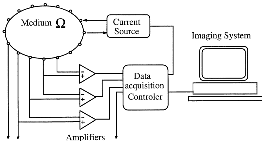
Figure 2.1: Block Diagram of a typical EIT system.
