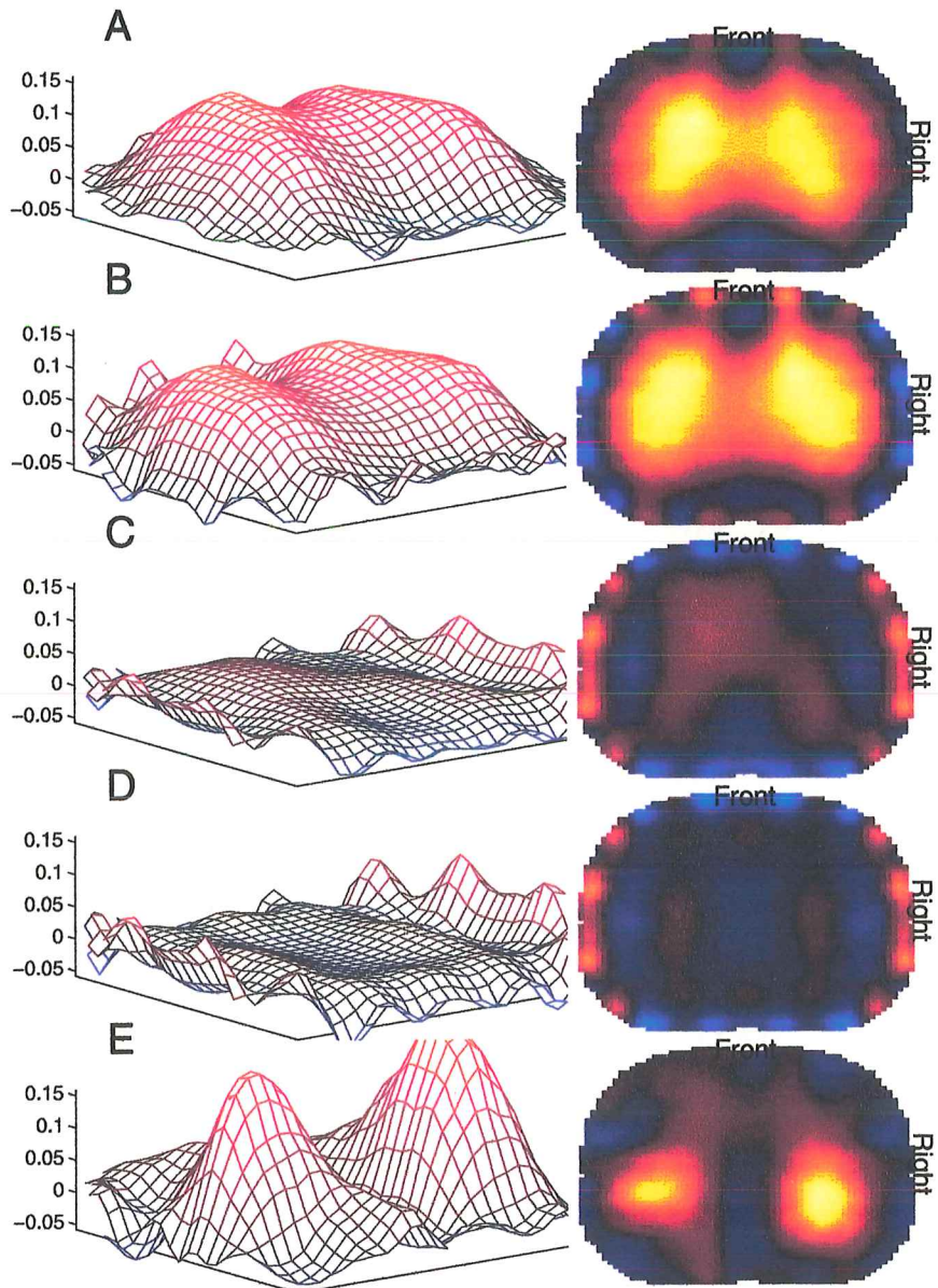
Figure 5.6: Images of conductivity change in the thorax.
