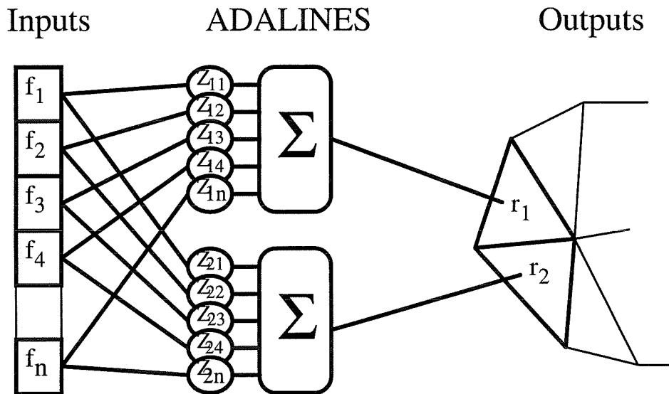
Figure 3.2: Neural Network configuration using ADALINES.
