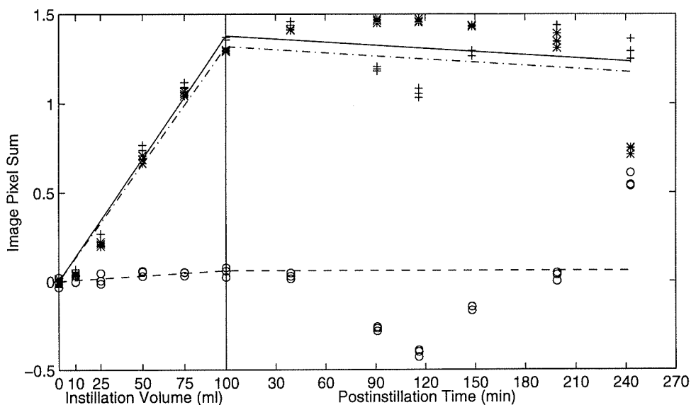
Figure 6.12: Image magnitude vs. instillation volume and reabsorption time.
