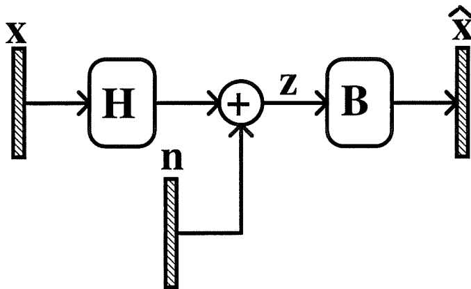
Figure 4.4: Equivalent communications systems block diagram
