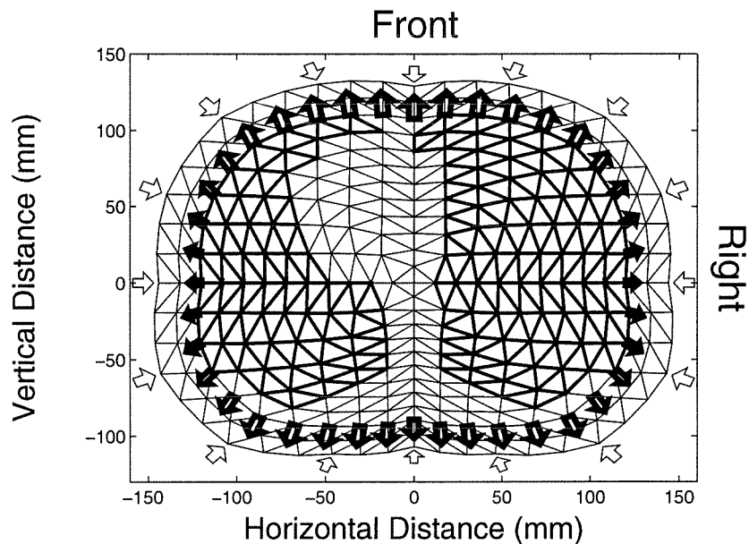
Figure 5.5: Finite element model of the electrical and mechanical properties of the thorax
