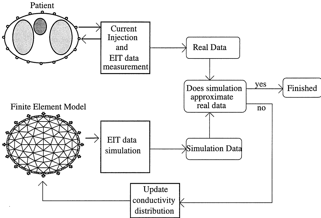
Figure 2.2: Modified Newton Raphson Algorithm
