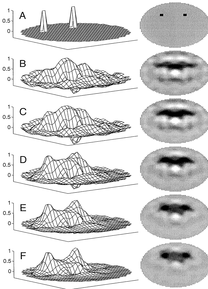
Figure 3.6: Reconstruction Errors due to elliptical deformation
