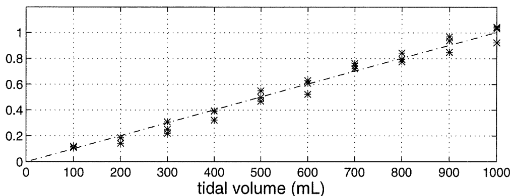
Figure 6.7: Conductivity change in the thorax from end expiration to end inspiration vs. tidal volume
