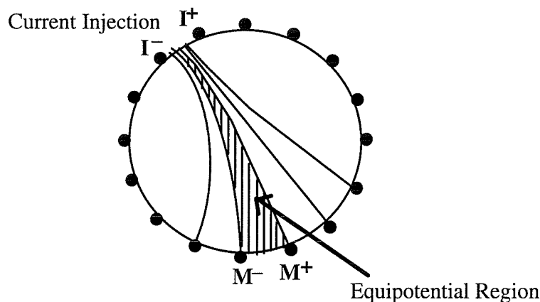
Figure 2.3: Equipotential backprojection regions for a measurement configuration.
