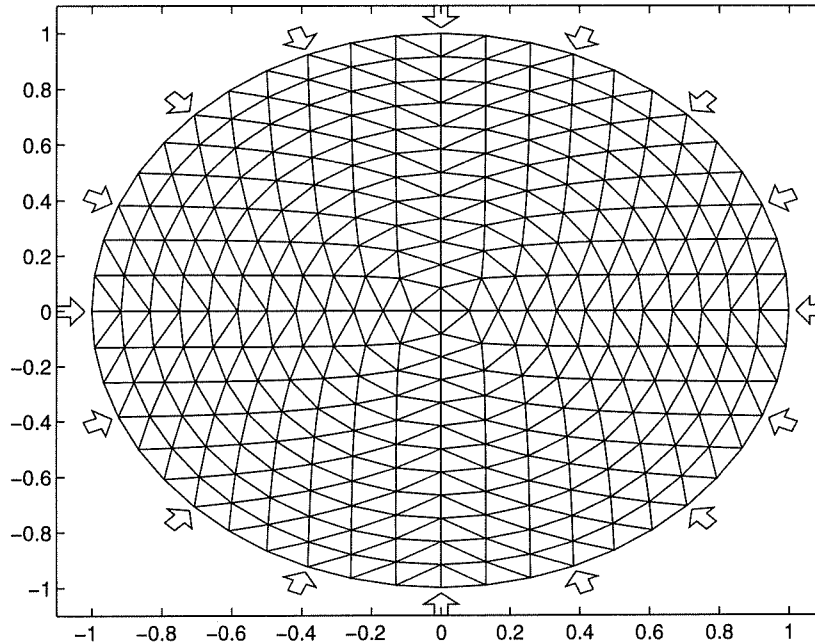
Figure 4.1: Finite Element Model used in this paper.
