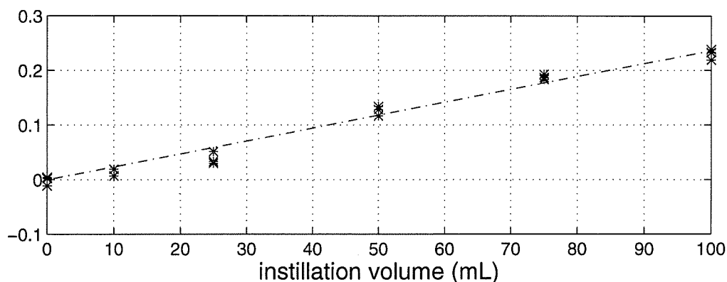
Figure 6.8: Conductivity change in the thorax vs. instilled fluid quantity
