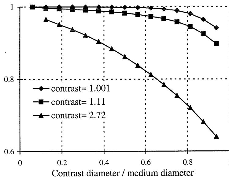
Figure 4.3: Normalised mean signal to area ratio for a circular contrast as a function of the contrast region diameter
