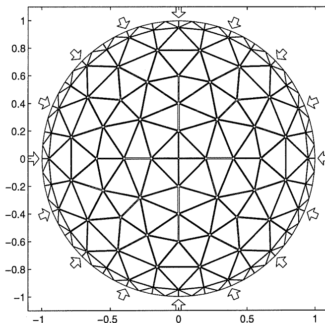
Figure 3.1: Finite element model and electrode placements.
