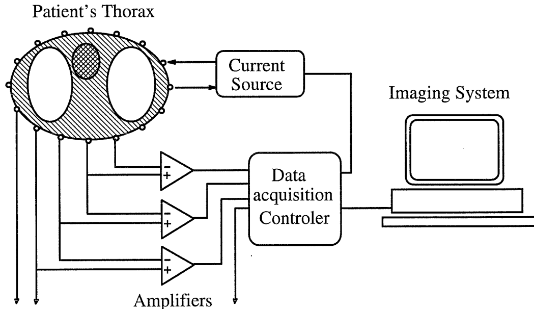
Figure 6.1: Block Diagram of our EIT system.
