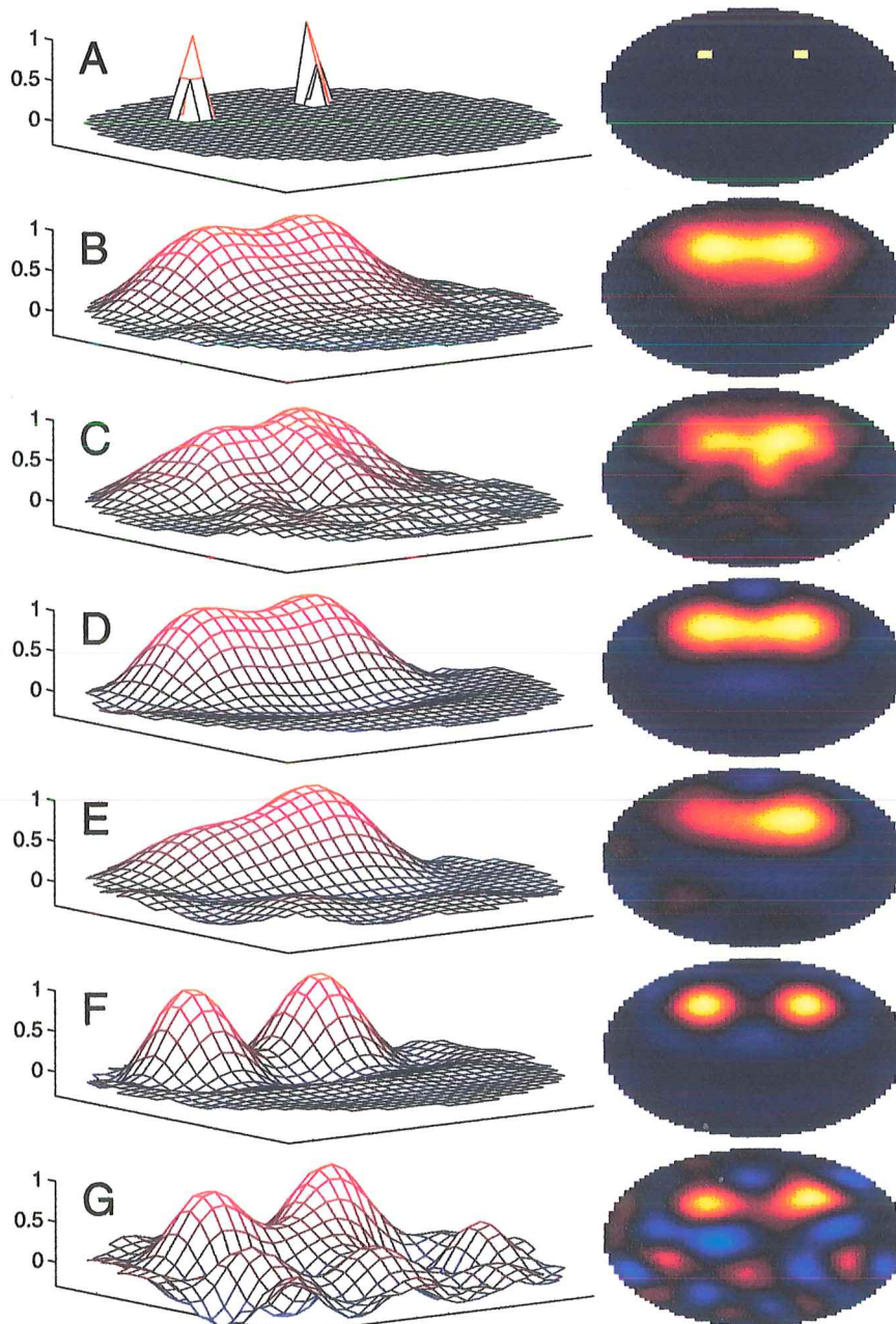
Figure 4.5: Reconstructed Images
