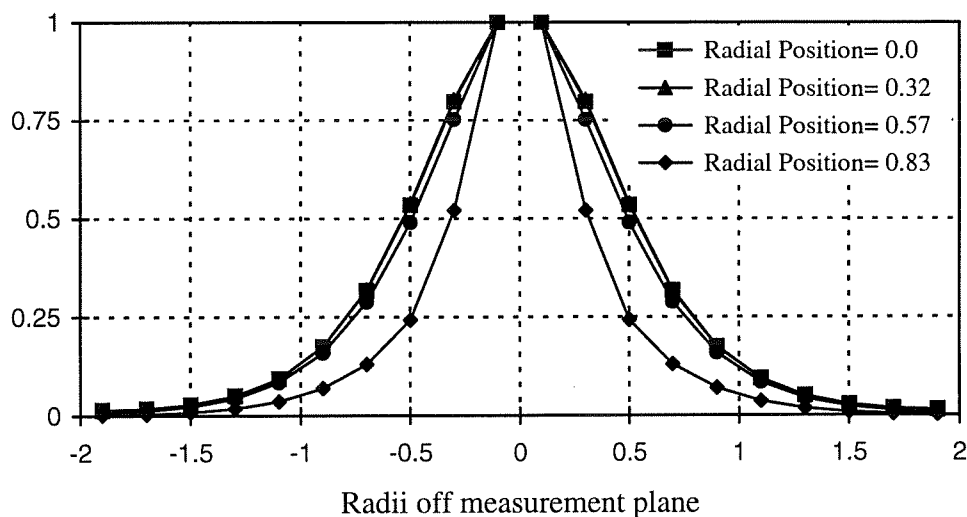
Figure 5.4: Normalised EIT sensitivity to off plane conductivity changes vs. radii of measurement plane
