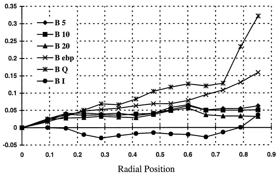
Figure 4.8: Position error vs. radial position for different algorithms
