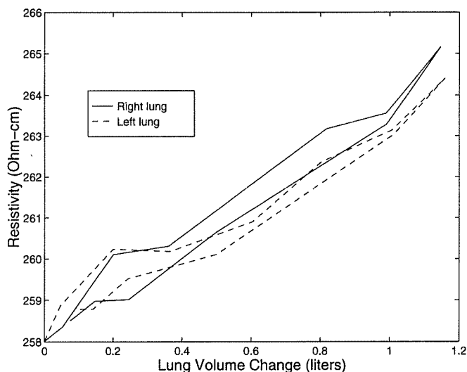
Figure 2.7: From Newell (1993): Peak resistivity in the lung field of a normal human subject increased as air was inspired.
