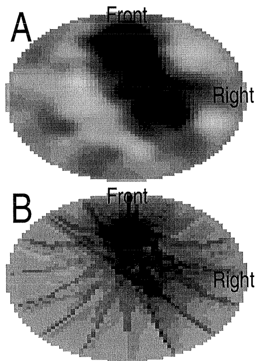
Figure 3.7: Images of two non conductive objects in saline solution A: Image using neural networks B: Image using backprojection
