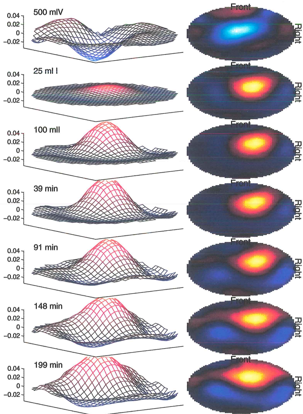
Figure 6.11: Images of conductivity change in the dog thorax for experiment #4.
