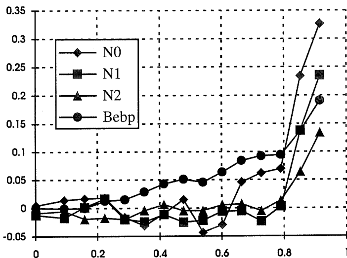
Figure A.1: Position error vs. radial position for different noise figures
