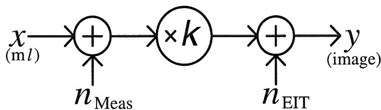
Figure 2.4: Model of EIT image formation and noise
