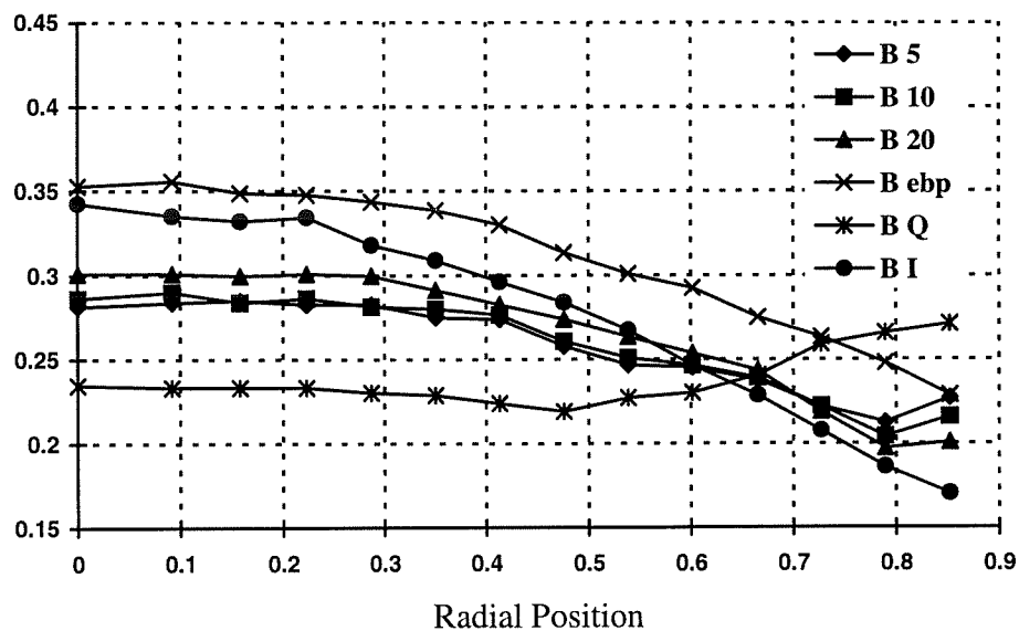
Figure 4.9: Blur radius vs. radial position for different algorithms
