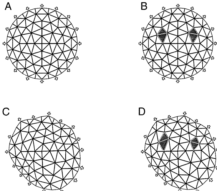
Figure 5.1: A measurement configuration with geometrical and electrode placement error
