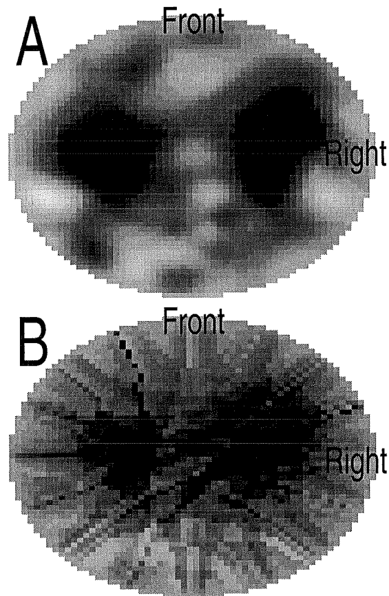
Figure 3.8: Image of conductivity changes (inspiration - expiration) in the author's thorax
