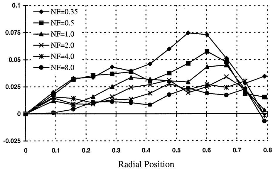
Figure 4.6: Position error vs. radial position for different noise figures
