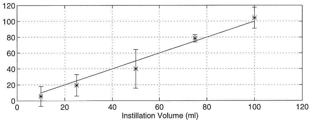
Figure 6.10: Average volume from EIT image vs. Instilled fluid Volume
