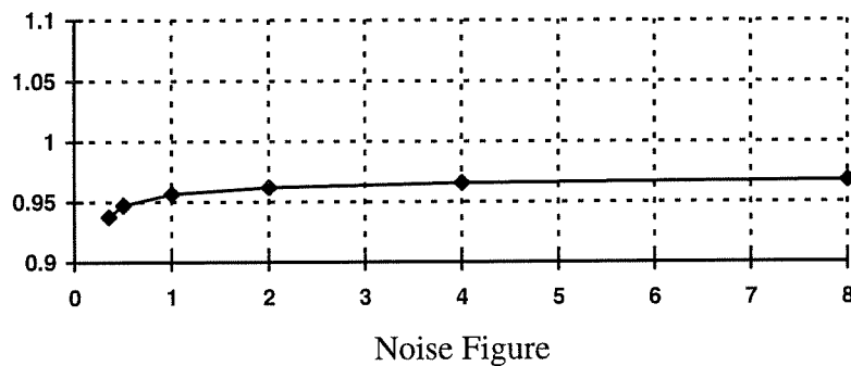
Figure 4.10: Quantitative Gain versus Noise Figure
