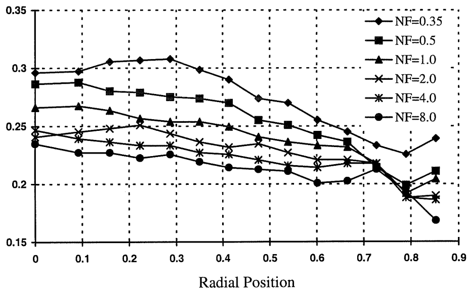
Figure 4.7: Blur radius vs. radial position for different noise figures
